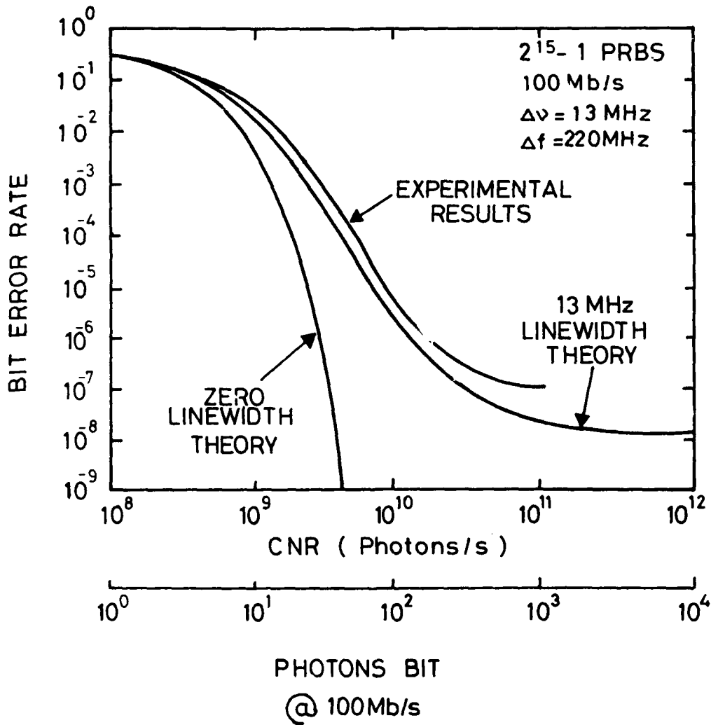
Fig.9 Performance of binary FSK
