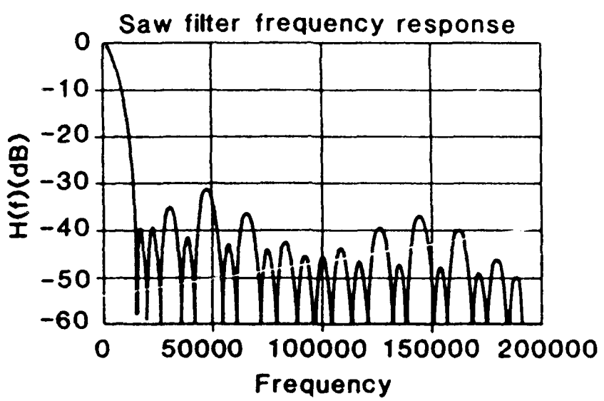
Fig.14 CFT frequency response
