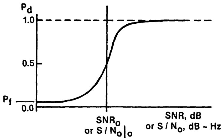
Fig.6.9 A typical "S" curve for the general detector of Fig.6.8 P_f fixed.
