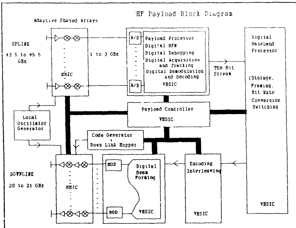
Fig 11.4 EHF payload block diagram
