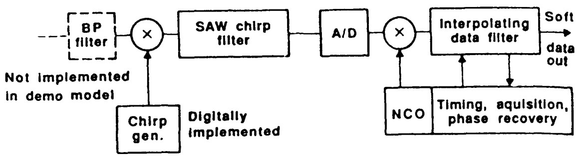
Fig.13 Block diagram of MCD demonstration model built at ELAB-RUNIT
