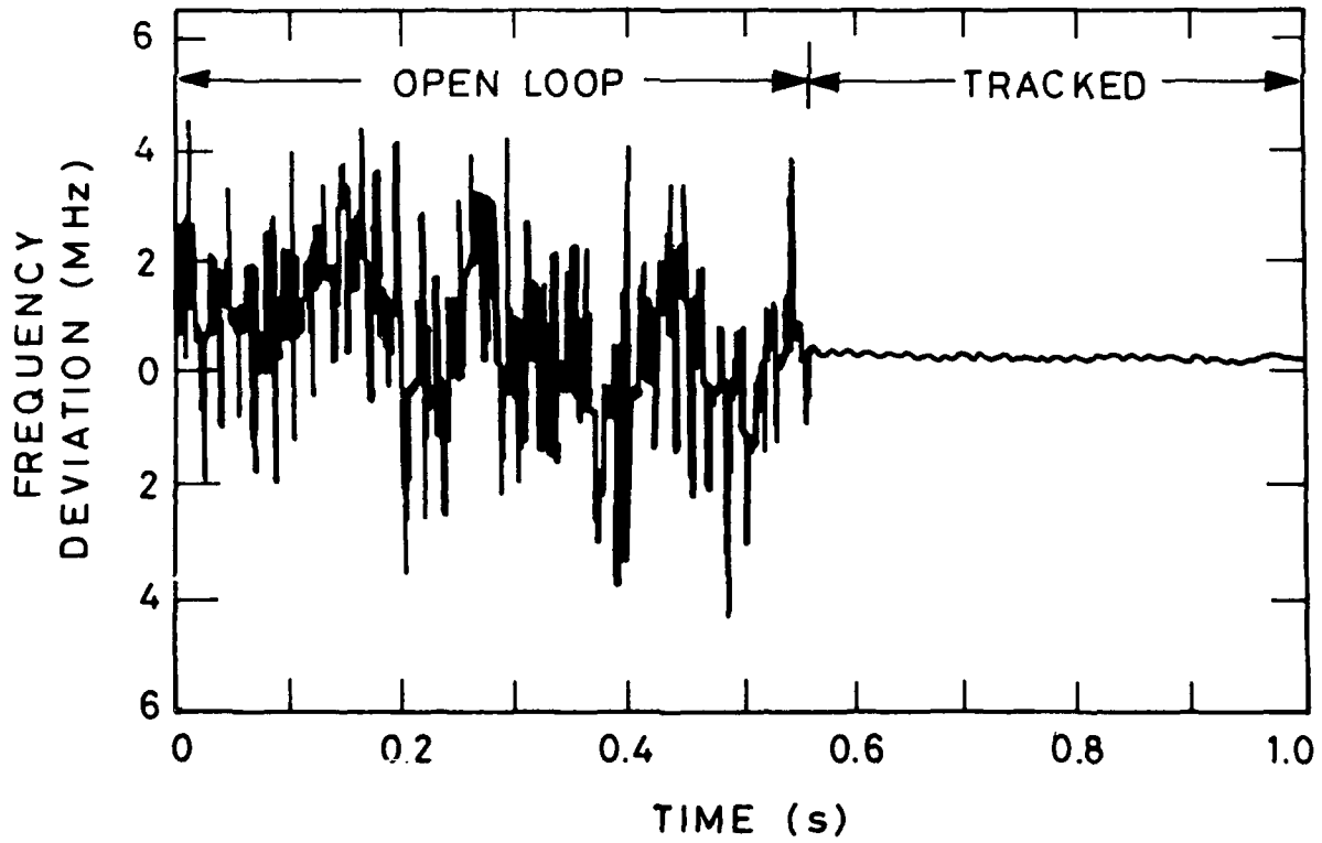
Fig.7 Frequency deviation
