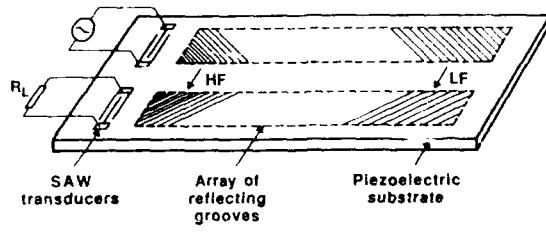
Fig.8.2.3 SAW chirp line with RAC structure [8.2.1]
