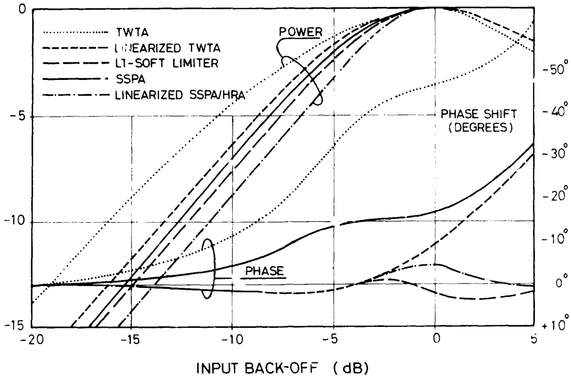
Fig 8.4.6 Transfer characteristics
