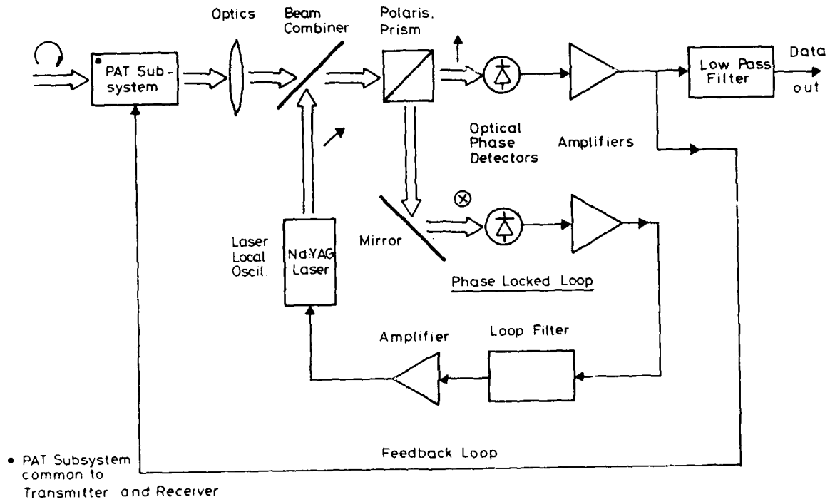
Fig.8.5.13 Nd:YAG LASER receiver assembly (ASK)
