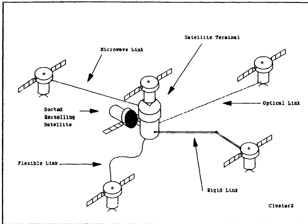
Fig.10.7 MEWS system
