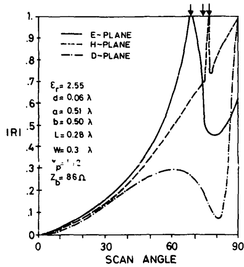
Fig. 3 Reflection coefficient for infinite array of microstrip patch radiators (after Pozar and Schaubert, IEEE Trans. AP-32, Det 1984)
