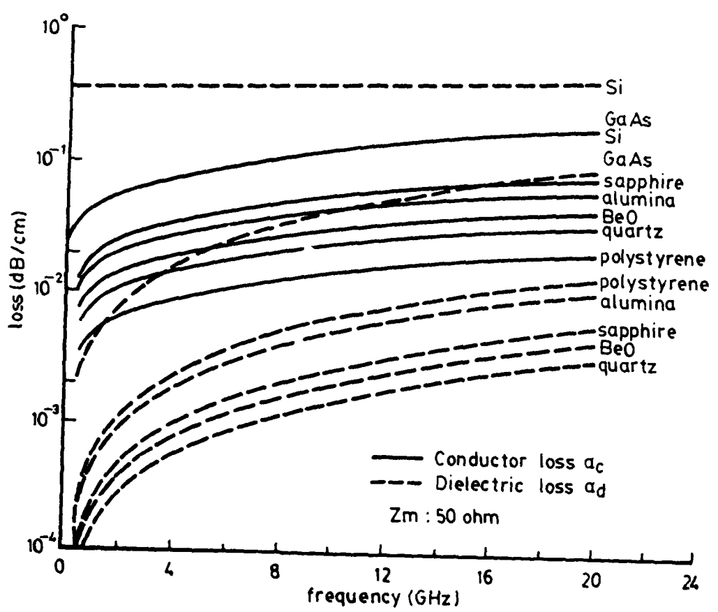
Fig.2 Conductor and dielectric losses as functions of frequency for microstrip lines on various substrates (Reproduced from Gupta et al. (1979)) h = 0.635 mm except for GaAS and Si where h = 0.254 mm
