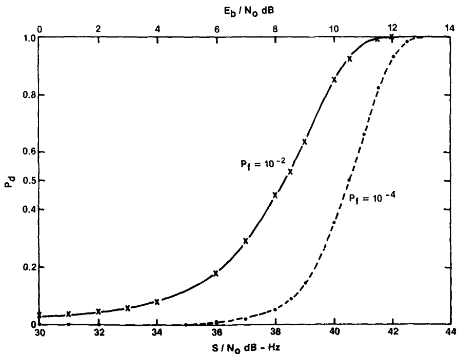
Fig.6.10 Values of P_d versus S/N_0 , E_b/N_0 for c = 1 , W = 10 MHz, T = 1 s, and 2 values of P_f .
