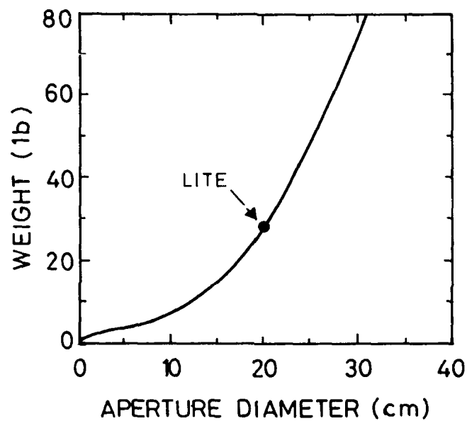
Fig.4 Telescope/gimbal weight
