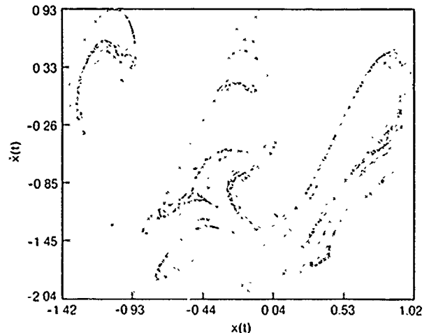
FIG. 16. Chaotic attractor corresponding to q=1.43 , k=0.3 .
