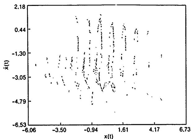
FIG. 18. Chaotic attractor for (\beta, \omega, k, q) \equiv (15, 2.25, 1.5, 21) . The system makes excursions to numerous side wells.
