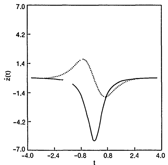
FIG. 6. Velocity profile \dot{z}(t) in the center well (solid curve) and in the side well (dotted curve). \beta=1 .
