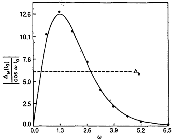
FIG. 4. Melnikov function amplitude in the side well ( z_1 z_2 ). The solid curve represents numerical calculation and data points are derived from Eq. (3.5). The dashed line represents Eq. (3.2). ( \beta, k, A \equiv (1, 1, 4) ).
