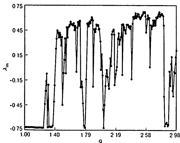
FIG. 14. Maximal Lyapunov exponent \lambda_m as a function of the driving force amplitude q . (\beta, \omega, k) \equiv (2, 2.25, 1) .
