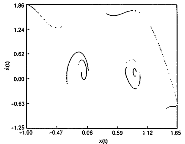
FIG. 8. Stable and unstable manifolds in parameter regime where no homoclinic behavior is expected. (\beta, \omega, k, q = A/2\pi) \equiv (2, 2.25, 1, 0.5) .
