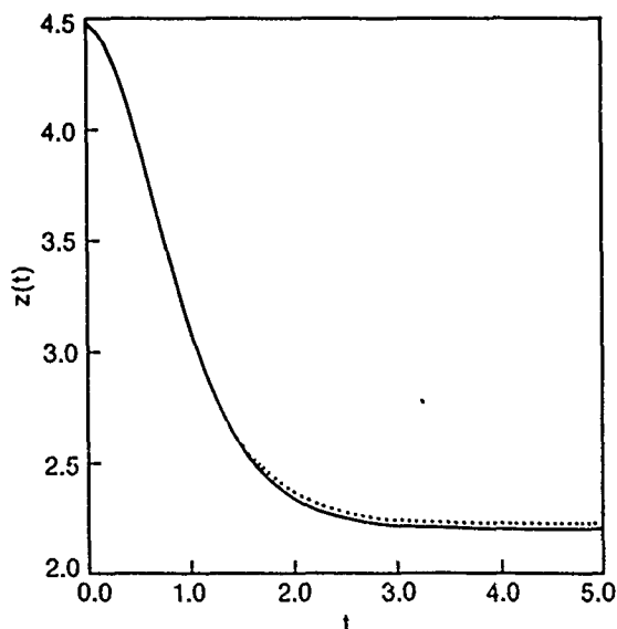
FIG. 3. Solution z(t) [Eq. (2.11)] in side well for \beta = 1 . The dotted curve represents Eq. (2.11) and the solid curve is obtained by direct (numerical) integration of (1.2).
