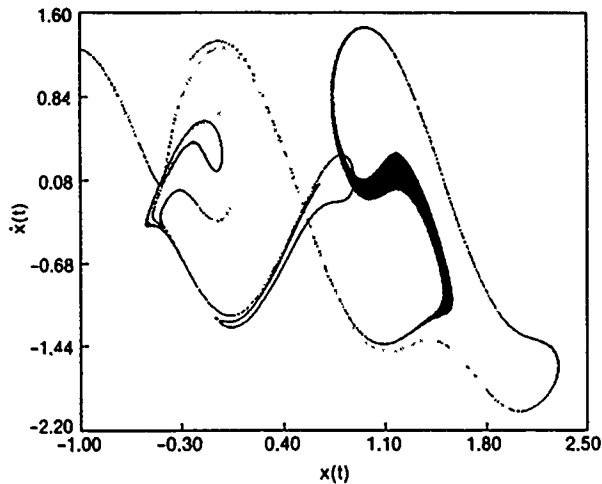
FIG. 13. Same as Fig. 12 but with q=1.25 . Supercritical case; homoclinic crossing has just occurred in center well.
