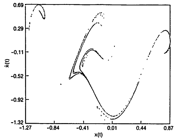
FIG. 15. Attractor corresponding to q=1.43 , k=1.0 . This case represents the possible onset of a chaotic attractor.
