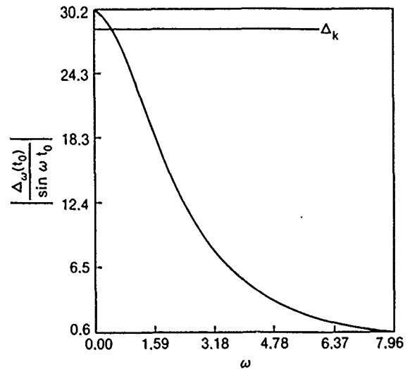
FIG. 5. Melnikov function amplitude in the center well ( z_1 z_3 ) for the same parameter values as Fig. 5. Both curves are obtained numerically.
