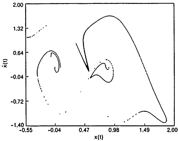
FIG. 9. Same as Fig. 8 but with q=0.72 . The stable manifold has developed a cusp and is approaching the unstable manifold in the side well.
