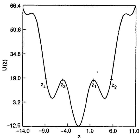
FIG. 1. Potential U(z) vs z for (\beta, \omega_0, x_0) \equiv (2, 1, 0) .
