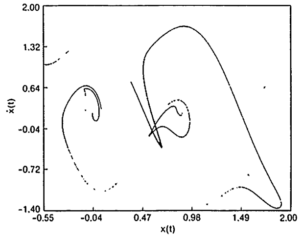
FIG. 11. Same as Fig. 10 but with q=0.75 . Supercritical case; a homoclinic crossing has taken place in the side well.
