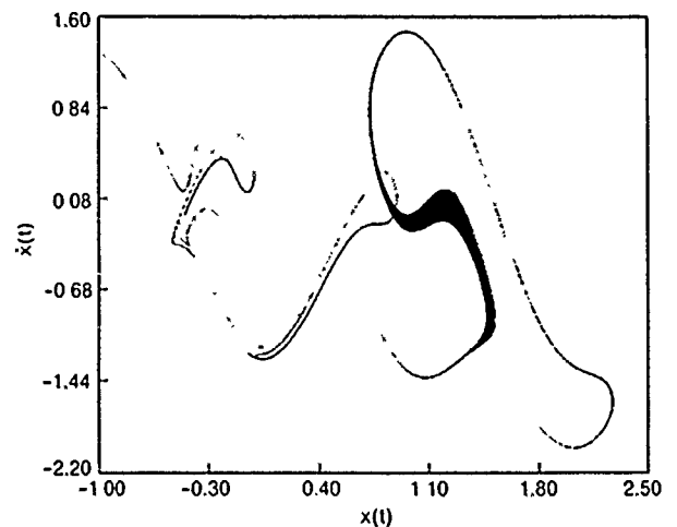
FIG. 12. Same as Fig. 11 but with q=1.21 . Near-critical case for homoclinic crossing in the center well; the manifolds are about to touch in the center well (upper left of figure). For this value of q , homoclinic crossing has already occurred in the side well. The blackened area represents the smearing of the manifold due to the numerical uncertainties referred to in the text.
