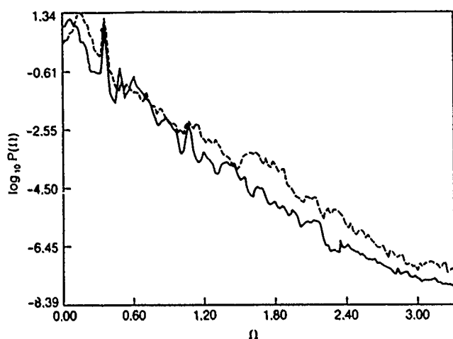
FIG. 17. Spectral densities corresponding to the attractors of Figs. 15 (solid curve) and 16 (dashed curve). Only the harmonics of the driving frequency are present, with the prominent peak on the left occurring at the fundamental driving frequency \omega/2\pi=0.36 .
