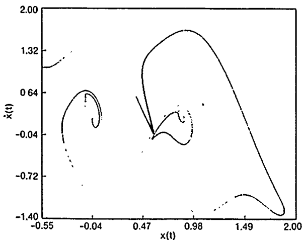
FIG. 10. Same as Fig. 9 but with q=0.73 . Critical case, the manifolds just touch in the side well.
