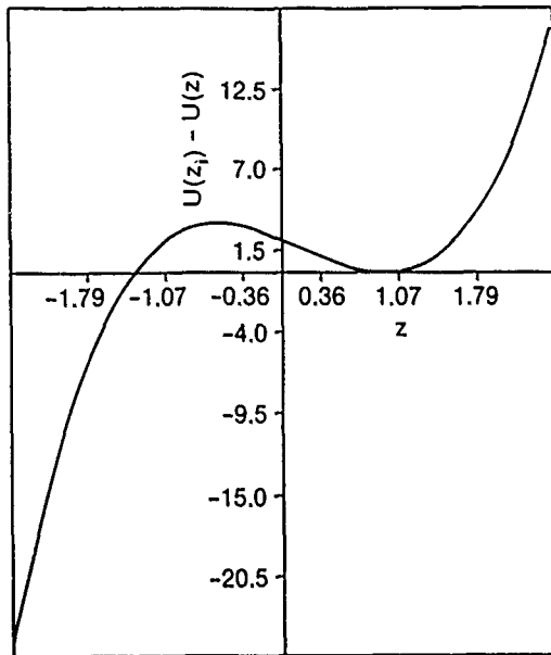
FIG. 2. Difference U(z_1) - U(z) on the separatrix. (\beta, \omega_0, x_0) \equiv (1, 1, 0) .
