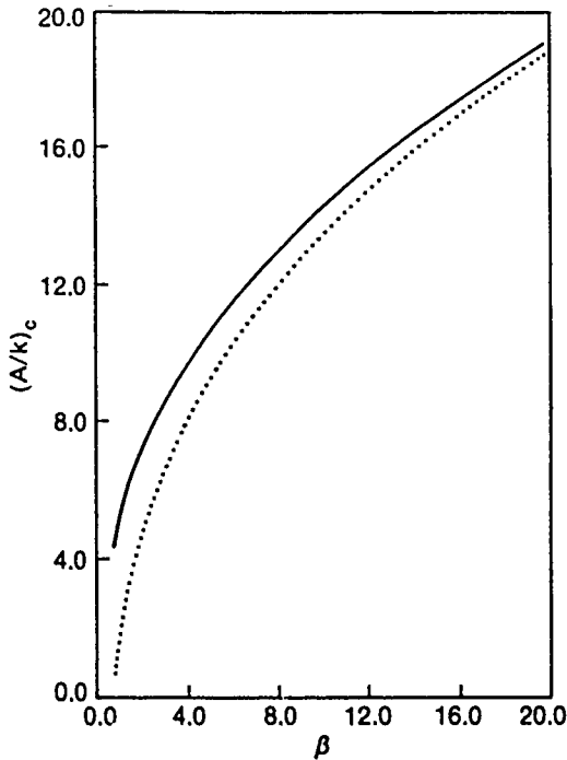
FIG. 7. Critical values of (A/k)_c as a function of \beta in center well (solid curve) and side well (dotted curve). Both curves are derived numerically at the critical frequency \omega_c corresponding to the peak of the Melnikov function amplitude in the side well.
