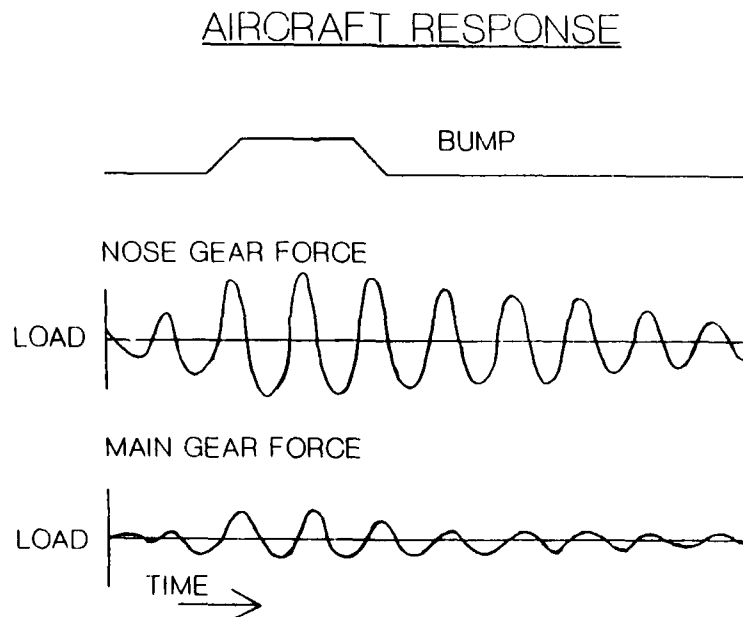
FIGURE 9. TYPICAL TIME HISTORY PLOT GENERATED BY "TAXI"
