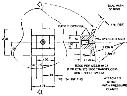
Figure 13. Example of a Rebound Chamber Pressure Tap Fitting.
