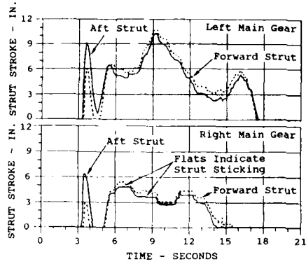
Figure 11. Example of Strut Friction during a Lateral Drift Landing.
