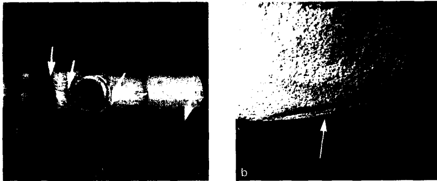
Fig. 13. a: The 0.34 m (13.4 in) long crack emanated from a fatigue crack in the trunnion radius.
