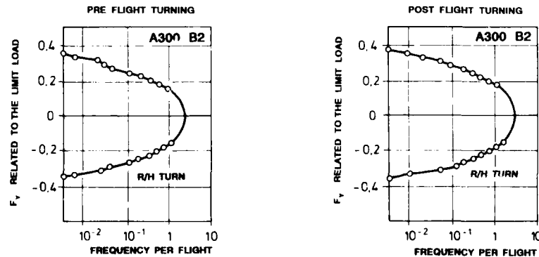
FIG.16 FREQUENCY DISTRIBUTIONS OF THE SIDE LOADS ON THE NOSE LANDING GEAR DURING TURNING [ 12 ]
