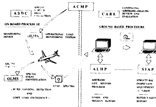
FIG.28 AIRFRAME CONDITION MONITORING PROCEDURE, ACMP
