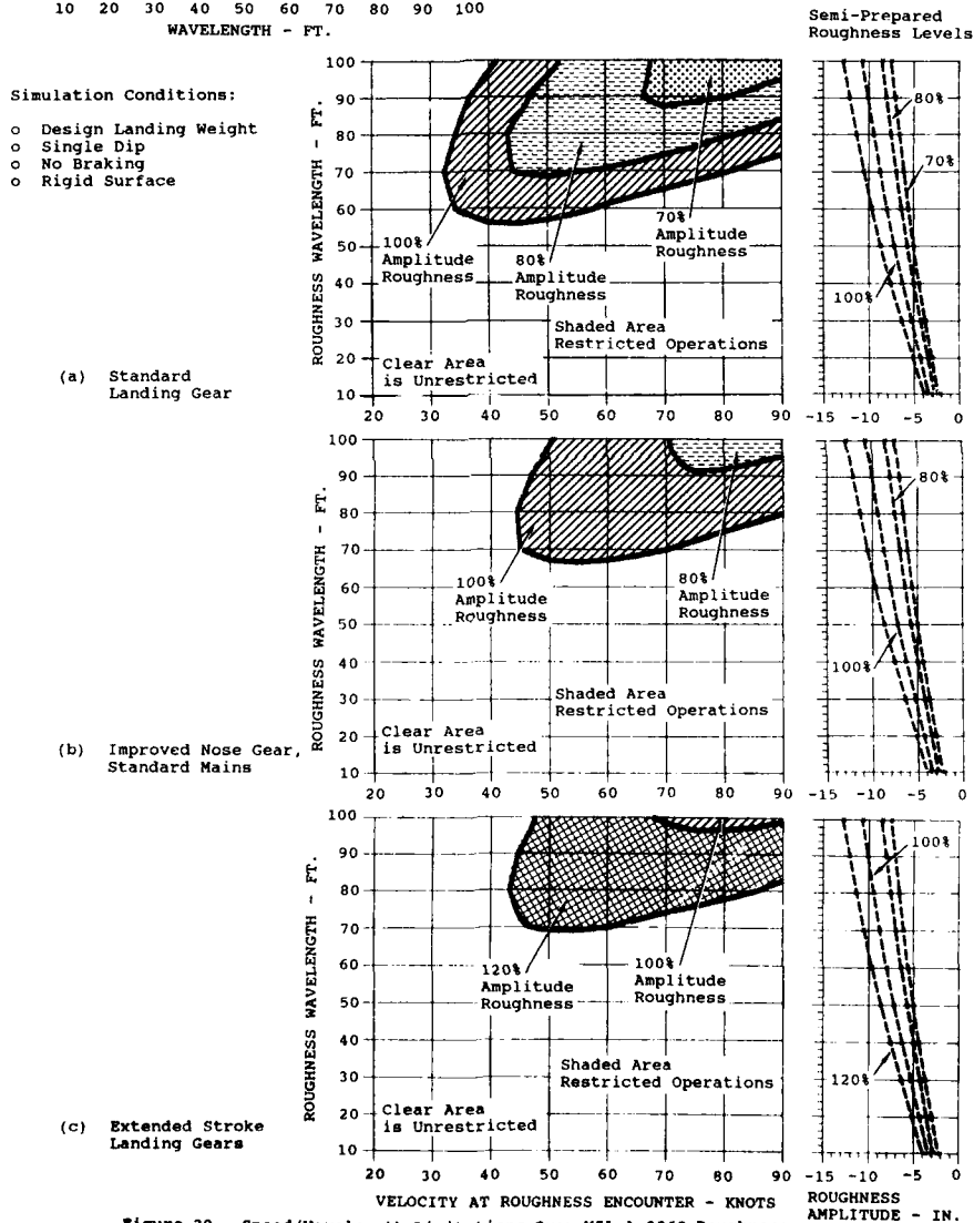
Figure 29. Speed/Wavelength Limitations Over MIL-A-8862 Roughness for Standard, Improved Nose/Standard Main, and High Sink Rate Landing Gears.
