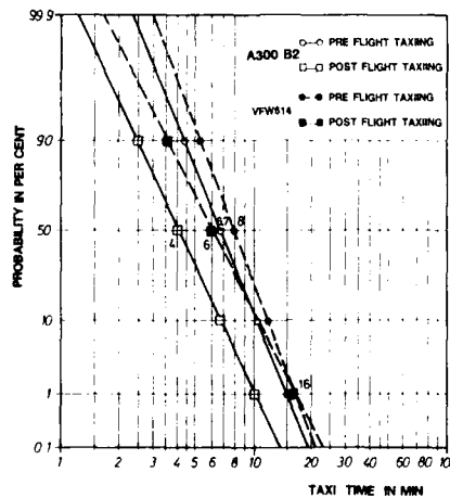
FIG.22 FREQUENCY DISTRIBUTIONS OF TAXI TIMES [ 12,16 ]
