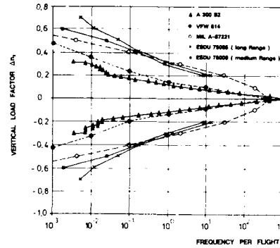
FIG.15 FREQUENCY DISTRIBUTIONS OF THE VERTICAL LOAD FACTOR DURING TAXING OF TRANSPORT AIRCRAFT [ 6, 12, 16, 29 ]
