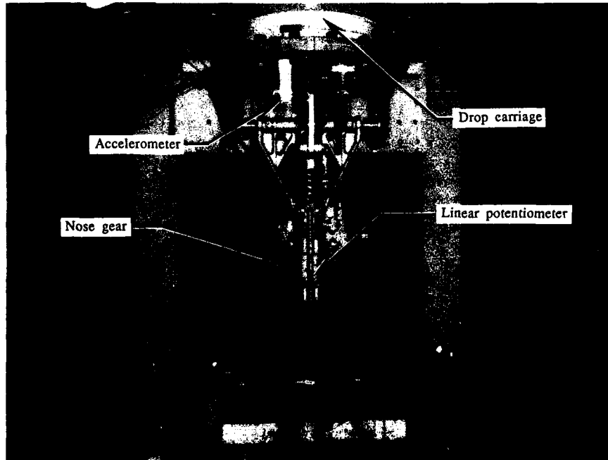
Figure 5. Nose gear mounted on drop carriage.
