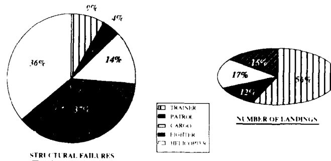
Fig. 3. Proportion of landing gear structural failures by aircraft type.
