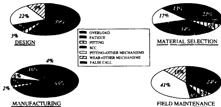
Fig. 27. Distribution of failure mechanisms by cause of failure.
