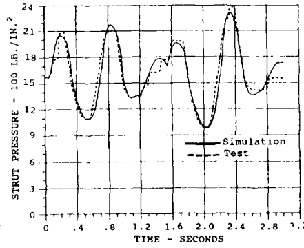
(b) Extended Stroke Main Gear
