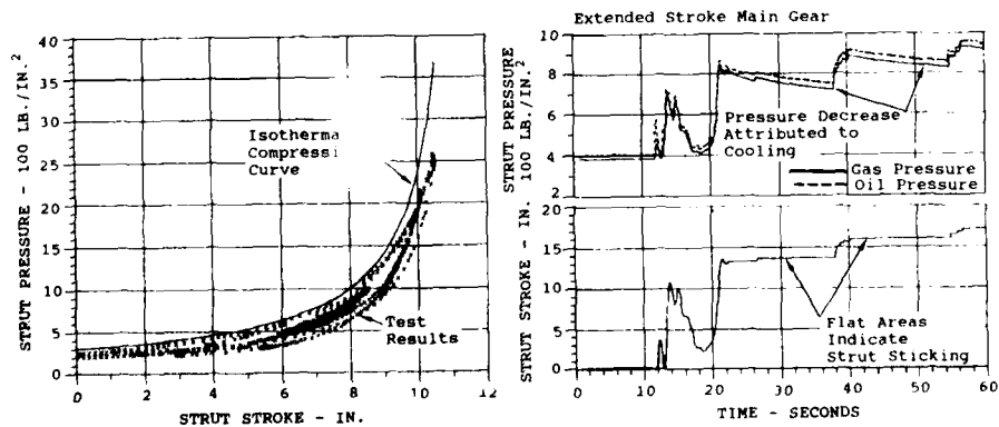
Figure 10. Example of Main Landing Gear Strut Friction during Landing Rollout.
