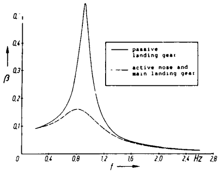
Pitch angle - Vertical excitation at the nose landing gear
