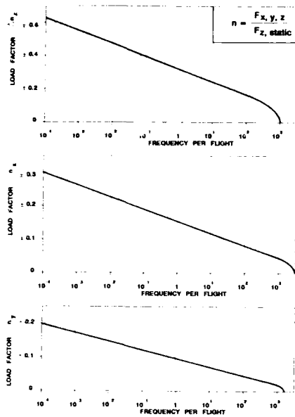
FIG.14 FREQUENCY DISTRIBUTIONS OF THE LOAD FACTORS ON THE MAIN LANDING GEAR DERIVED FROM A FIGHTER AIRCRAFT DURING UNBRAKED TAXING [ 17, 18 ]
