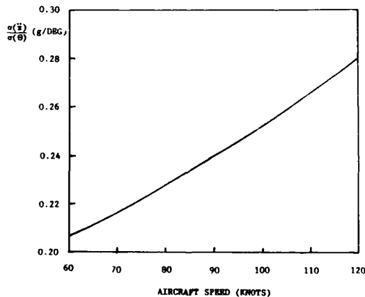
FIGURE 7. VERTICAL FORCES DUE TO SHIP PITCH
