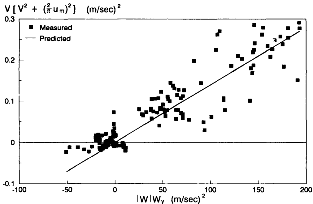
Figure 12. Wind-induced longshore current versus wind velocity
