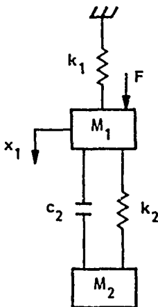
ABSORBER 2-DOF REPRESENTATION
