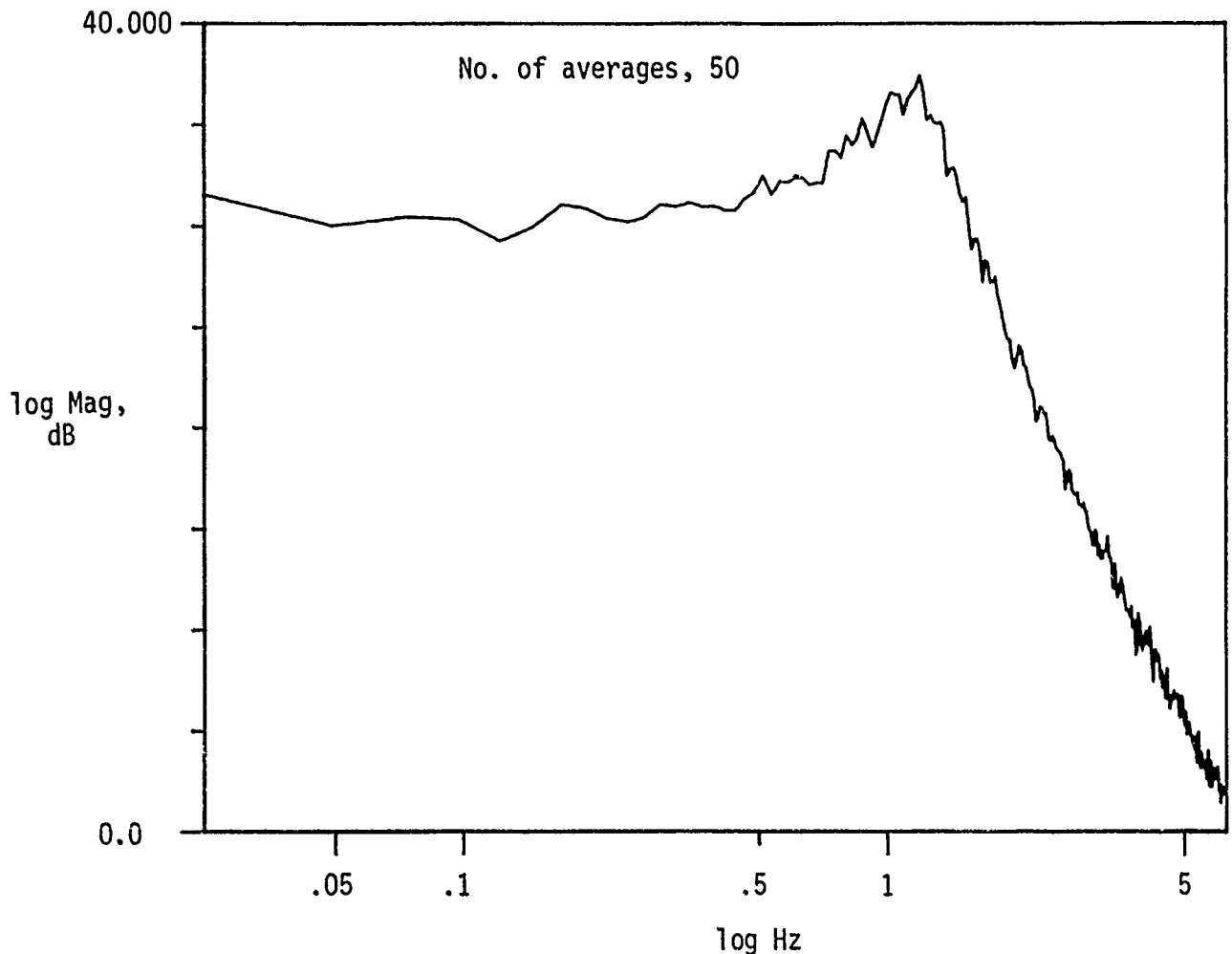
Modified LMED Frequency Response From Volts into Power Amp to Volts Out of LVDT
