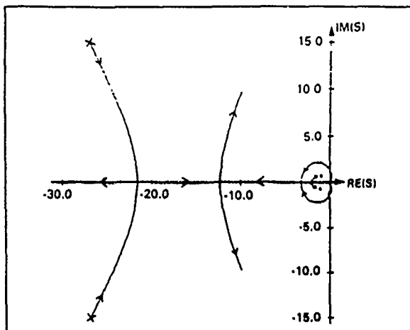
Fig. 8 Overall root locus.
