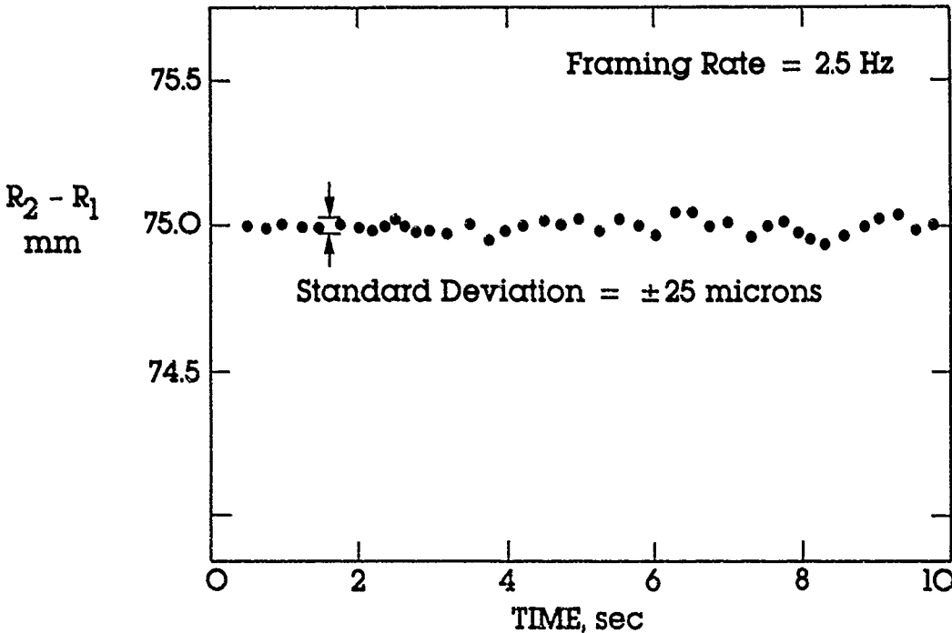
Experiment to Measure Range Resolution. Separation of T_1 and T_2 was Fixed at 75 mm to Obtain Streak Tube Calibration Factor.
