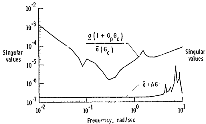
STABILITY CONDITION
