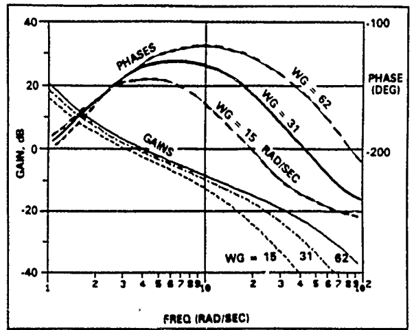
Fig. 15 Bode plots for three gyro bandwidths.
