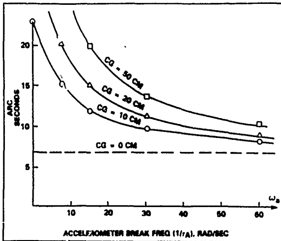
Fig. 16 Accelerometer time constant effect on pointing error.
