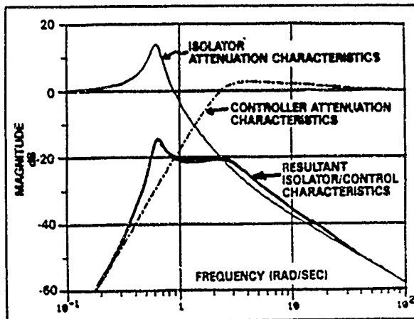
Fig. 18 Idealized isolation
