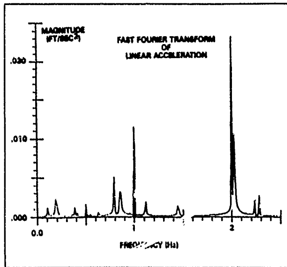
Fig. 5 Fast Fourier transform (FFT) of disturbance response - linear acceleration.
