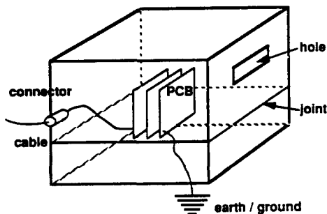
Fig. 2.10.1. Example of housing.
