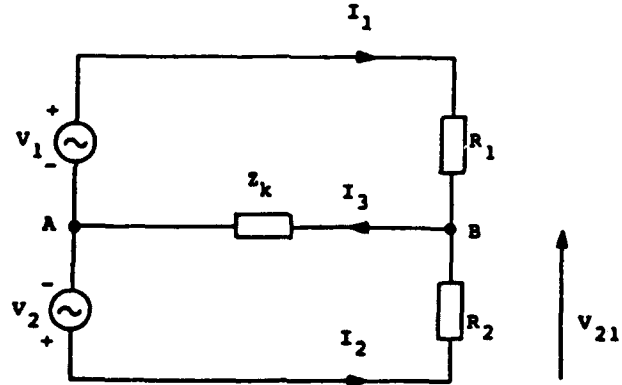
Fig. 2.1. Examples of common impedance.
