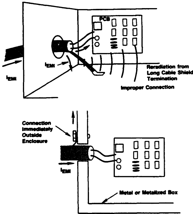
Fig. 2.15.4. Mounting of cables. (ref. D. White/ICT).
