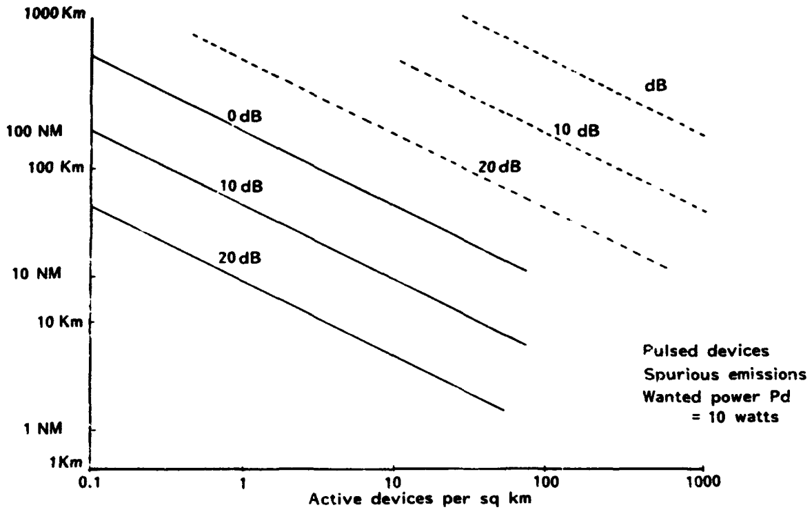
Figure 5 Range vs density of interferers for constant D/U ratio
