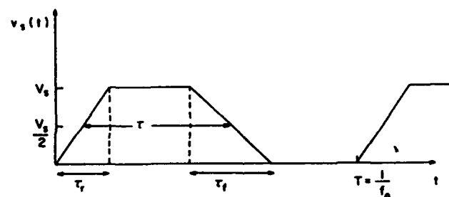
Fig. 10. A periodic, trapezoidal pulse train
