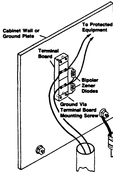
Fig. 2.12.3. Installation of protection device (Ref. D. White/ICT).
