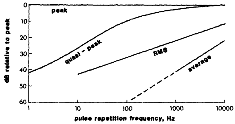
Fig 2.19. Detector Responses.
