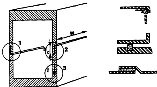
Fig. 2.3.2. : Joint techniques in box design (ref. Don White/ICT)
