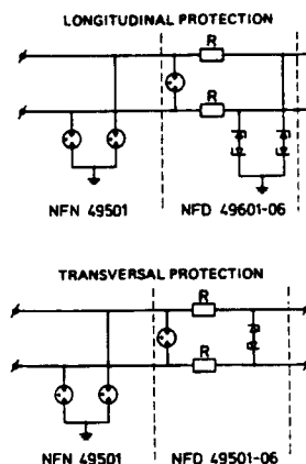
Fig. 2.12.1. Principle protection for electrical over stress.
