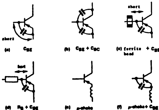
Fig.2.13.1 Avoiding HF signals to enter components.
