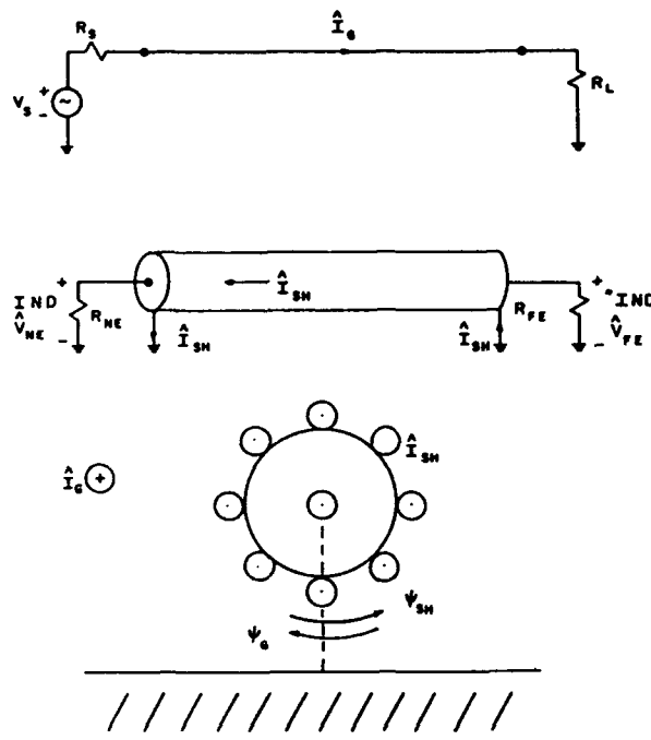
Fig. 14. Effect of a shield on inductive coupling
