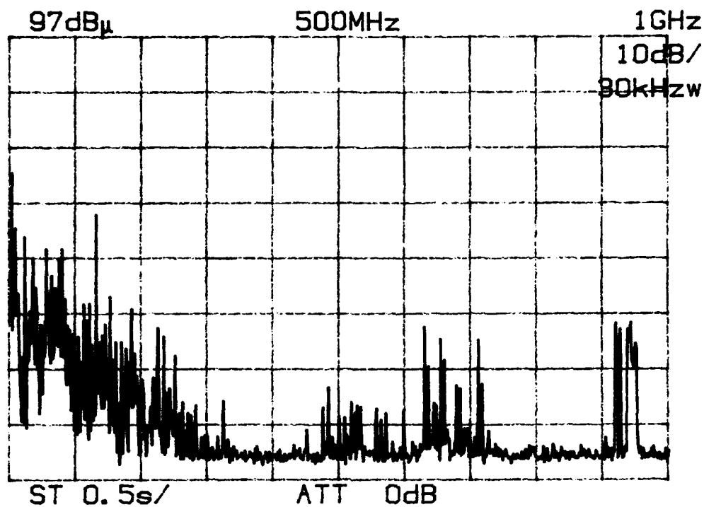
Fig 1.3. Ambient Radio Spectrum to 1GHz at York, U.K.
