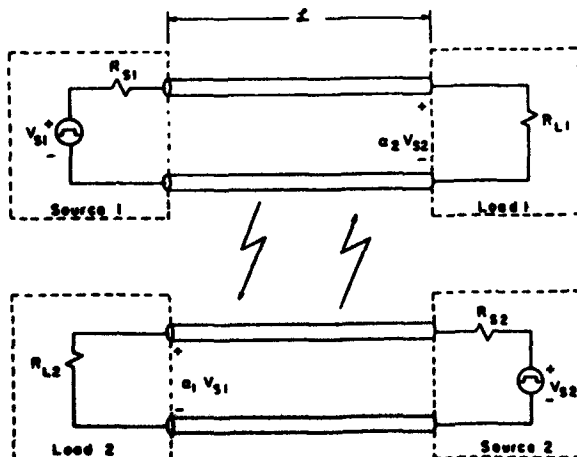
Fig. 1. Illustration of crosstalk
