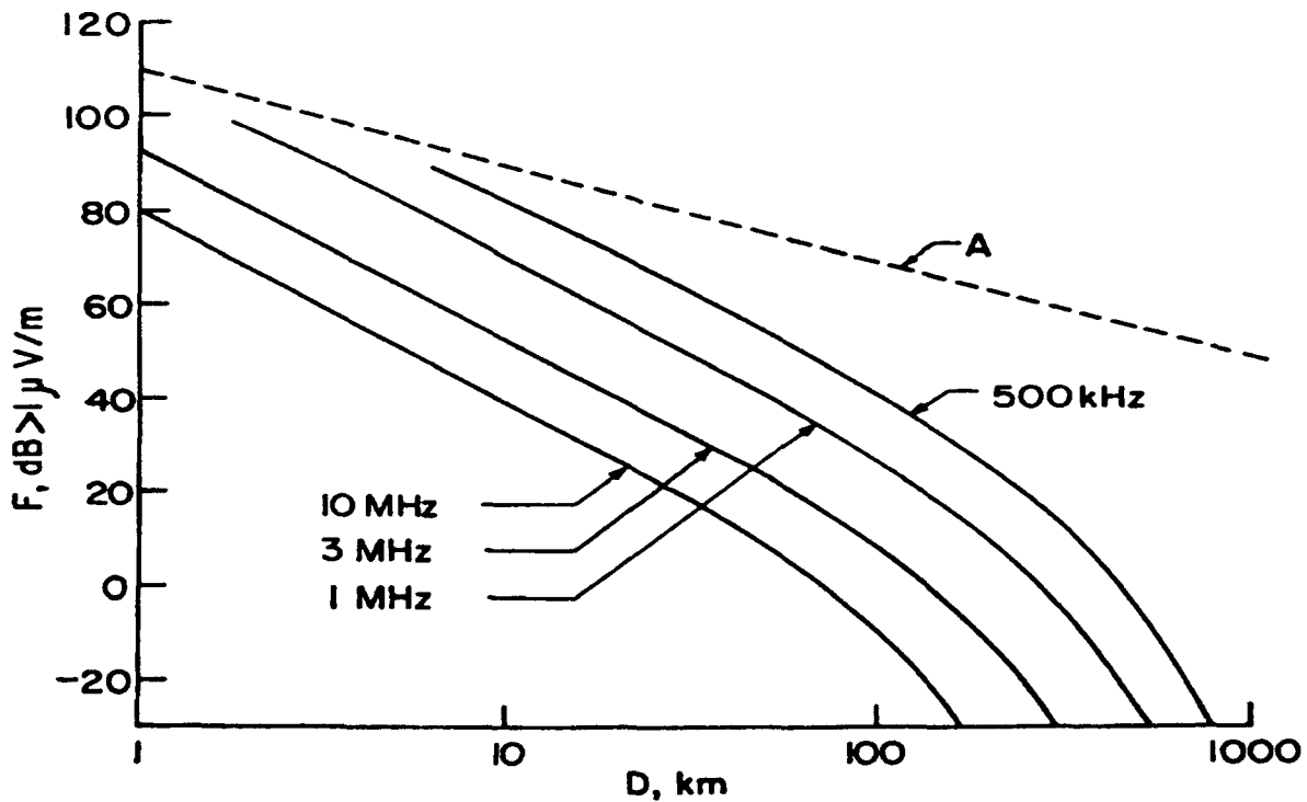
Figure 8: Groundwave Field-Strength variation with Distance (CCIR 368-2)
