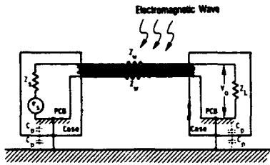
Fig. 2.4.1. Differential mode coupling.
