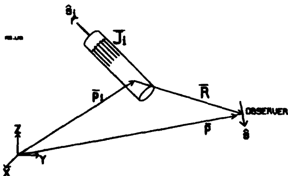
Fig. 12 A "thin wire" carrying current density \vec{J}_i gives rise to an electric field at the position of an observer.
