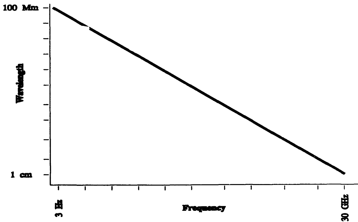
Figure 2: Relationship between wavelength and frequency for EM waves
