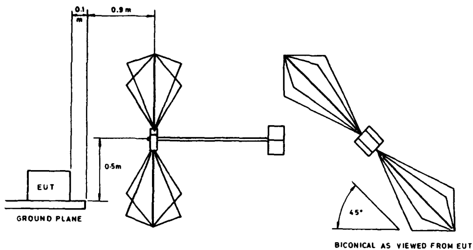
Fig 2.11. EUT and Antenna for 30 - 200MHz.
