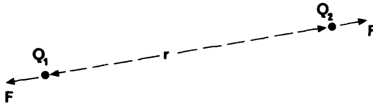
Figure 1.1 Illustration of the Forces between Two Point Charges.
