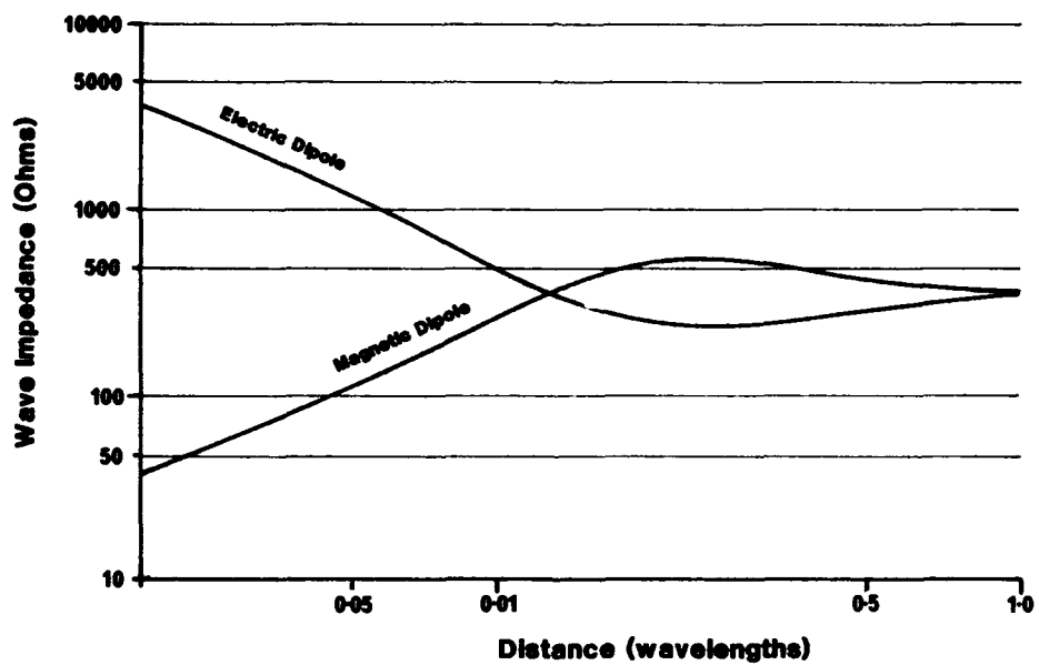
Figure 3.3 Plot of the Transverse Wave Impedances of Electric and Magnetic Dipoles.
