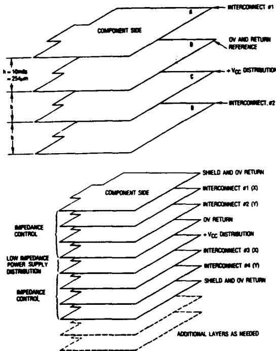
Fig. 2.15.1. Some multilayer PCB's.
