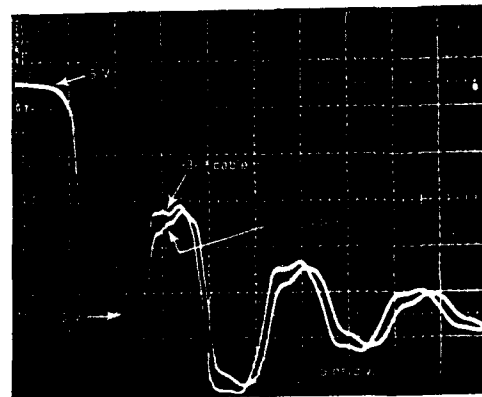
Fig. 2.9.2. Example of ringing due to line-reflections.
