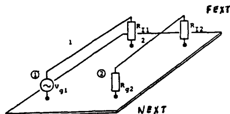
Fig. 2.8.1. Crosstalk of two wires.
