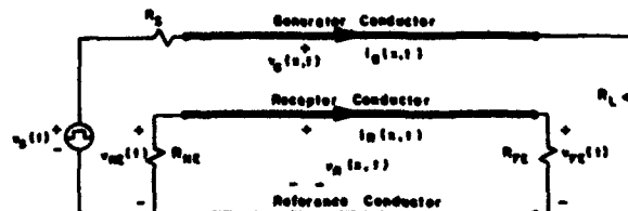
Fig. 2. A three-conductor transmission line
