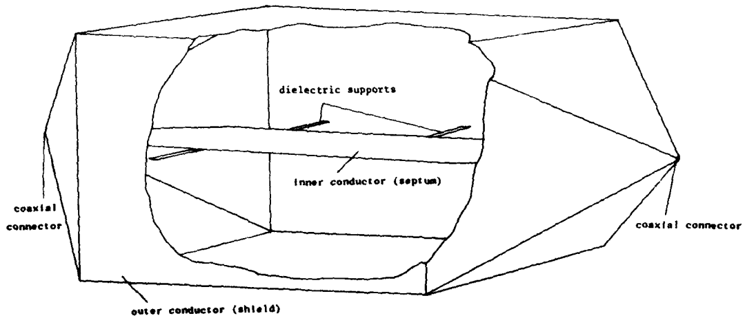
Fig 2.20. Cross-Section of a Crawford Cell.
