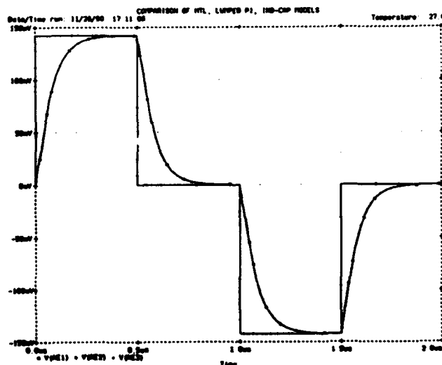
Fig. 11. Comparison of the time-domain predictions of the MTL, Lumped Pi, and inductive-capacitive coupling models for a trapezoidal pulse train
