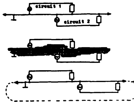
Fig. 1.1. : Common mode impedance coupling.
