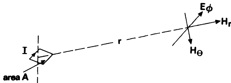
Figure 3.2 Field Components of a Magnetic Dipole.
