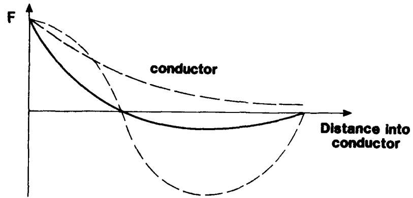
Figure 2.2 Wave Penetration into a Conductor.
