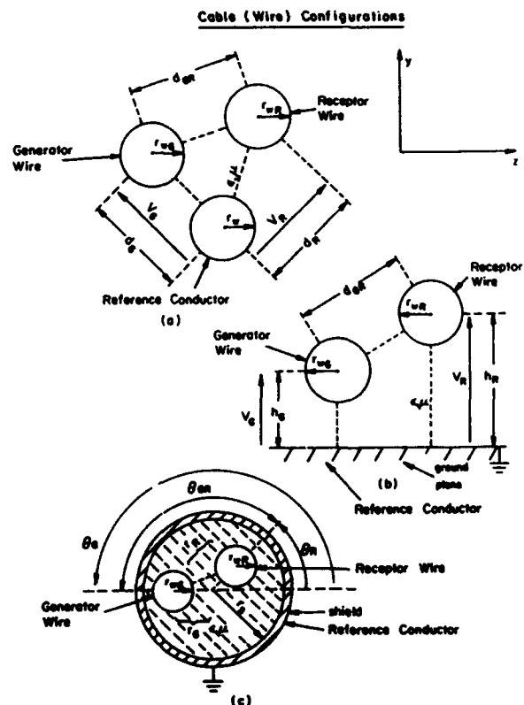
Fig. 3. Cross-sectional configurations of typical lines composed of wires in a homogeneous media
