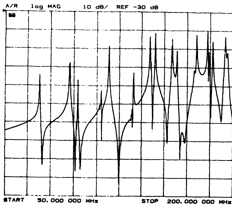
Fig 2.12. Frequency Response of Screened Enclosure 30 - 200MHz.
