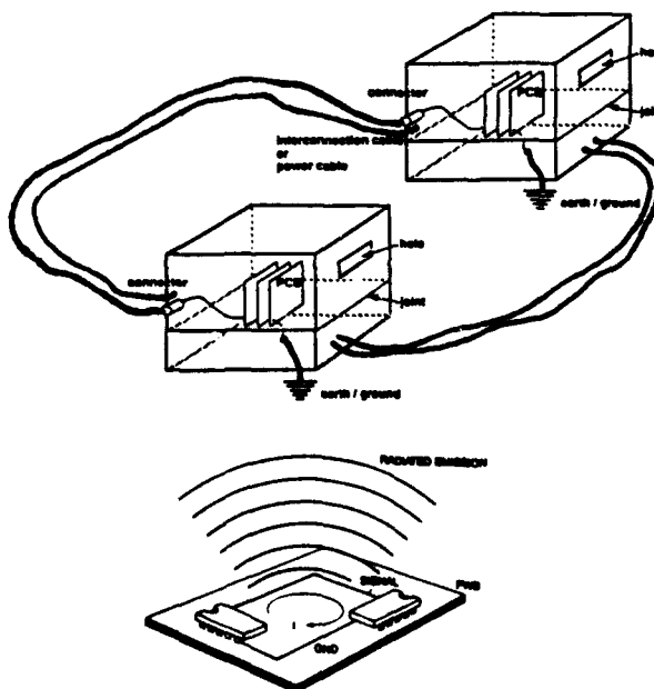
Fig. 2.2.2. Examples of CM in practice.
