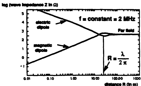
Fig.2.3.: Wave impedance.
