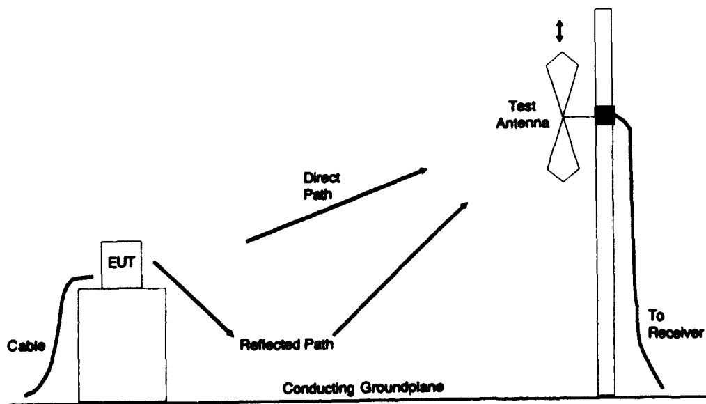
Fig 2.3. Side View of an OFTS.
