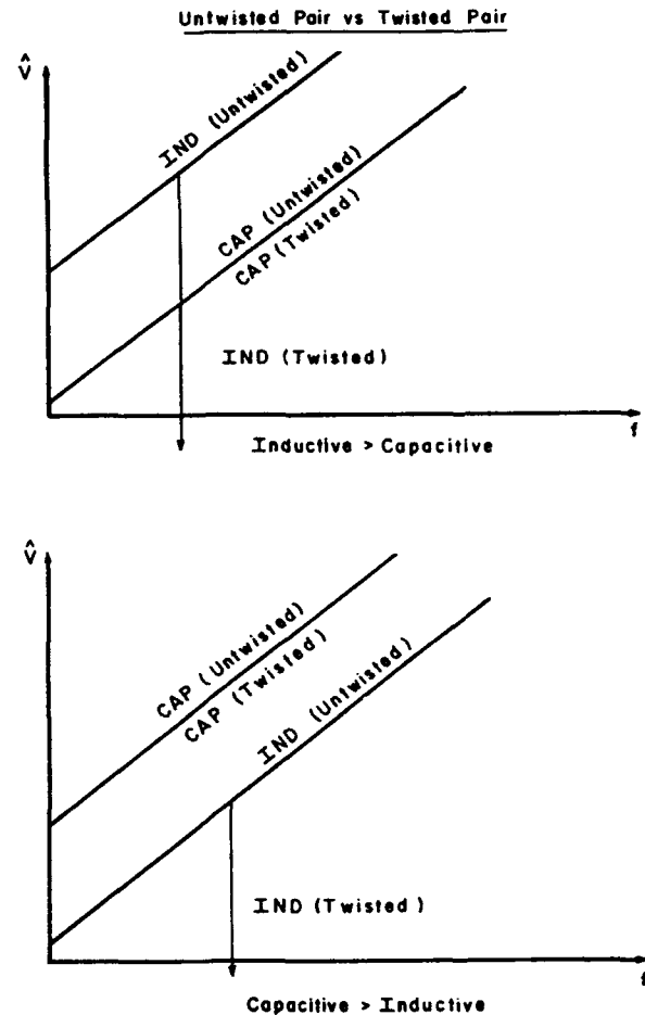
Fig. 22. Effect of twist on inductive and capacitive coupling for an untwisted pair compared to a twisted pair
