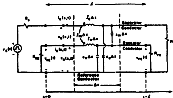
Fig. 5. The per-unit-length transmission-line model
