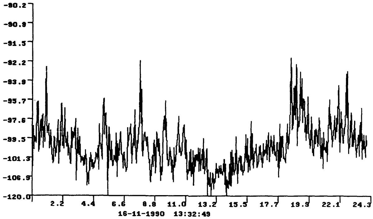
Figure 11: Diurnal variation of 47MHz Troposcatter received signal level
