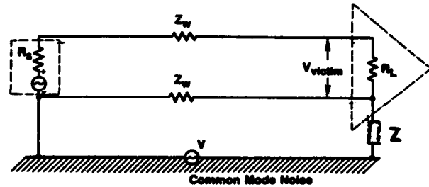
Fig. 2.3.1. Unbalanced system. (Ref. D. White/ICT)
