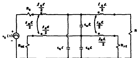
(b) Lumped Tee
