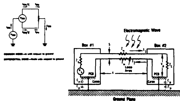
Fig. 1.6. : CM/DM coupling.
