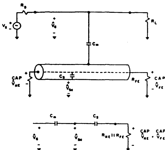
Fig. 13. Effect of a shield on capacitive coupling
