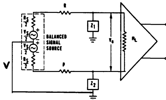
Fig. 2.3.2. Balanced system.
