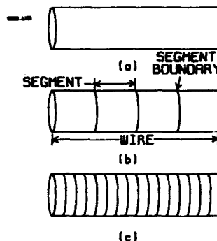
Fig. 13 A wire divided into segments, with various ratios of the segment length to the radius. (a) ratio 8; (b) ratio 2; (c) ratio 1/2.
