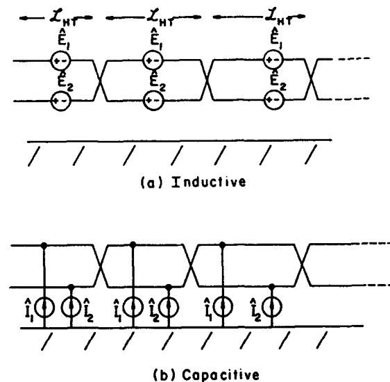
Fig. 20. Simplified model of coupling to a twisted pair
