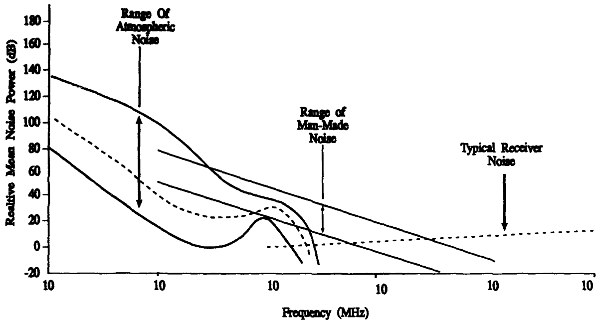
Figure 3: Variation Of Noise Power Level With Frequency for various sources
