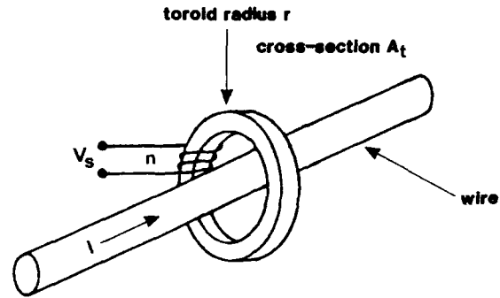
Fig 2.13. Current Transformer.
