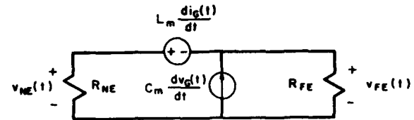
(b) Time-Domain Model
