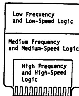
Fig. 2.15.2. Component placement on PCB.
