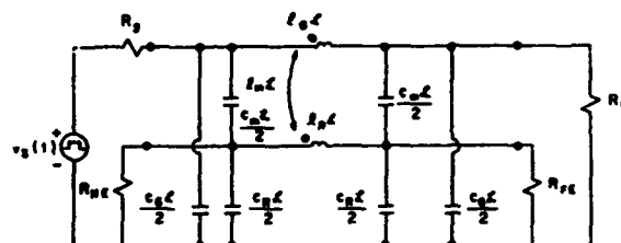
(a) Lumped Pi
