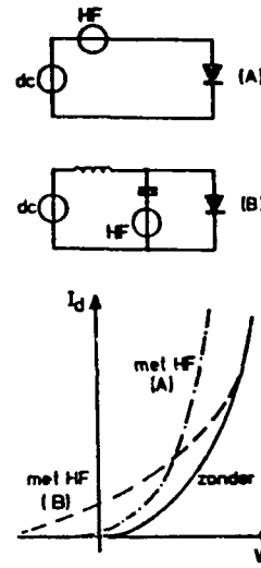
Fig. 2.13.2. DC-shift of diode-circuit due to HF demodulation.
