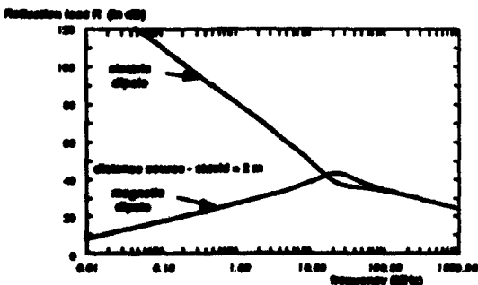
Fig. 2.4. : Reflection loss R as function of frequency
