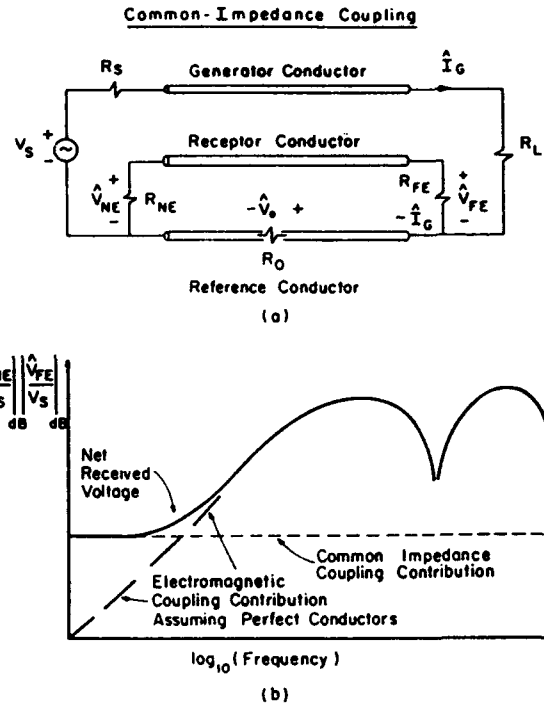
Fig. 12. Common-impedance coupling due to imperfect conductors
