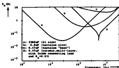
Fig. 2.11.2. Decoupling capacitors.
