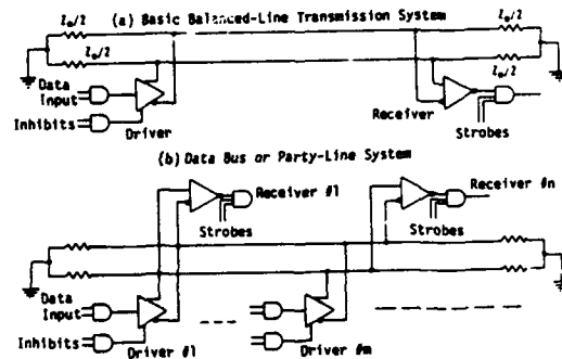
Fig. 2.9.1. Examples of "long-lines".
