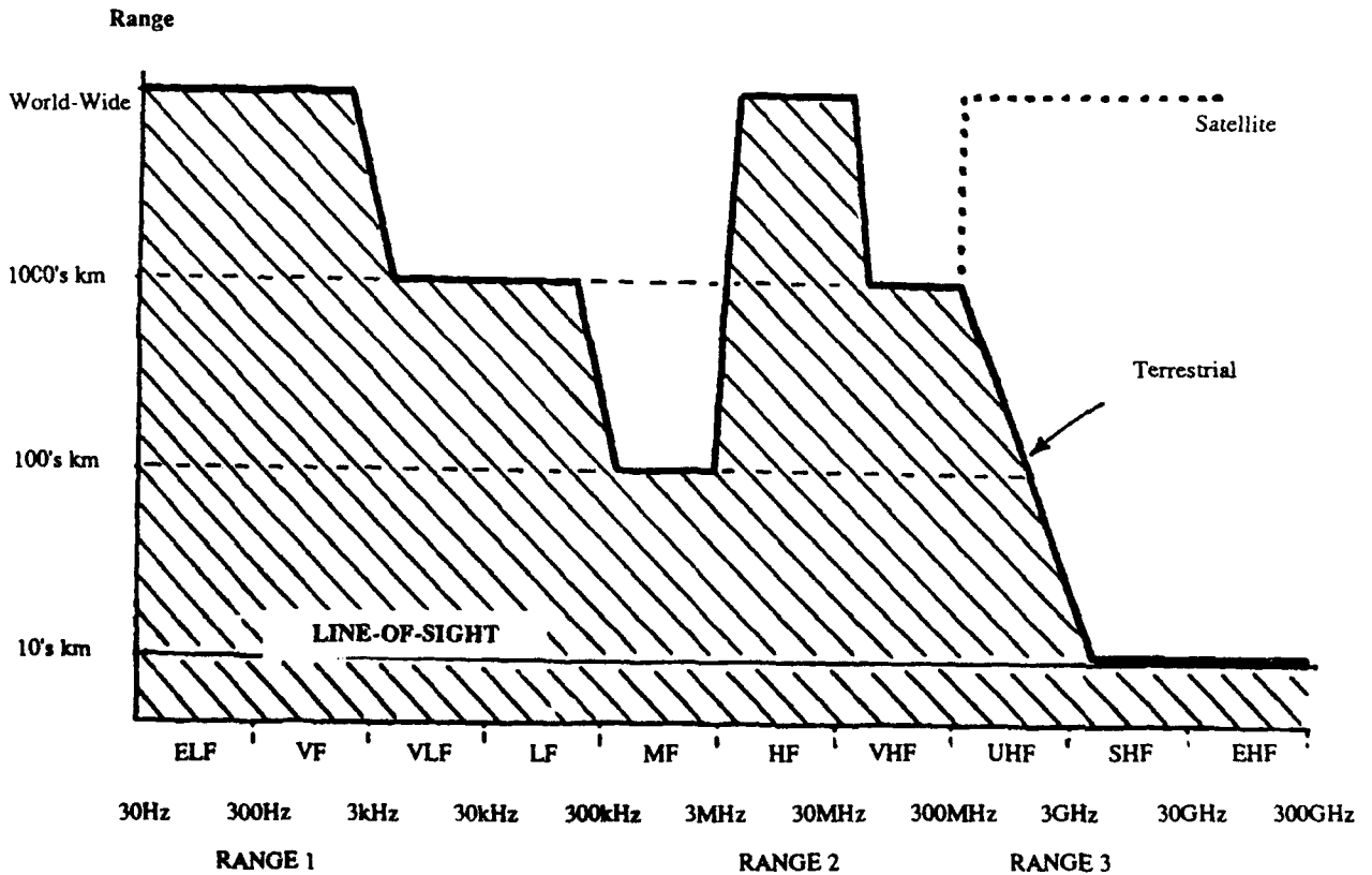
Figure 4: Variation of Radio System Range With Frequency
