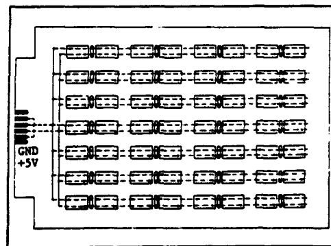
- Better Layout Reduce Power Distribution and Logic-Return Impedances, Trace Crosstalk and Board Radiation.
