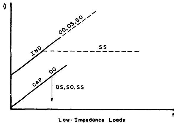
Fig. 16. Effect of shield grounding on inductive coupling for a shielded receptor wire
