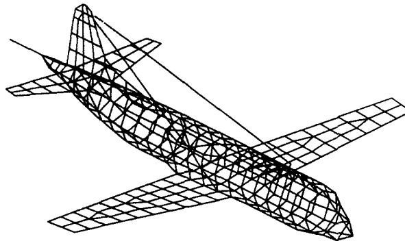
Fig. 17 "Elegant" Aircraft Model, 685 segments
