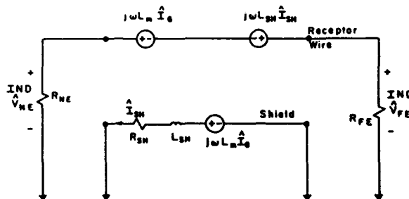
Fig. 15. Simplified model for inductive coupling to a shielded receptor wire
