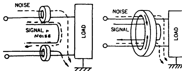
Fig. 2.7.2. Ferrite beads.
