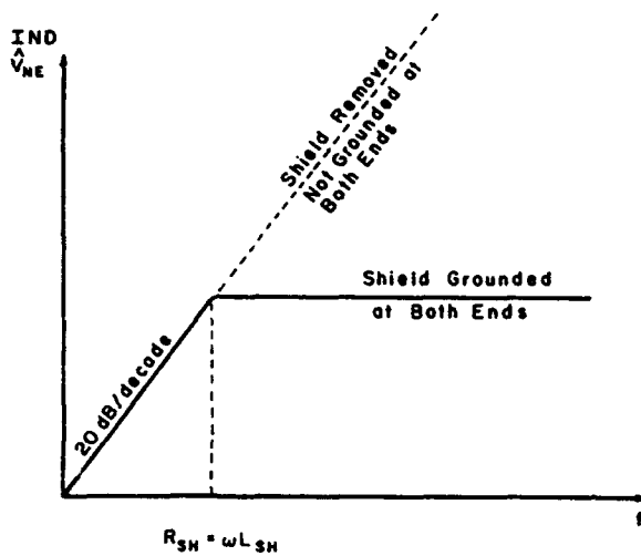
Fig. 16. Effect of shield grounding on inductive coupling for a shielded receptor wire
