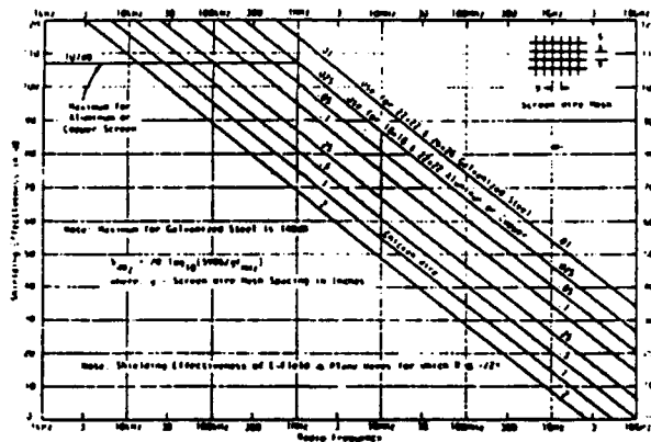
Fig. 2.10.3. SE of a grid. (Ref. D. White/ICT)
