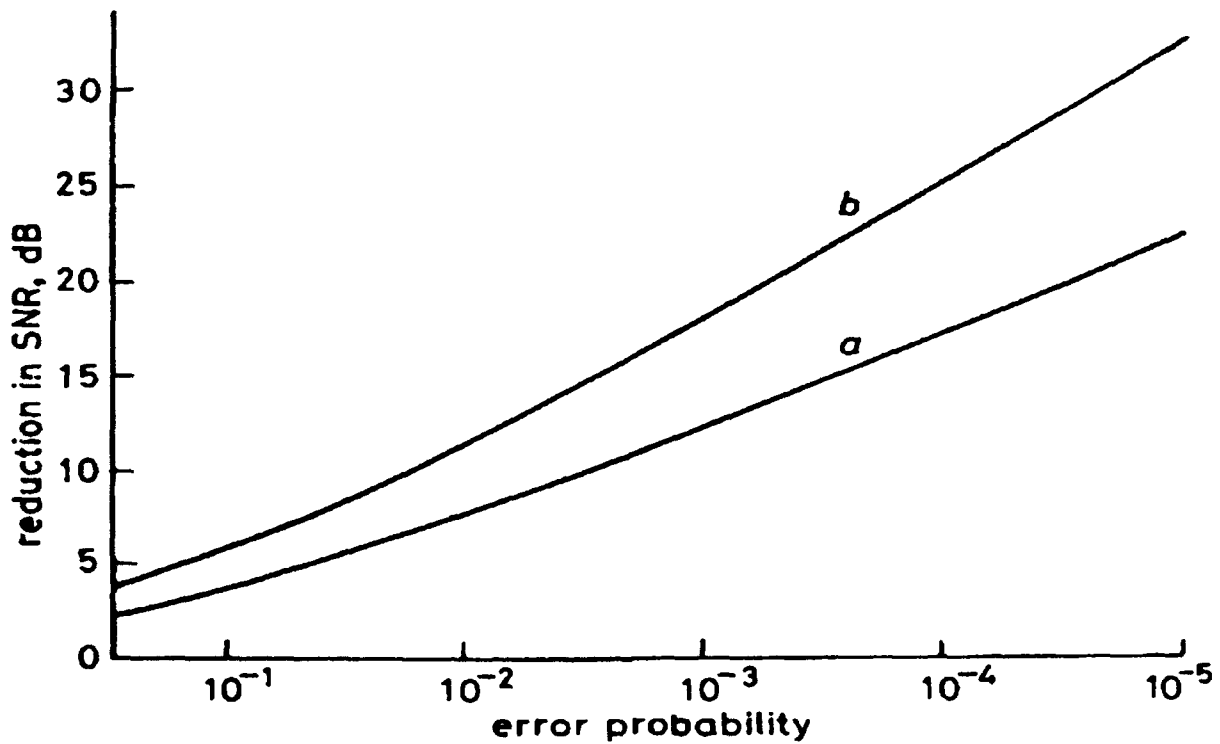
Figure 15: Reduction in SNR required at receiver using 2nd and 4th order diversity
