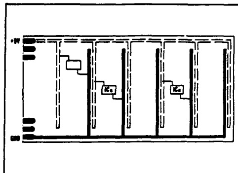
A Bad Layout Giving High Inductance and Few Adjacent Signal Return Paths, Which Leads To Crosstalk.
