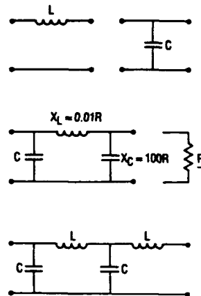
Fig. 2.7.1. Basic filter components.
