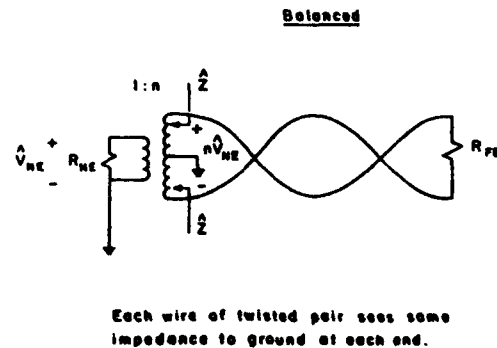
Fig. 18. Twisted pair configurations for unbalanced and balanced modes
