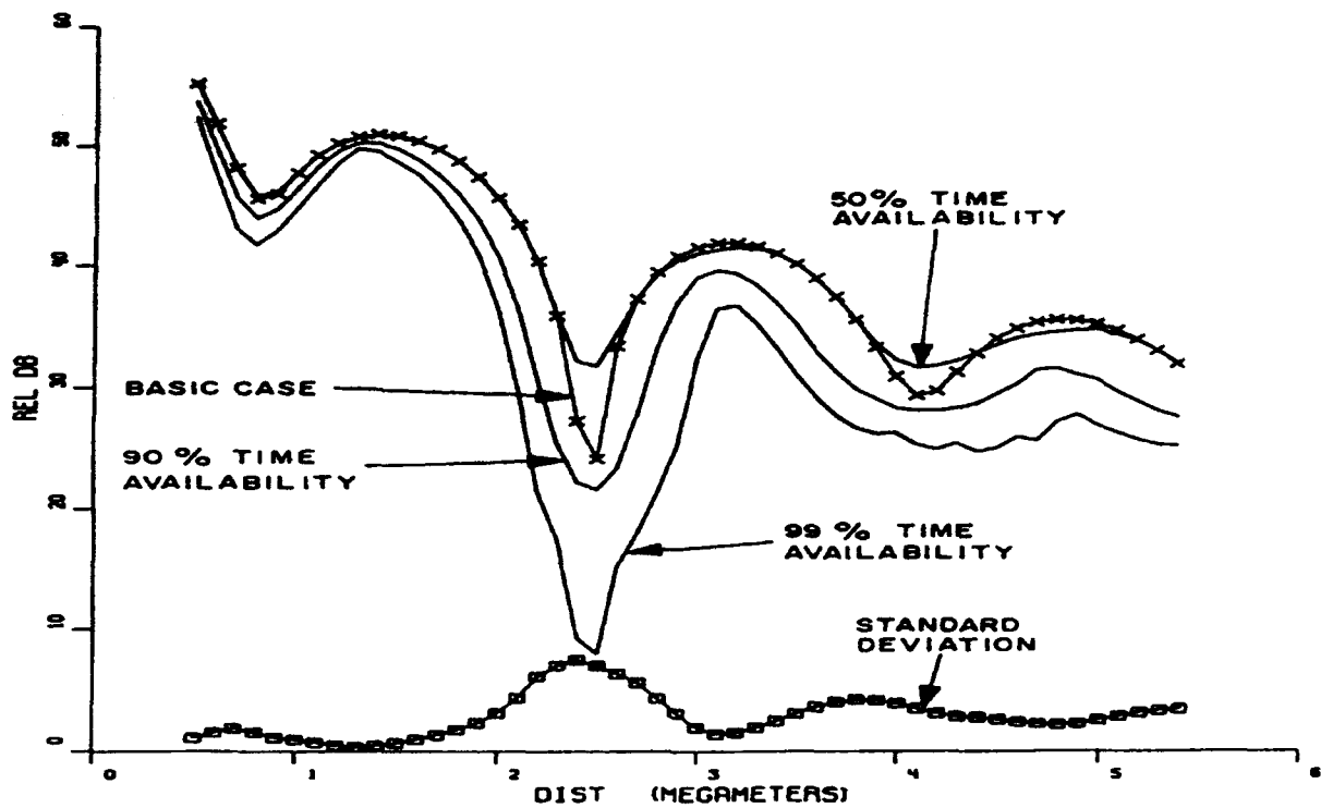
Figure 7: VLF Field Strength variations with Distance (Kelly 1986)
