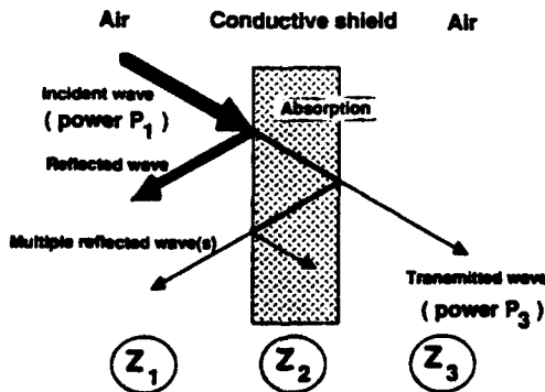
Fig. 2.2. : Shielding of materials.
