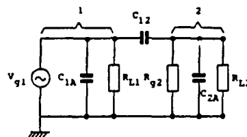
Fig. 2.8.2. Capacitive crosstalk.
