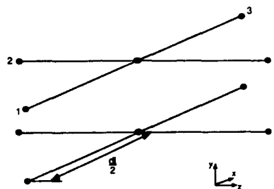
Fig. 19 TLM 2D node made up of parallel wire transmission line.
