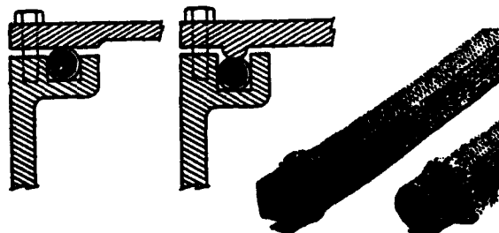
Fig.3.2.: Applying a gasket in practice
