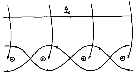
Fig. 19. Effect of a twisted pair on inductive coupling
