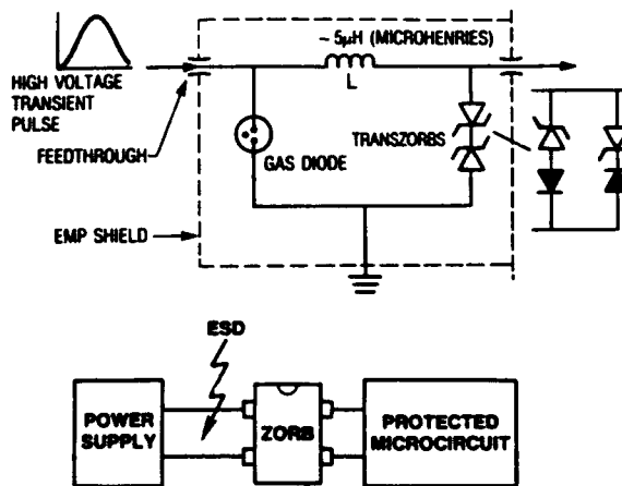
Fig. 2.12.2. Typical protection devices.
