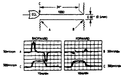
Fig. 2.8.4. Example of crosstalk.
