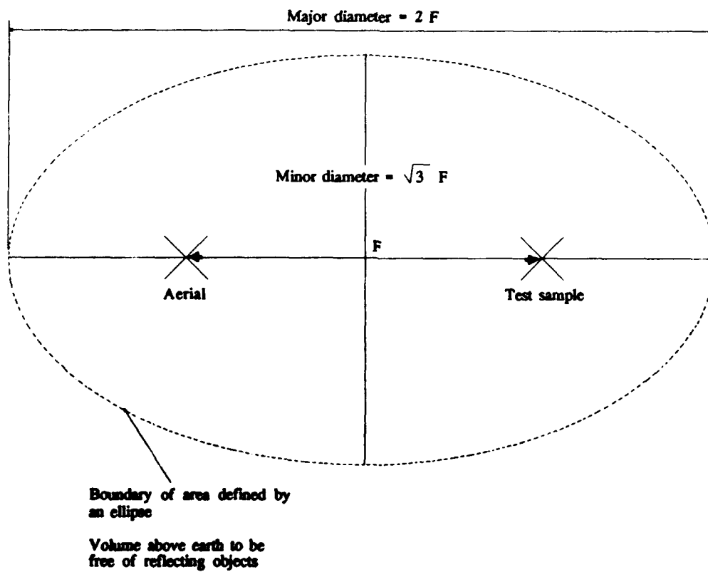
Fig 2.1. Plan View of an OFTS.
