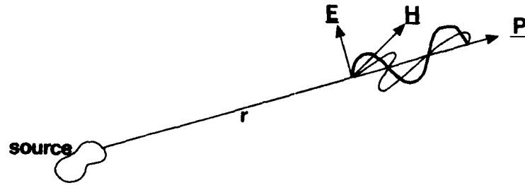
Figure 2.1 A Spherical Electromagnetic Wavefront.
