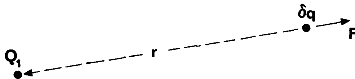
Figure 1.2 Derivation of the Electric Field of a Point Charge.
