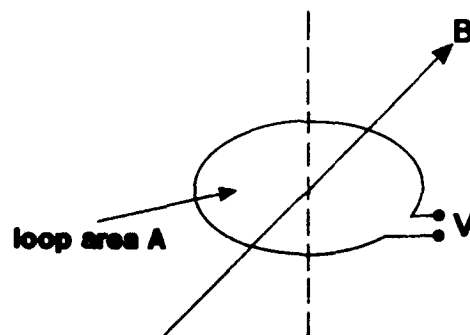
Figure 1.4 Illustration of Faraday's Law of Induction.
