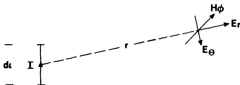
Figure 3.1 Field Components of an Electric Dipole.
