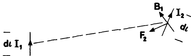
Figure 1.3 Illustration of the Magnetic Force between Two Current Elements.
