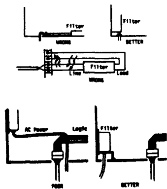
Fig. 2.6.2. Mounting of power line filter.
