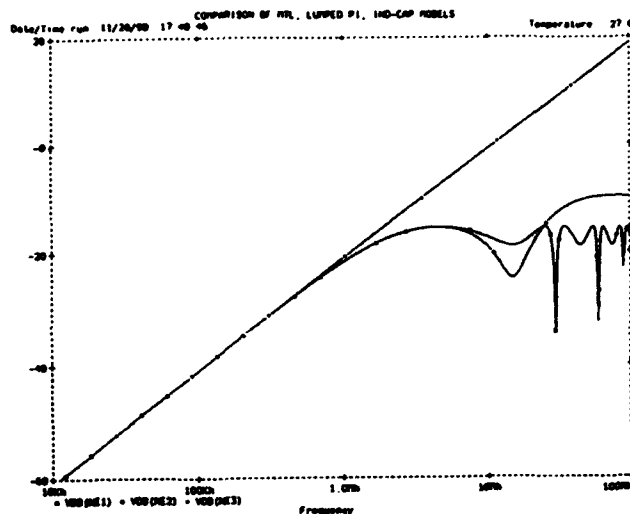
Fig. 9. Comparison of the frequency-domain predictions of the MTL, Lumped Pi, and inductive-capacitive coupling models
