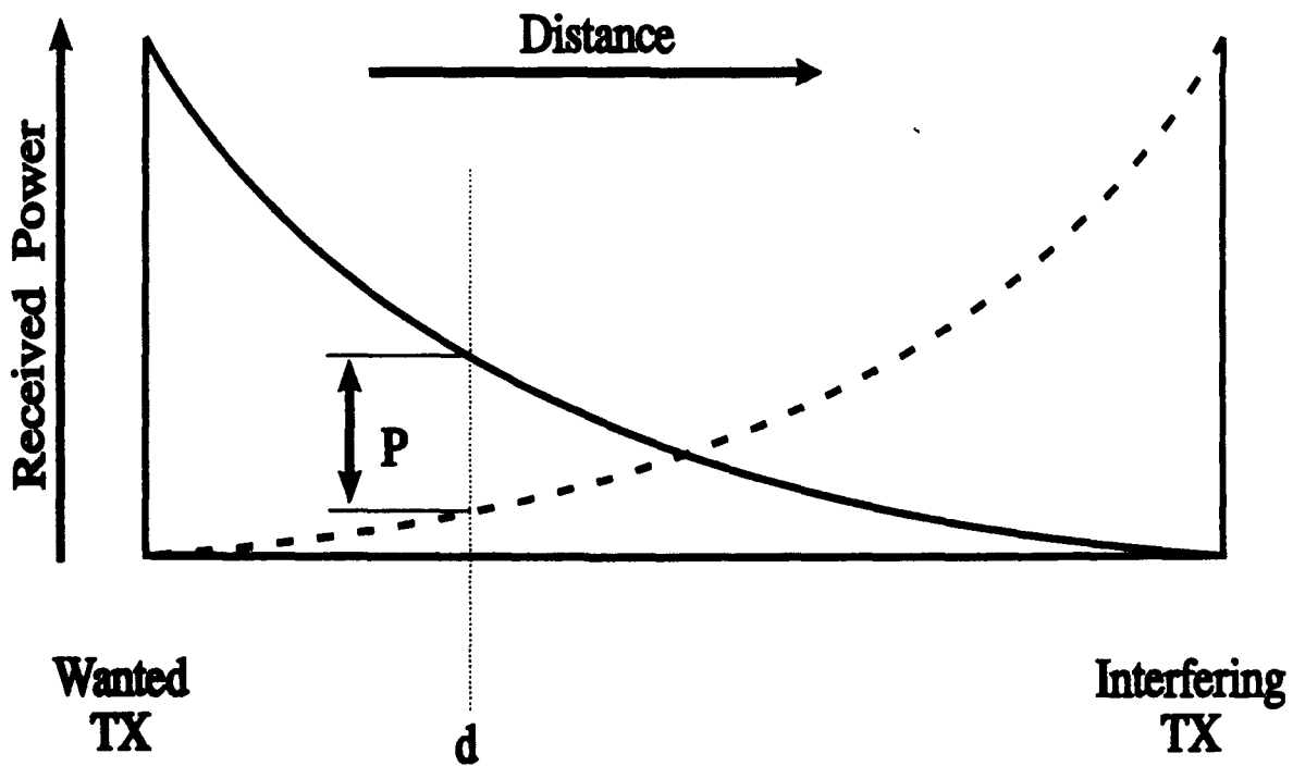
Figure 17: Illustration of frequency dependent rejection
