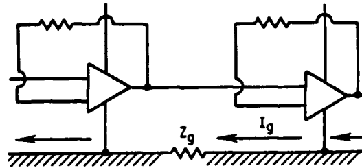
Circuit-example (op-amp design)
