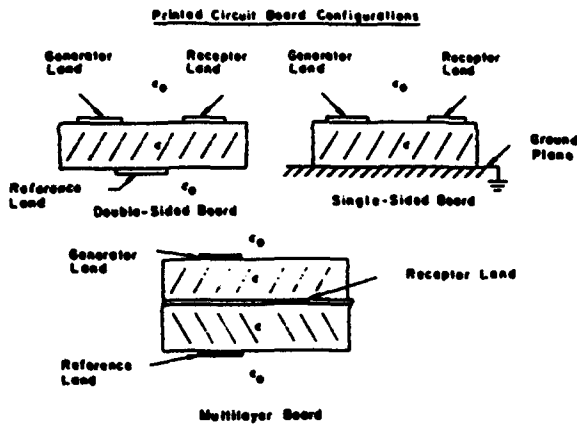
Fig. 4. Crosssectional configurations of PCB lands
