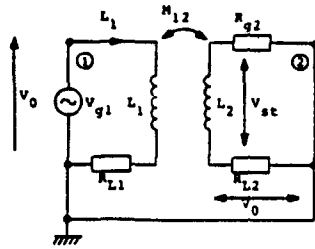
Fig. 2.8.3. Inductive coupling.
