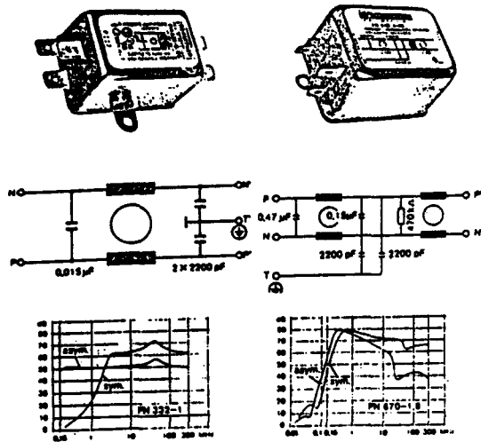
Fig. 2.6.1. Power line filters.
