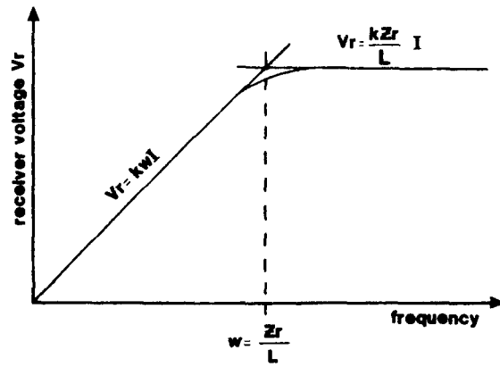
Fig 2.14. Frequency Response of Current Transformer.
