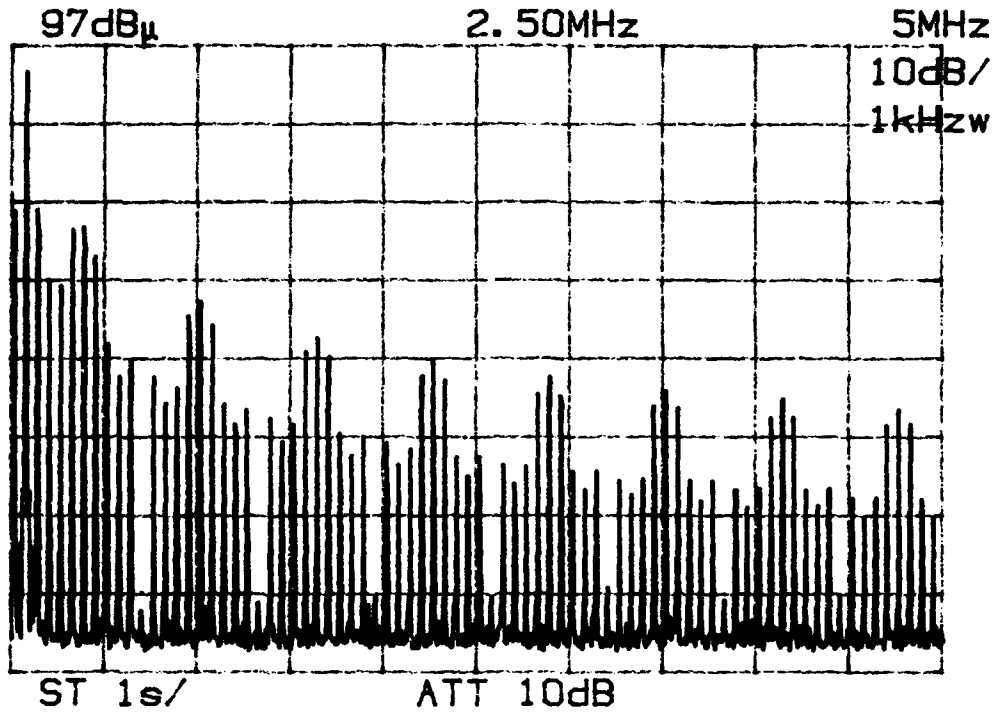
Fig 1.1. Spectrum of Harmonics from a Digital Circuit.
