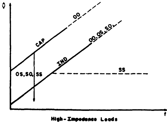
Fig. 17. Effect of shield grounding on crosstalk to a shielded wire
