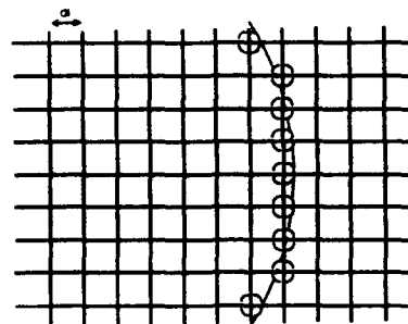
Fig. 18(b) Wavefront superimposed on TLM mesh showing approximate scattering centres.
