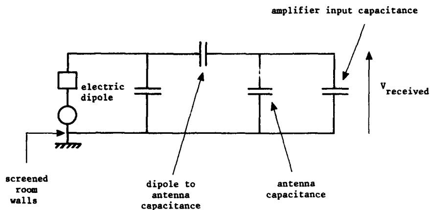
Fig 2.8. Equivalent Circuit for EUT to Antenna Capacitive Coupling.
