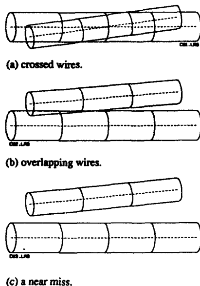
Fig. 15 Wire spacing errors for nearly parallel wires.
