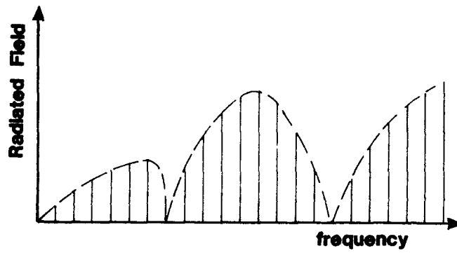
Figure 4.2 Radiated Spectrum of a Digital Pulse Train.
