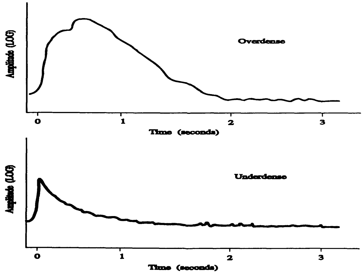
Figure 10: Amplitude-Time Profiles of signals via meteor trails
