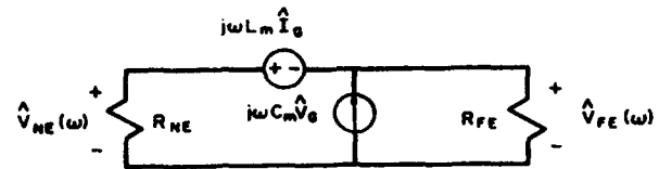
(a) Frequency-Domain Model
