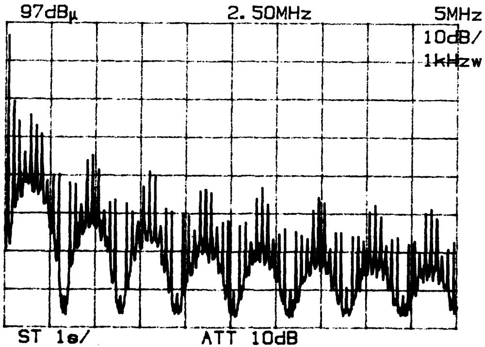
Fig 1.2. Continuous Spectrum of Digital Data.
