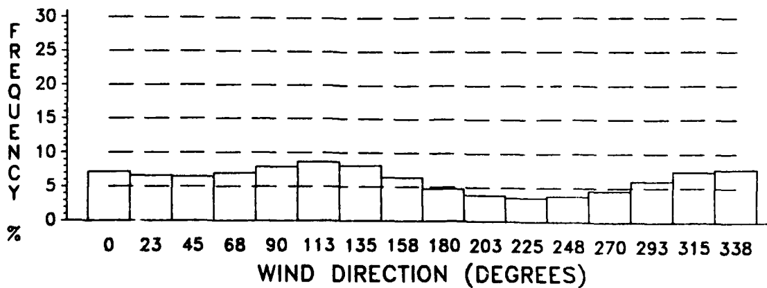
Figure E-6. Wind Direction Frequency, January, 50 KM.
