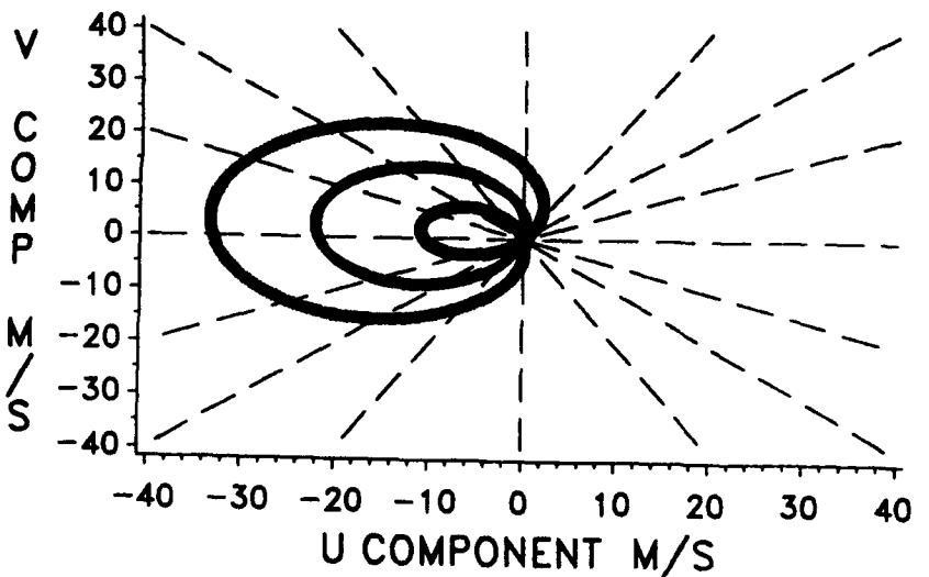
Figure E-31. Wind Interpercentile Range and Mean, July, 60 KM.
