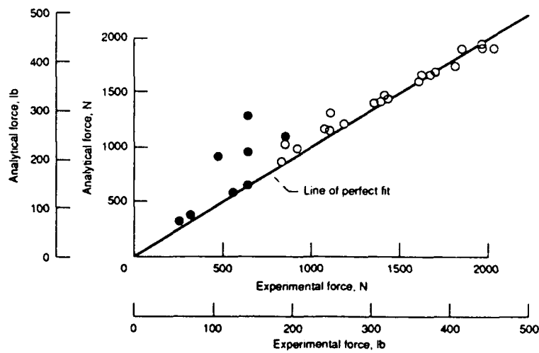
Fig. 8.—DANST predictions for peak force compared to experimental data (data from two lowest torque levels shown as solid symbols).
