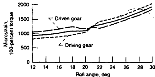
(a) Single-tooth loading
