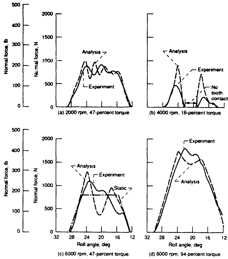
Fig. 7.—DANST force predictions compared to strain gage data.
