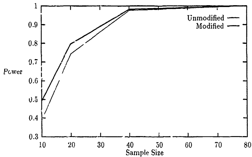
Figure 4.6. Cramer von Mises Power Test for the Exponential Distribution with the Median Rank
