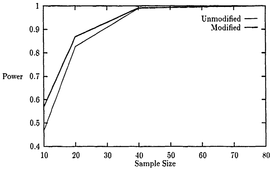
Figure 4.10. Cramer-von Mises Power Test for the Double Exponential Distribution with the Median Rank
