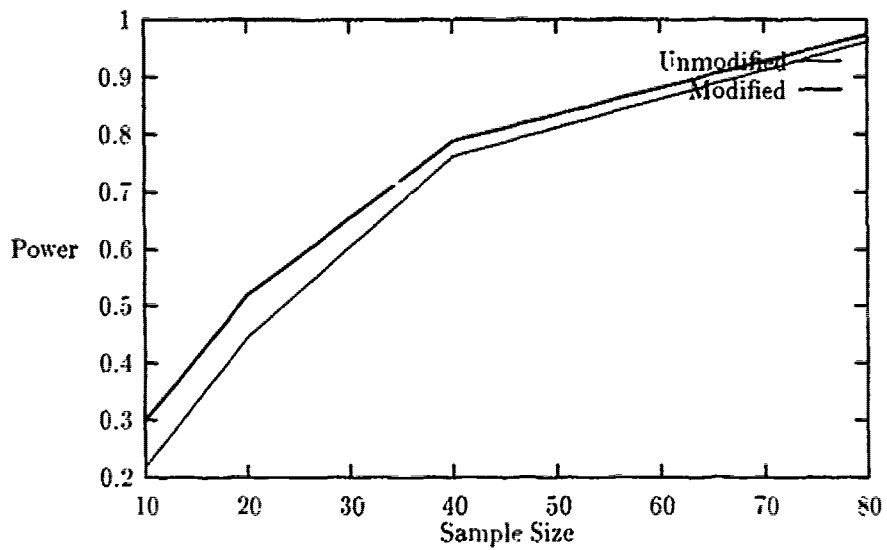
Figure 4.4. Cramer-von Mises Test for the Weibull Distribution with the Median Rank
