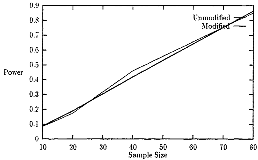
Figure 4.11. Anderson-Darling Power Test for the Uniform Distribution with the Mean Rank
