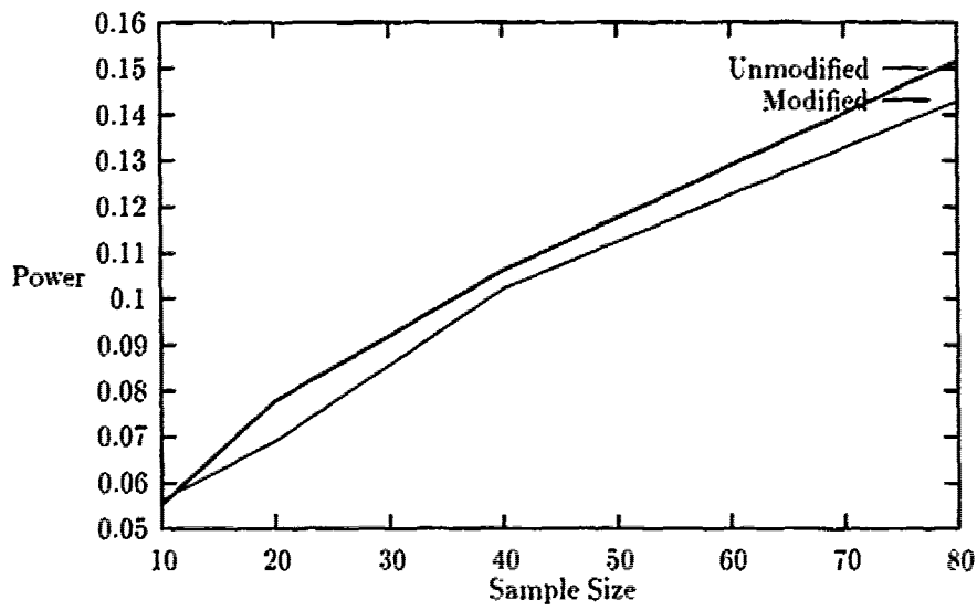
Figure 4.14. Cramer-von Mises Power Test for the Weibull Distribution with the Mean Rank
