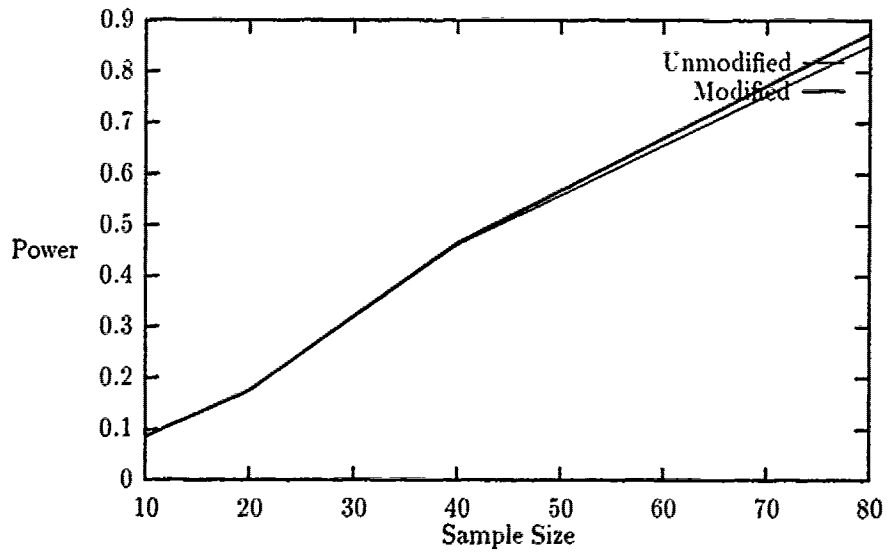
Figure 4.1. Anderson-Darling Power Test for the Uniform Distribution with the Median Rank
