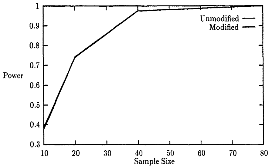
Figure 4.16. Cramer-von Mises Test for the Exponential Distribution with the Mean Rank
