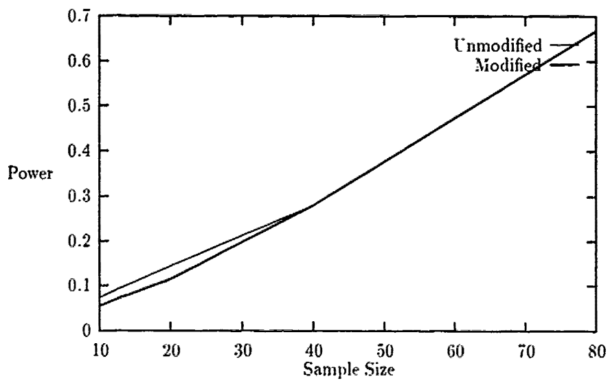
Figure 4.2. Cramer-von Mises Power Test for the Uniform Distribution with the Median Rank
