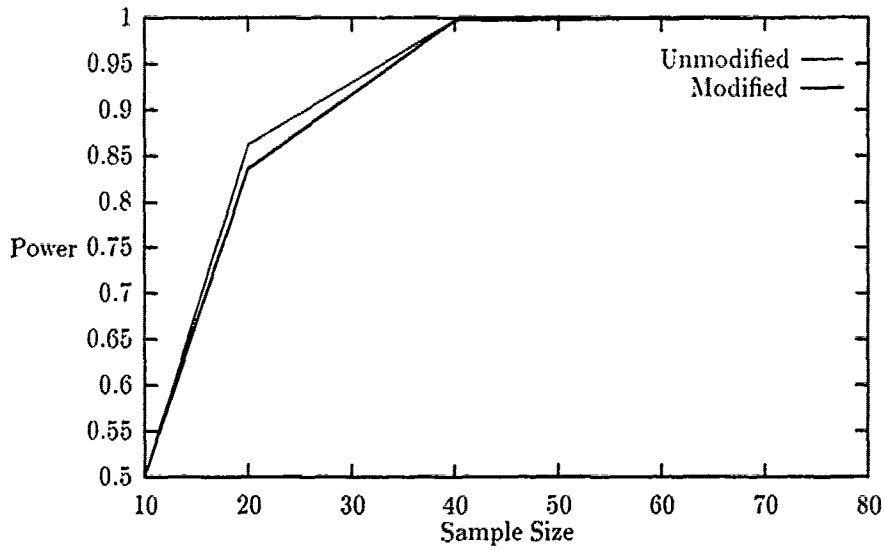
Figure 4.9. Anderson-Darling Power Test for the Double Exponential Distribution with the Median Rank
