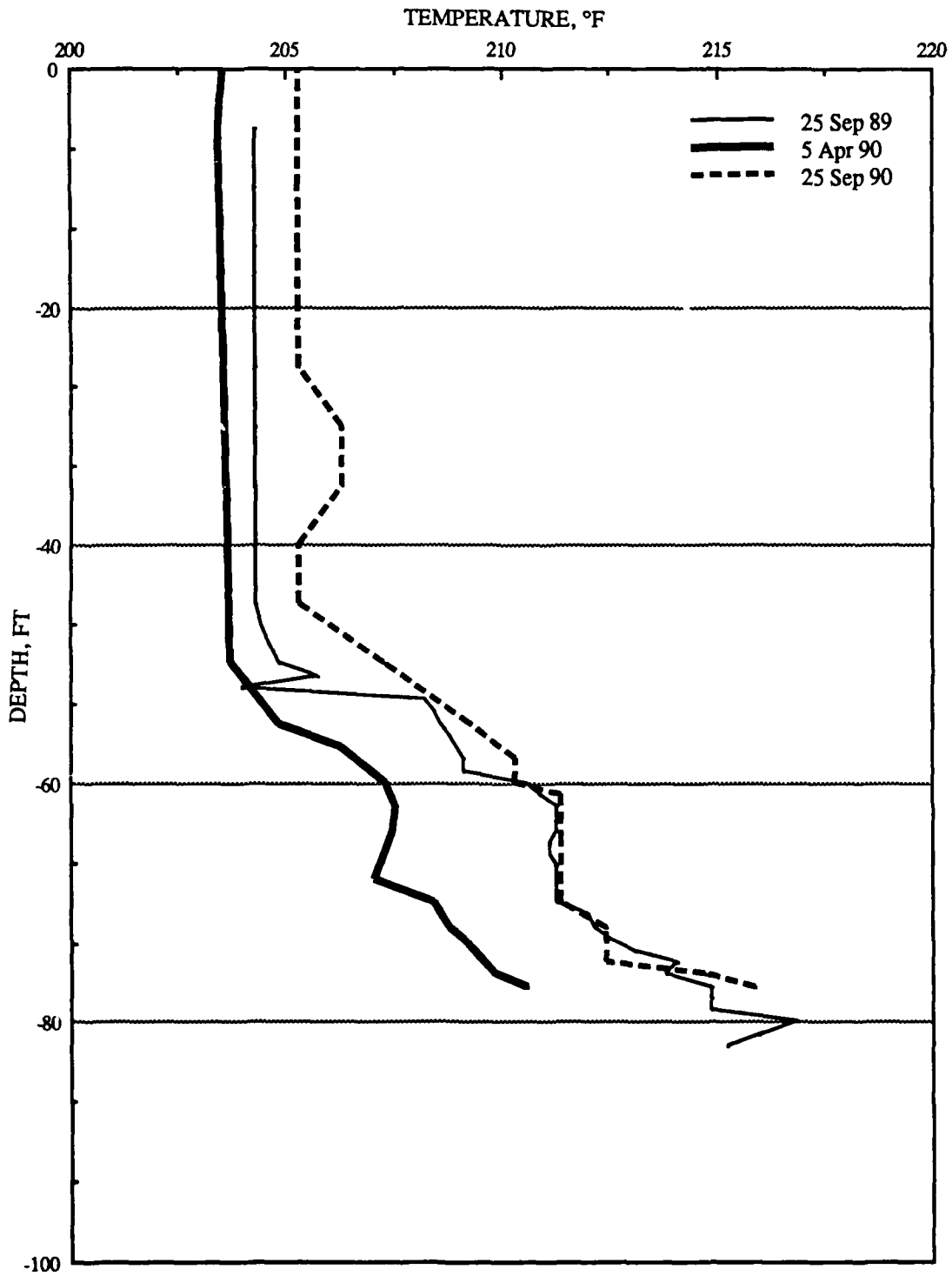
FIGURE 30. Temperature Profile, Well 4K-1.
