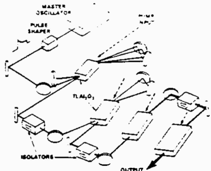
MH1 Fig. 1. Schematic of the \text{Ti:Al}_2\text{O}_3 amplifier system. The master oscillator is a cw \text{Ti:Al}_2\text{O}_3 single frequency ring laser. The \text{Ti:Al}_2\text{O}_3 amplifier consists of four stages: a four-pass preamplifier, a two-pass amplifier, and two single-pass amplifiers. The pump source is a frequency doubled Nd:YAG laser.
