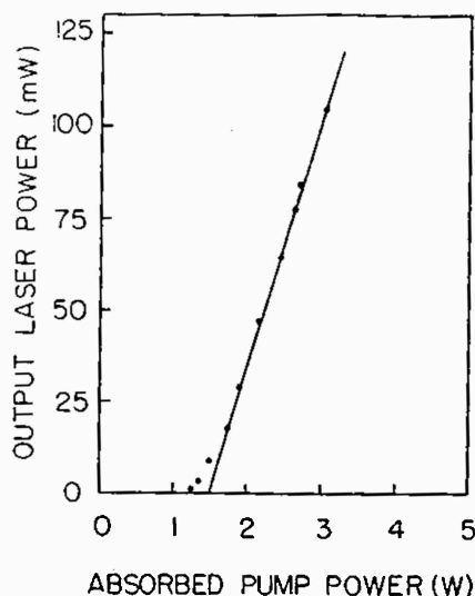
Fig. 9 Output power of the cw Cr:Mg 2 SiO 4 laser as a function of absorbed pump power.
