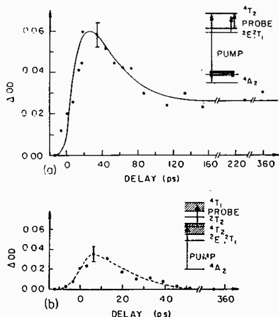
Fig. 1. Time evolution of the optical density (a) at 3.9 \mu\text{m} , and (b) at 2.16 \mu\text{m} in the metastable ( ^2E + ^2T_1 ) state and the ZVL and LLV levels of the ^4T_2 state of emerald at room temperature. The radii of the pump and the probe pulses at the sample position are both 0.35 mm. Both the pump and the probe pulses are linearly polarized parallel to the c_3 axis of the crystal. Insets show the relevant energy-level diagrams of emerald, and the pump, probe and relaxation transitions. The zero time is accurate within 5 ps. Size of a typical error bar is shown. The solid curve in (a) is a computer fit to the experimental data using the rate equations and relaxation rates described in the text.
