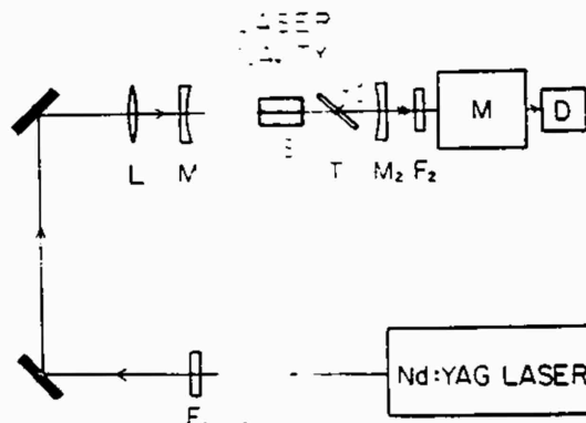
Fig. 1. Schematic diagram of the experimental arrangement used for wavelength tuning the Cr:forsterite laser: F_1 = 1064-nm transmitting, visible blocking filter; F_2 = pump beam blocking, laser output transmitting filter; L = focusing lens; M_1 = back mirror; M_2 = output mirror; S = sample; T = birefringent plate tuning element; M = monochromator, and D = detector.
