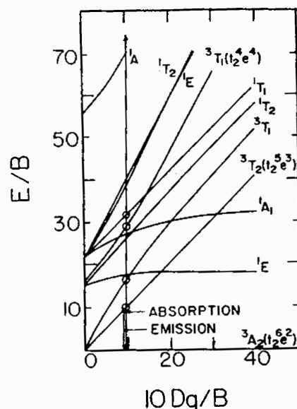
Fig. 3 Tanabe-Sugano diagram for \text{Cr}^{4+} in tetrahedral coordination. The values Dq=915 \text{ cm}^{-1} and B=970 \text{ cm}^{-1} were used to assign transitions shown in Fig. 1 and listed in Table 1.
