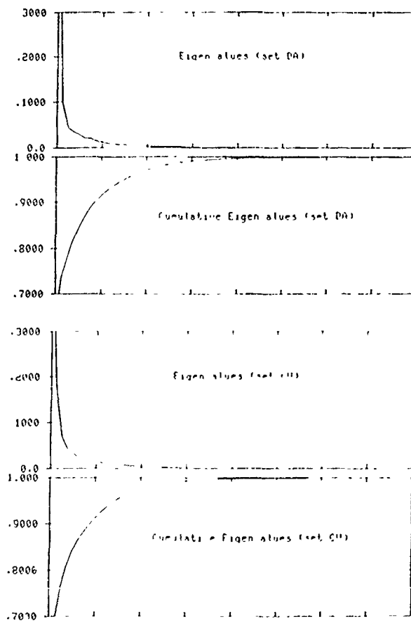
Figure 2.13 Correlation Matrix and Eigenvalue Characteristics Speech, Magnitude DFT, Linear Frequency
