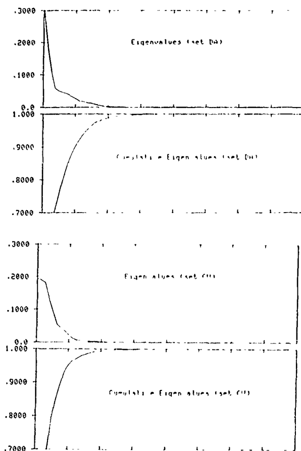
Figure 2.11 Correlation Matrix and Eigenvalue Characteristics Speech, DFT, Linear Frequency
