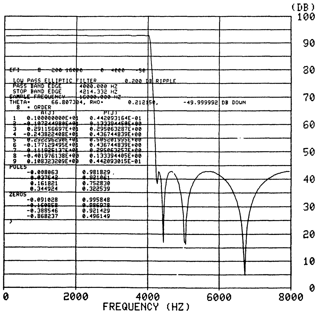
Figure 5.1 FLT Filter Characteristics
