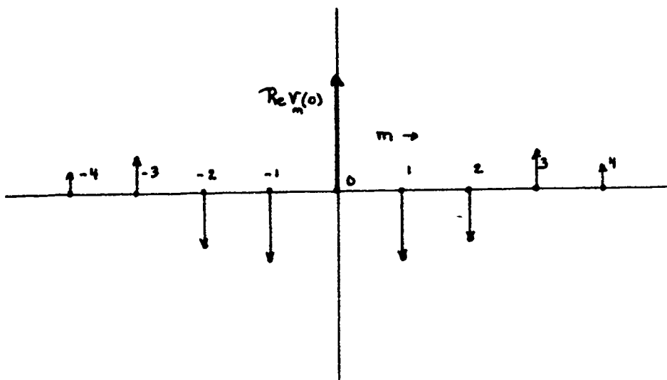
Figure 2.18 Digital Box-Car Filter (Real Components)
