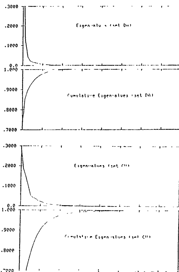
Figure 2.12 Correlation Matrix and Eigenvalue Characteristics Speech, DFT, Log Frequency
