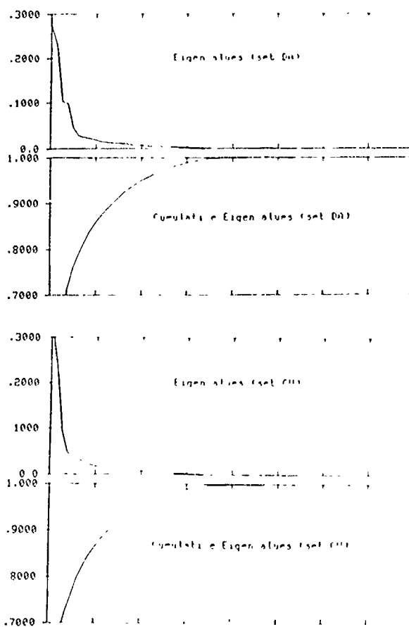
Figure 2.16 Correlation Matrix and Eigenvalue Characteristics Speech, Log Magnitude DFT, Log Frequency
