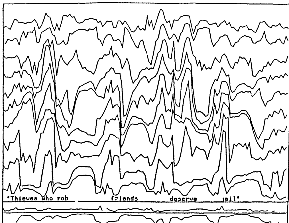
Figure 5.2 Line Spectral Pair Display
