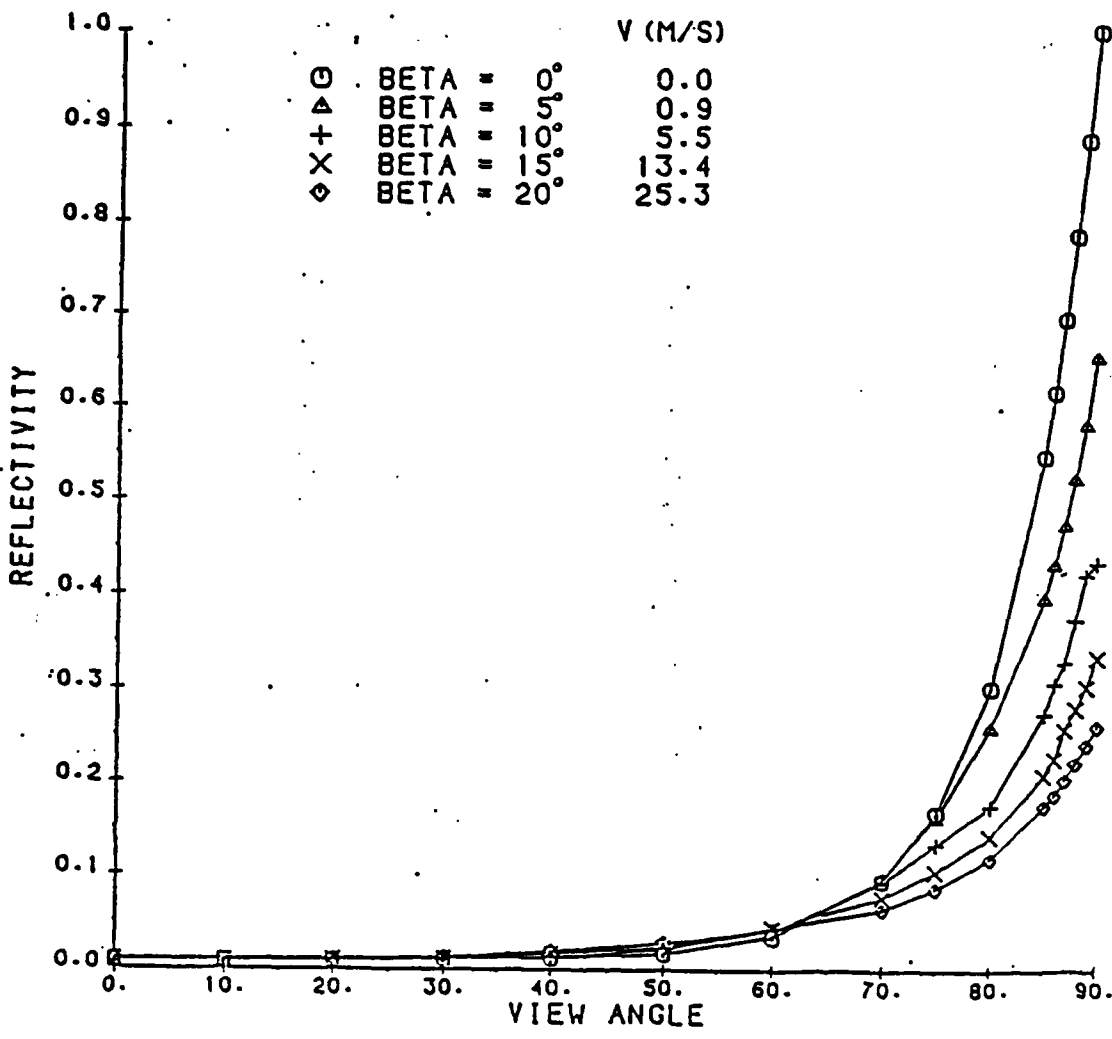
Figure 4.3: Average infrared reflectivity of the ocean surface 8–14 \mu\text{m} as a function of view angle ( \theta_V ) and wave slope angle ( B ) caused by changes in wind velocity.
