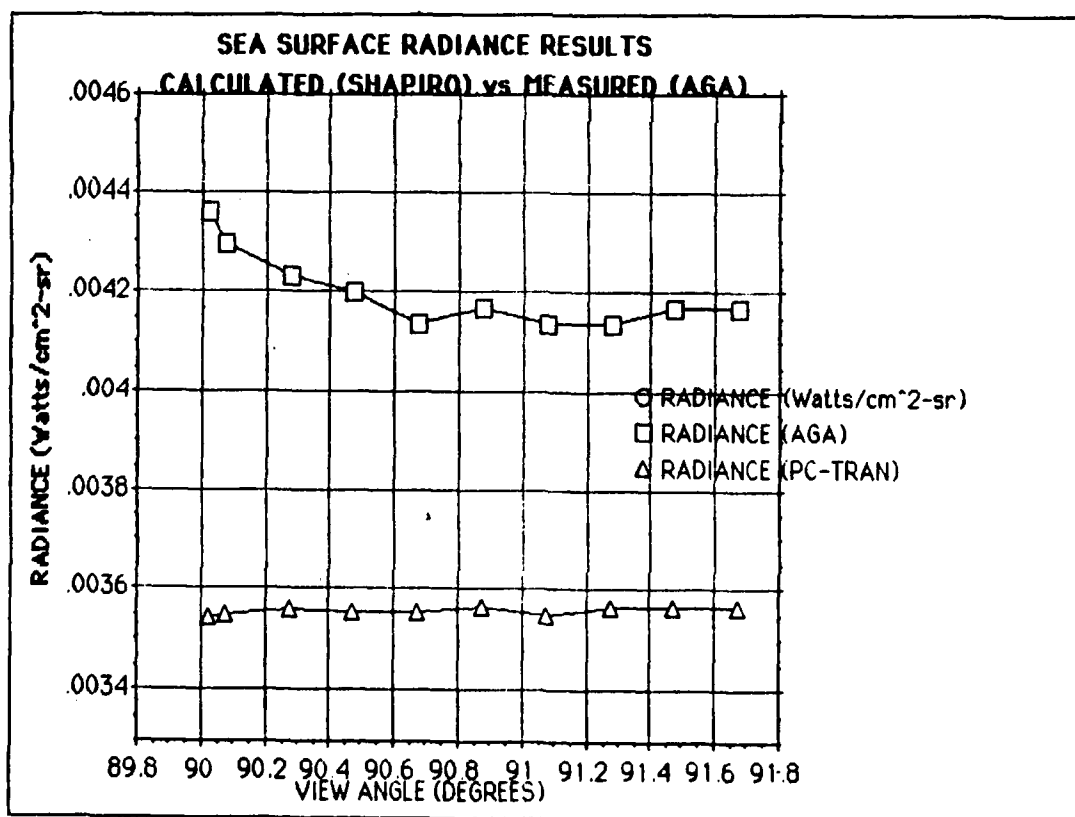
Figure 5.5: Calculated vs. measured radiance using the Shapiro algorithm and PC-TRAN at low grazing angles (May 2, 1990).
