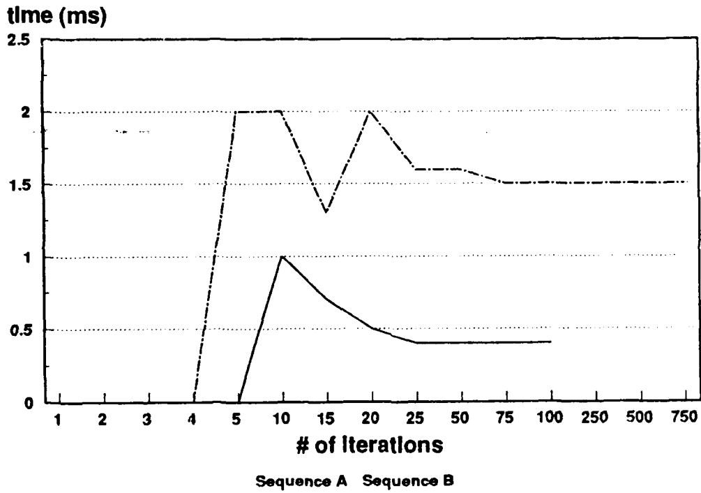
Figure 4. Insertion (75 tuples)
