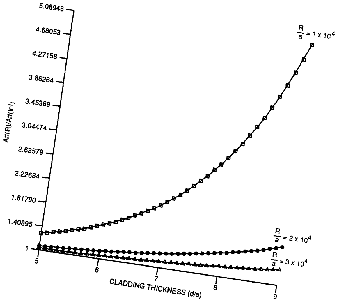
FIGURE 3. Normalized Cladding Thickness Versus Normalized Attenuation for AT&T DSF at 1.55 \mu\text{m} .
