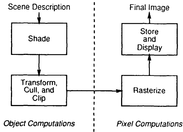
Figure 2: A typical rendering pipeline. The dotted line divides object-level and pixel-level operations.
