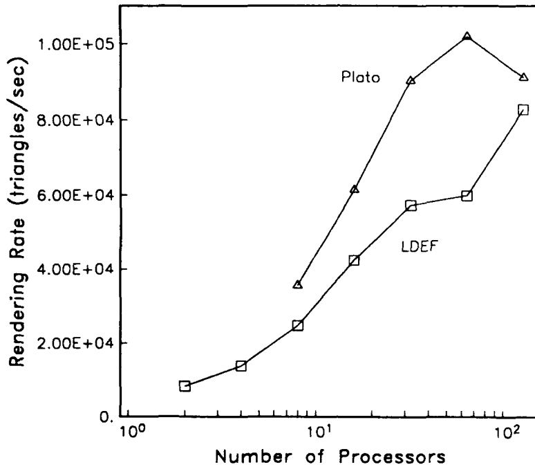
Figure 13: Rendering rates for the LDEF and Plato scenes.
