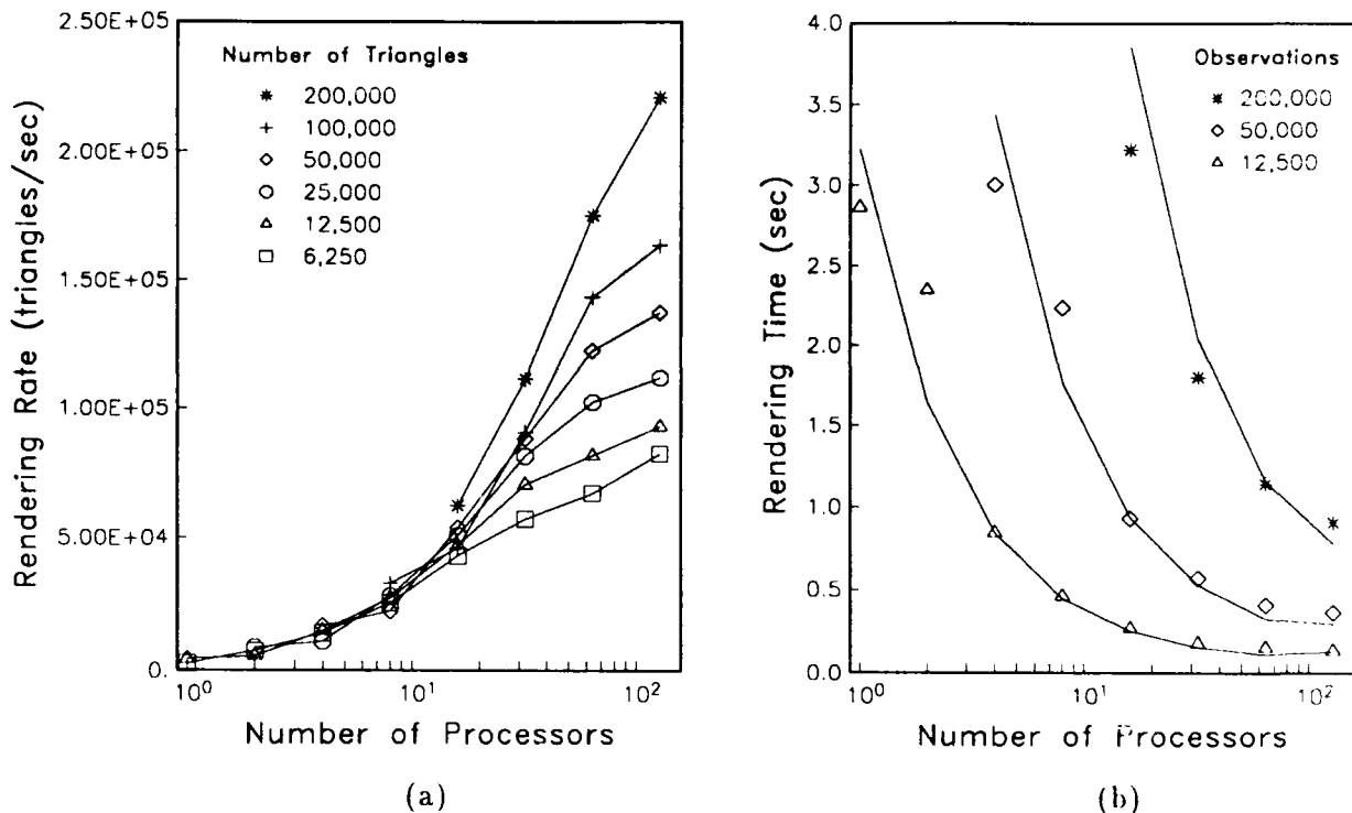
Figure 8: (a) Observed rendering rates for several random triangle scenes. (b) Observed and predicted rendering times for n = 12500, 50000, \text{ and } 200000 . Solid lines are the predicted performance.
