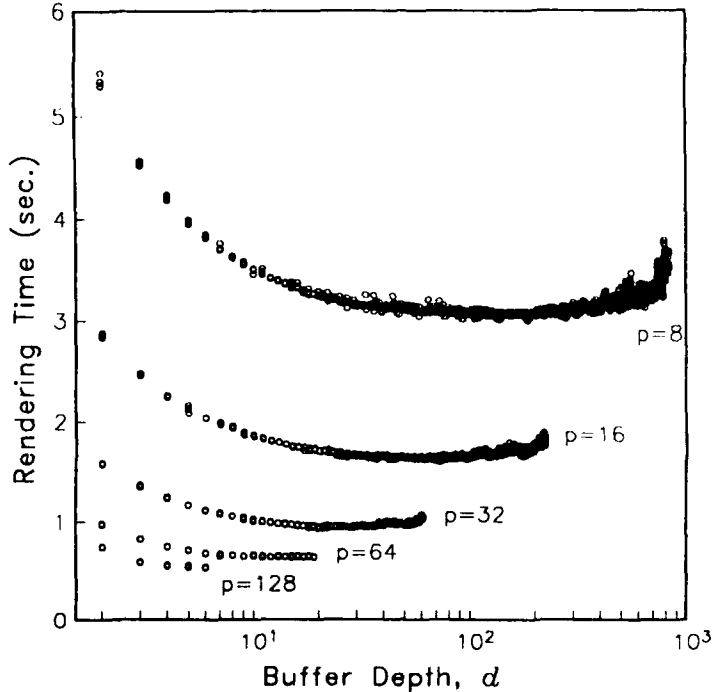
Figure 7: Execution time as a function of buffer depth for the standard test scene. d = 2, \dots, v/2 .
