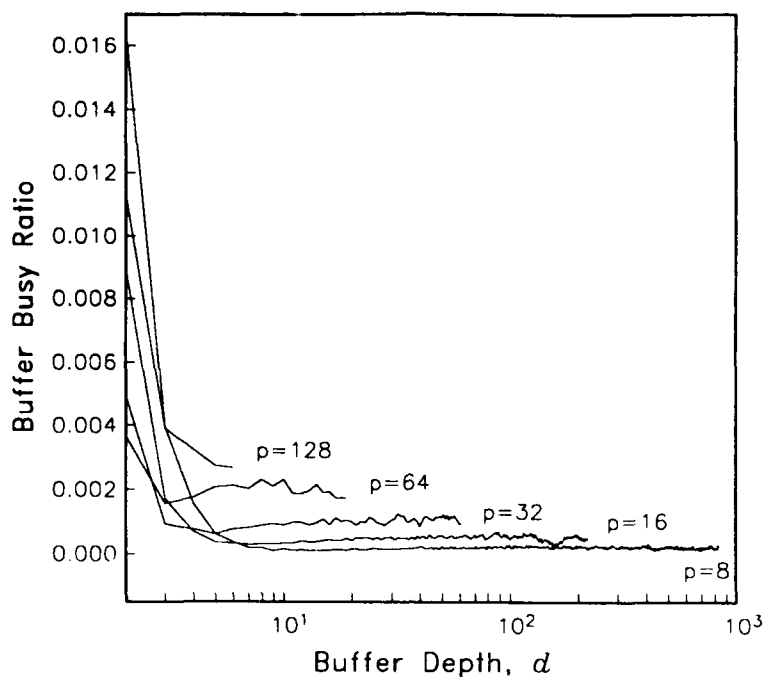
Figure 5: Buffer busy ratio vs. buffer depth.
