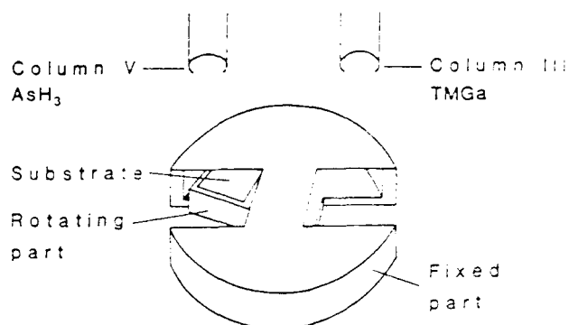
Figure 1. Schematic of the rotating susceptor for ALE.
