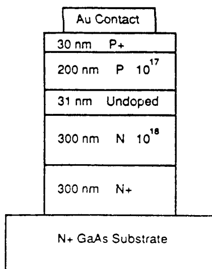
Figure 11. Cross-sections of the PiN diode
