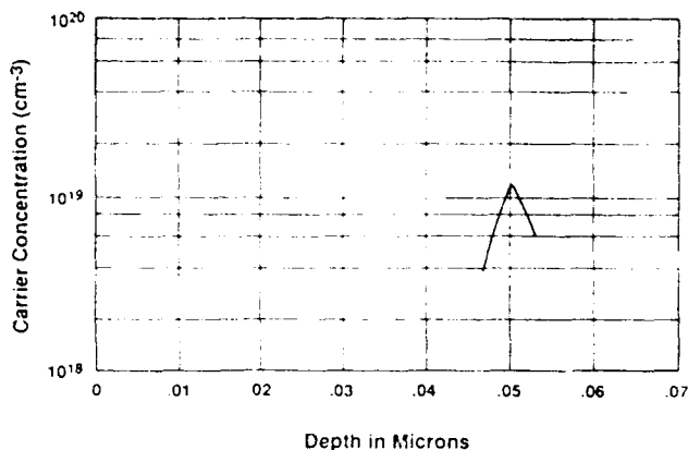
Figure 8. C-V profile of a delta-doped structure
