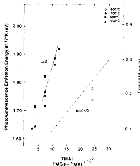
Figure 3. PL emission energy at 77^\circ\text{K} of \text{Al}_x\text{Ga}_{1-x}\text{As} and corresponding solid composition x as function of \frac{\text{TMA}}{\text{TMA}+\text{TMGa}} molar ratio in column III stream.
