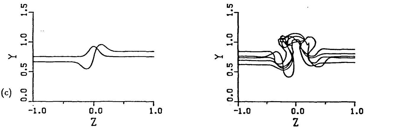
Figure 12. Evolution of multiple hairpin vortices in a uniform shear: (a) top view, (b) side view, (c) end view; all three coordinates are plotted on the same scale.
