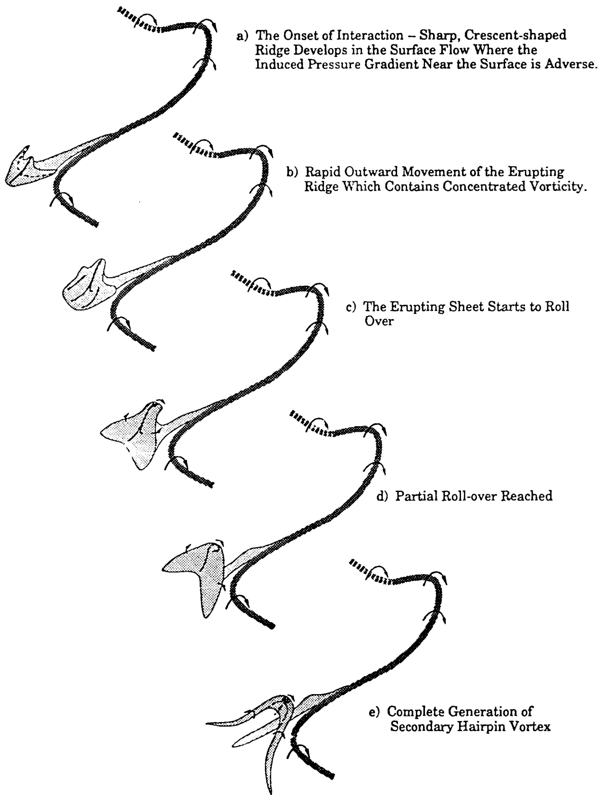
Figure 24. The generation of secondary vortex via surface interaction for an asymmetric hairpin vortex
