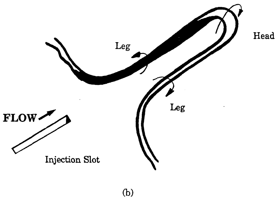
Figure 15. Illustration of experimental generation of a single hairpin vortex by surface injection using system shown in figure 14. (a) Dual-view picture of dye-marked single hairpin vortex. (b) Isometric schematic of single hairpin after generation.
