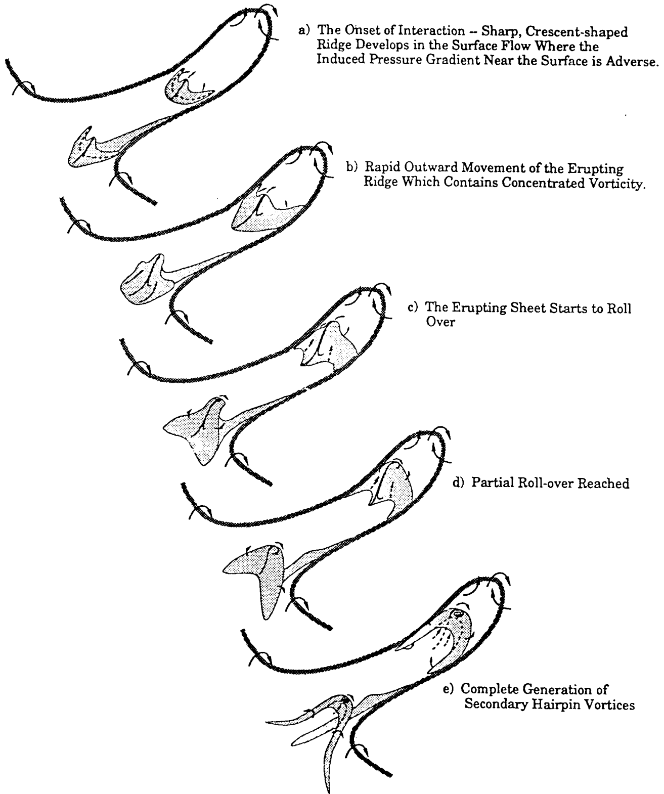
Figure 22. The generation of secondary vortices via surface interaction for a symmetric hairpin vortex
