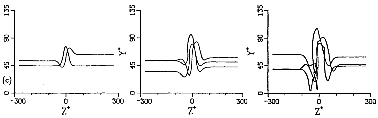
Figure 13. Evolution of three vortices in a turbulent mean profile: (a) top view, (b) side view, (c) end view; \epsilon = 0.0013 , vortices shown after 120 and 240 time steps with \Delta t = 0.016 .
