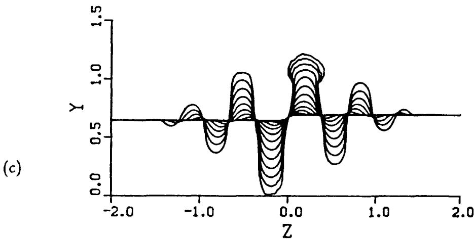
Figure 8. Evolution of a small "step" in a two-dimensional vortex convected in a uniform shear flow: (a) top view, (b) side view, (c) end view; \epsilon = 0.00267 , 440 time steps with \Delta t = 0.034 . The vortex position is plotted every 40 time steps.
