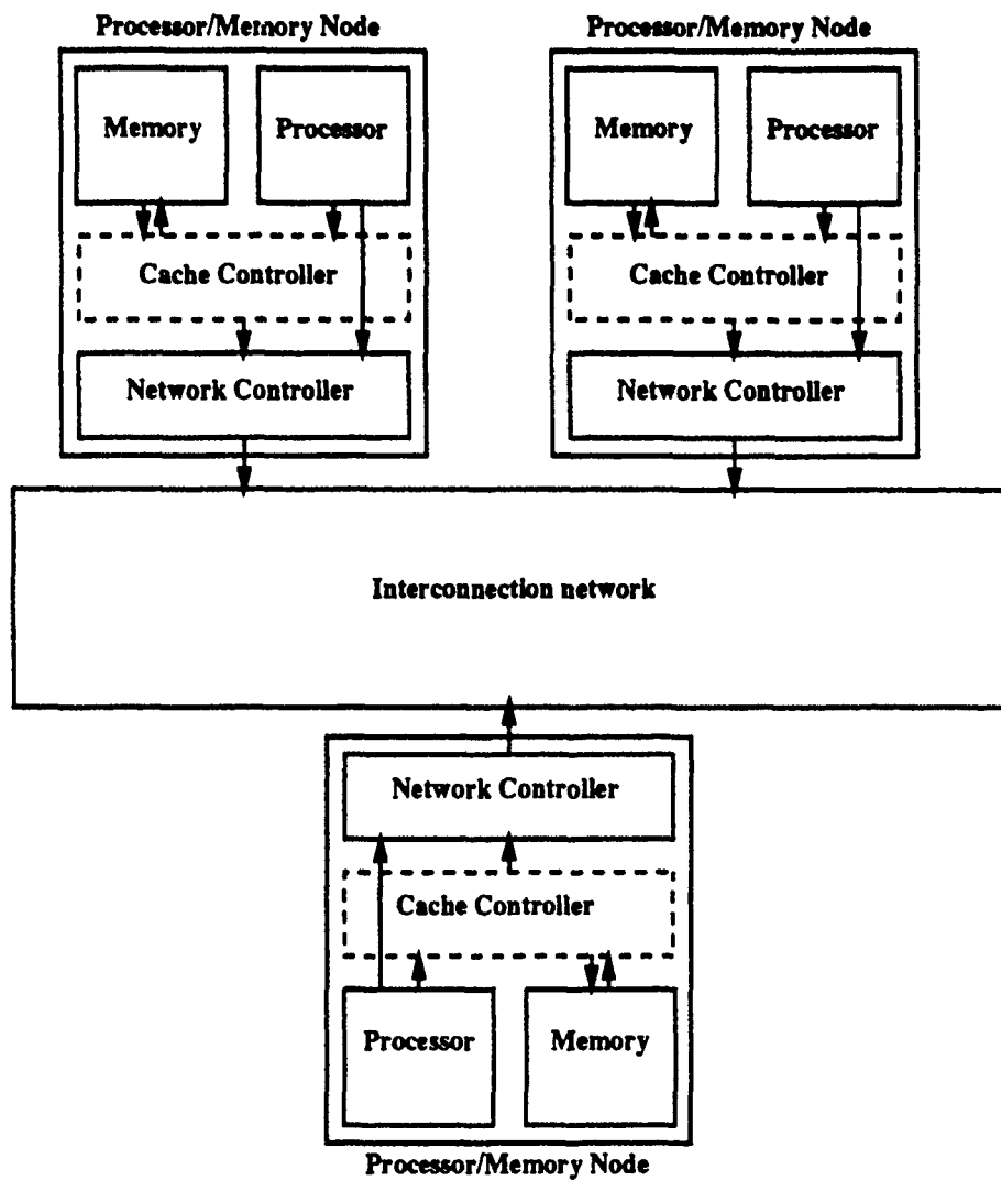
Figure 4-3: Typical network-based architecture supported by the simulator.
