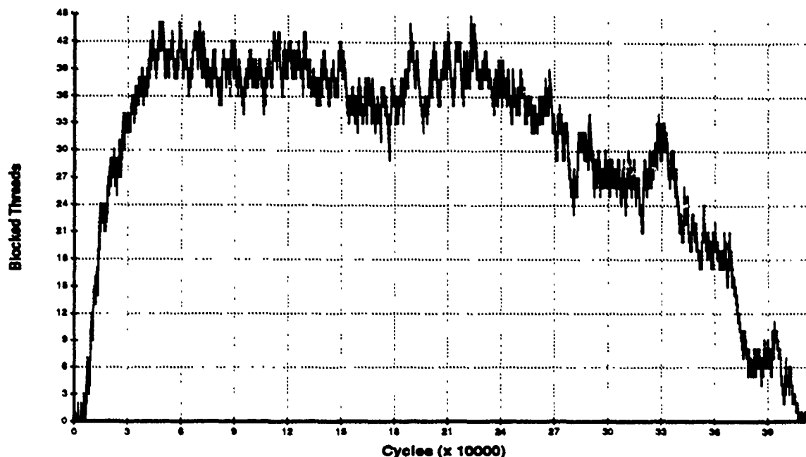
Figure 3-7: Number of threads spinning in the memory manager semaphore during execution of the 8-queens program (processors=64).
