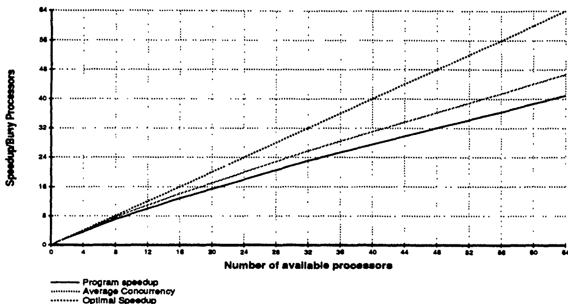
Figure 3-15: Speedup and average concurrency graphs for the 8-queens program on hypercube machines.
