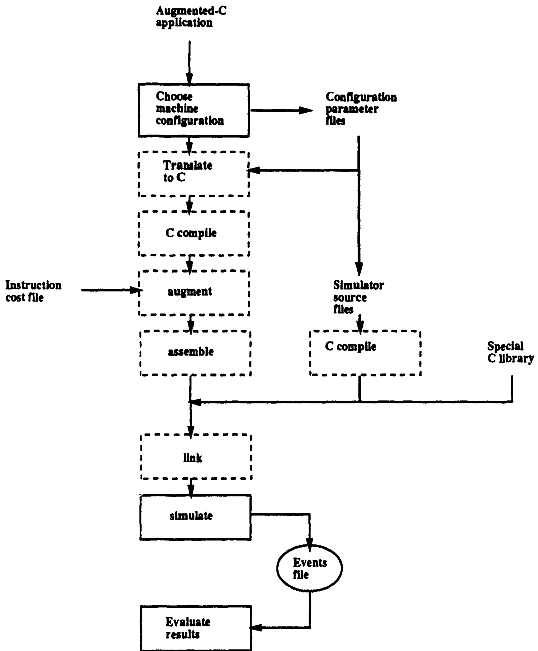
Figure 3-1: Creation, simulation and evaluation of a program using Proteus. Steps in dashed boxes are invisible to the user.
