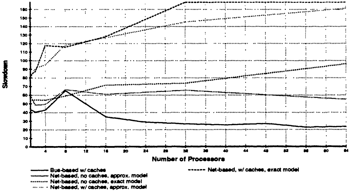
Figure 5-7: Program slowdown per processor for the 8Queens program.
