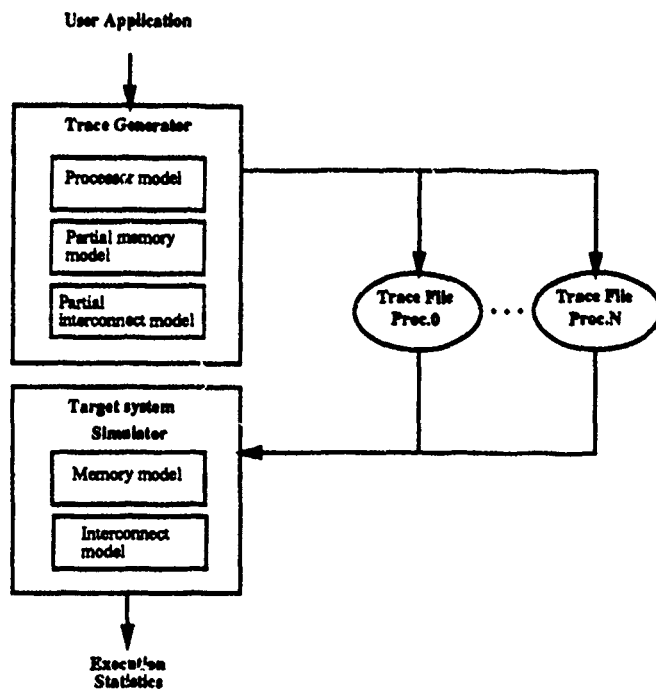
Figure 2-2: Typical structure of a multiprocessor trace-driven simulation system.
