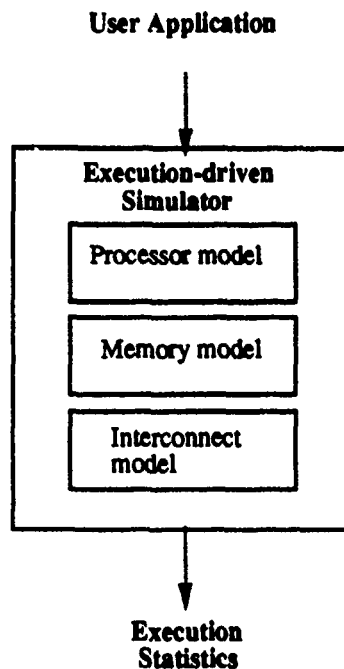
Figure 2-3: Typical structure of an execution-driven simulation system.
