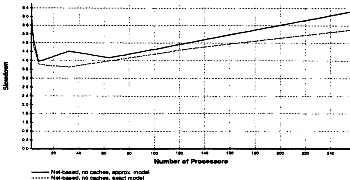
Figure 5-5: Program slowdown per processor for the Qsort program.
