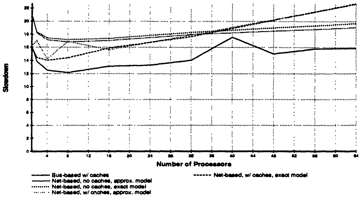
Figure 5-6: Program slowdown per processor for the Fib program.
