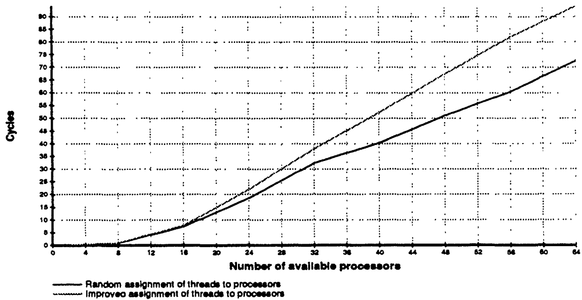
Figure 3-14: Average bus contention latencies for various machine sizes.
