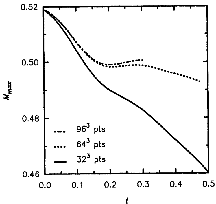
Figure 23: Time history of maximum Mach number, 3D.
