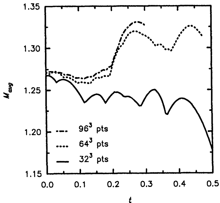
Figure 22: Time history of average Mach number, 3D.
