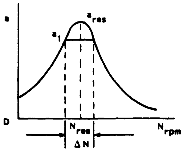
FIGURE 18 - DEFINITION OF TERMS IN EQUATION [45]
