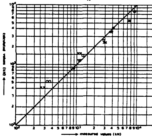
CALCULATED AND EXPERIMENTAL DATA OF F_y
