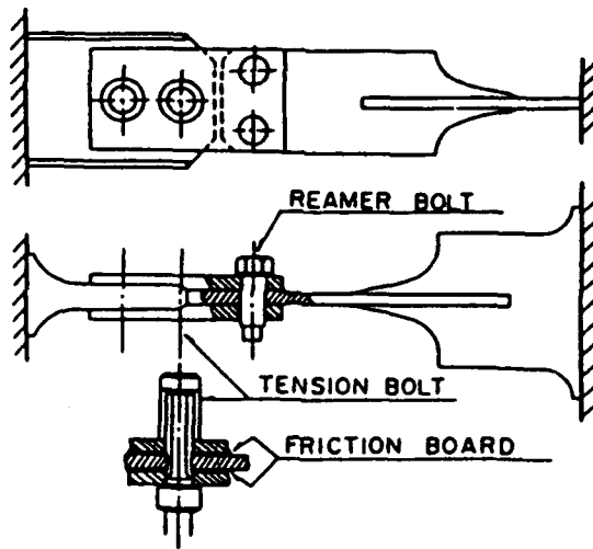
FIGURE 19 - NEW TYPE OF EXCITER (REF. 8)
