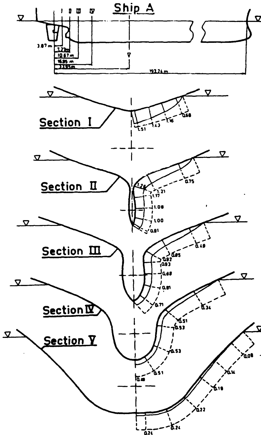
FIGURE 9 - EXAMPLE OF VARIATION OF SOLID BOUNDARY FACTORS, INCLUDING INFLUENCE FROM FREE SURFACE EFFECTS, REF. 59. DOTTED LINES REPRESENT THE VALUE S = 2.0
