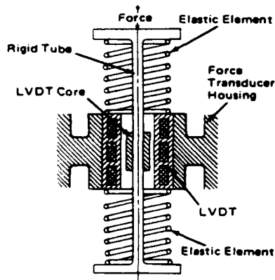
SCHEMATIC DIAGRAM GRAM RANGE FORCE TRANSDUCER
