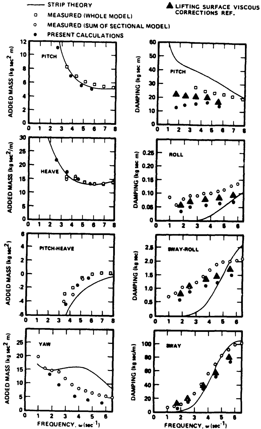
FIGURE 15 - MOTION COEFFICIENTS FOR SERIES 60, C_B = 0.70 AT Fr = 0.20 , FROM REF. 71 (CONCLUDED)
