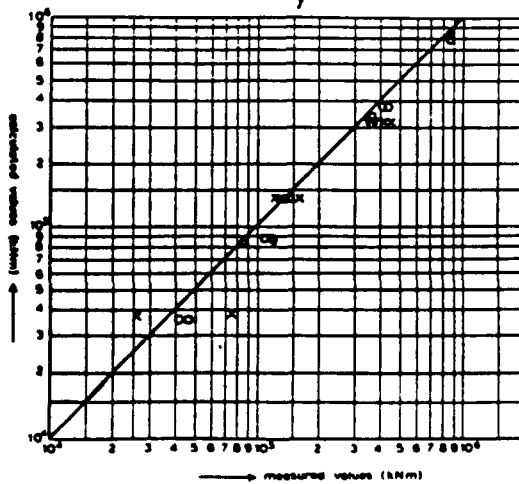
CALCULATED AND EXPERIMENTAL DATA FOR M_z
