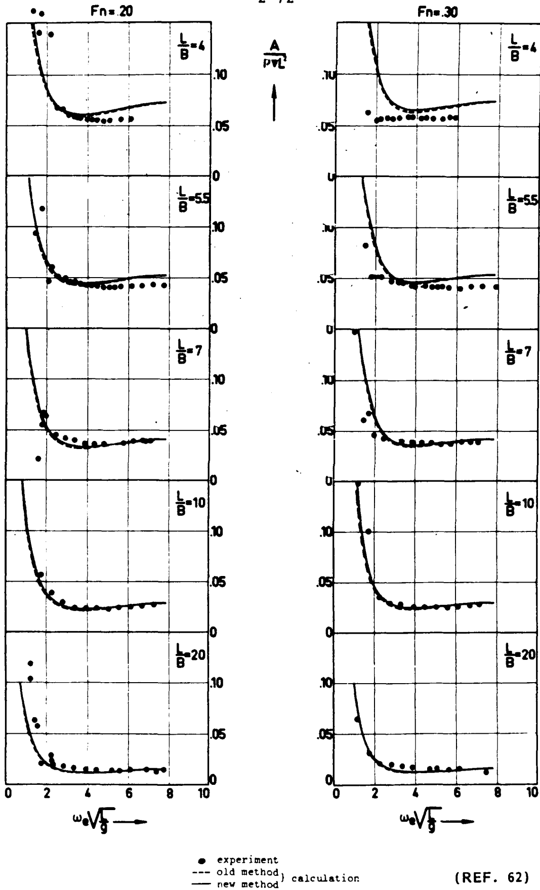
FIGURE 13 - COEFFICIENT OF ADDED MASS MOMENT OF INERTIA FOR PITCH
