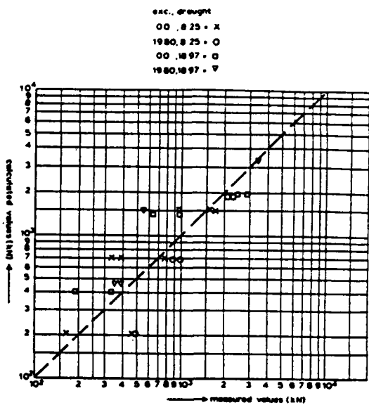
CALCULATED AND EXPERIMENTAL DATA FOR F_x
