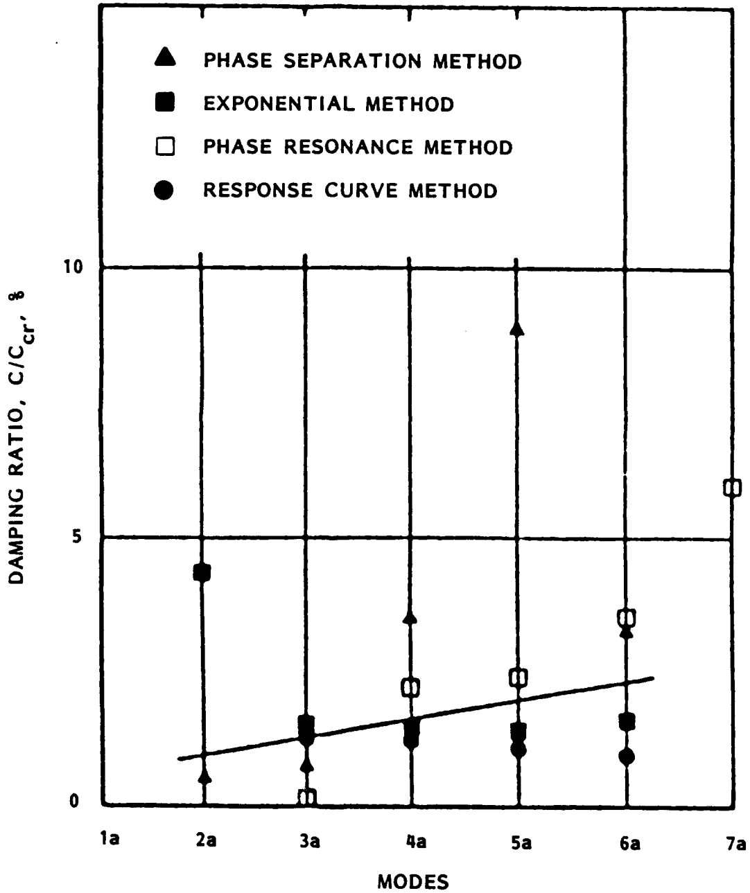
FIGURE 4 - DAMPING COEFFICIENT IDENTIFIED BY DIFFERENT ANALYSIS METHODS FOR A CAR FERRY (REF. 12)
