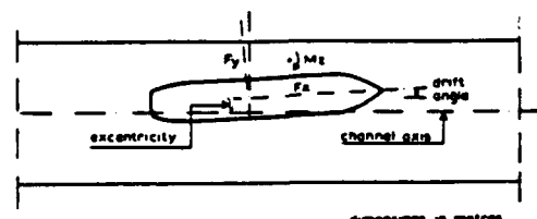
EXPERIMENTAL SET-UP AND SIGN CONVENTIONS
