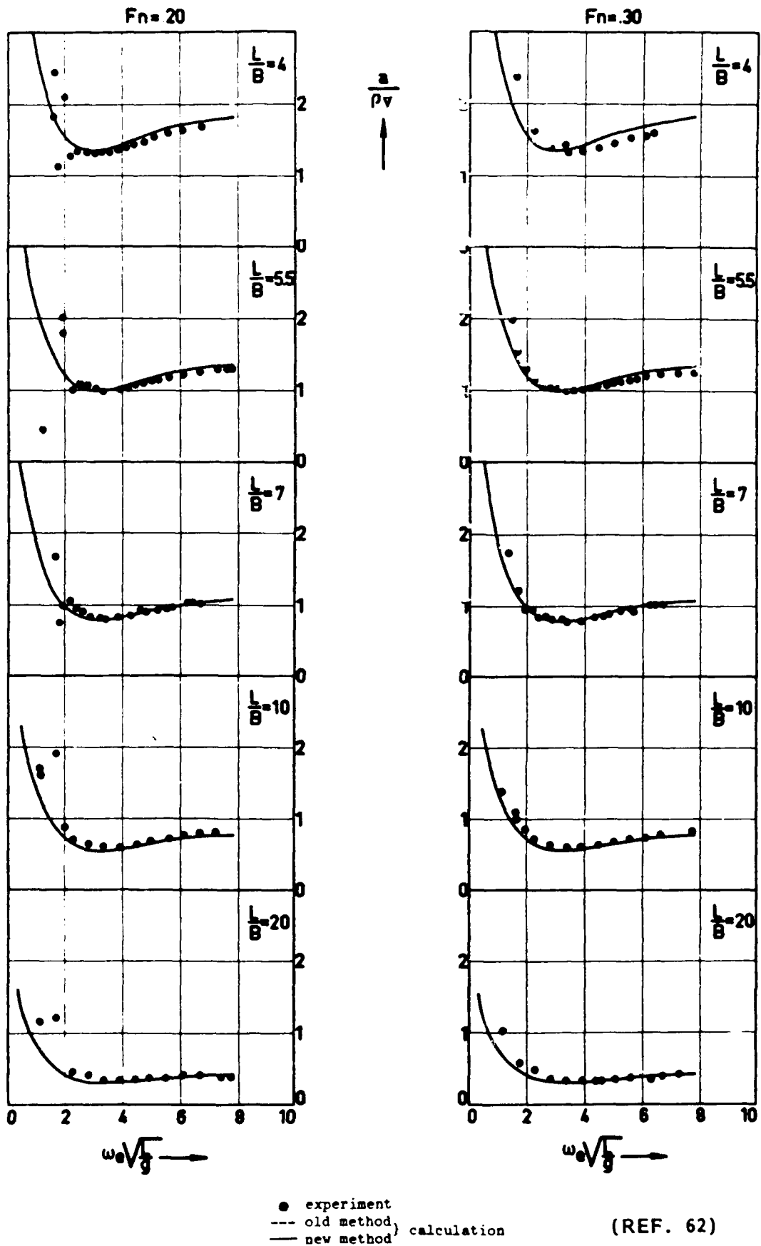
FIGURE 11 - ADDED MASS COEFFICIENT FOR HEAVE
