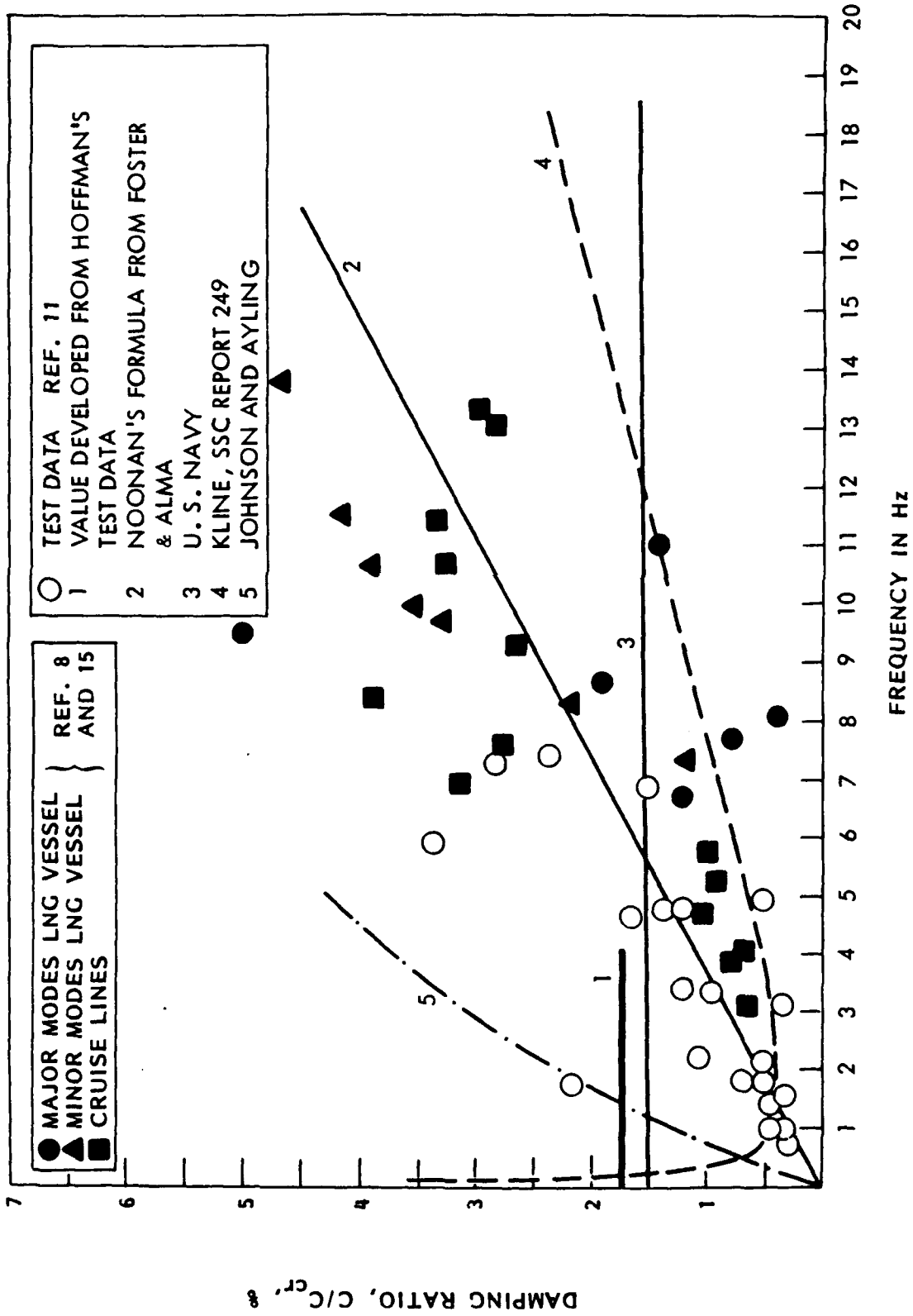
FIGURE 3 - DAMPING COEFFICIENTS DETERMINED BY VARIOUS INVESTIGATORS
