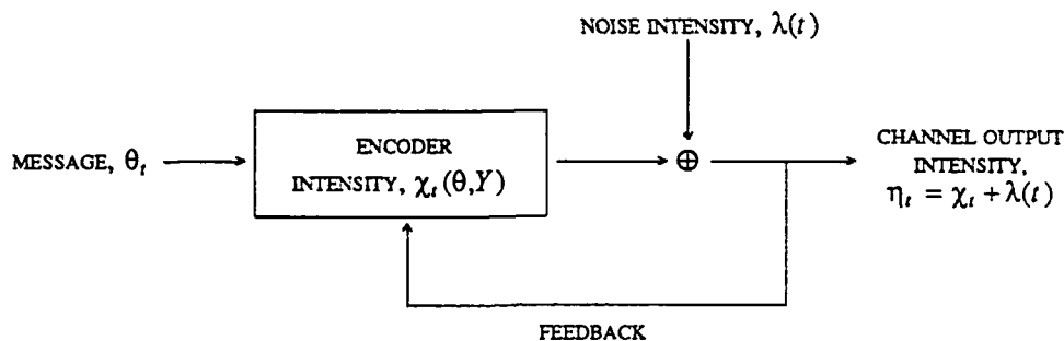
Figure 1. Poisson channel model.
