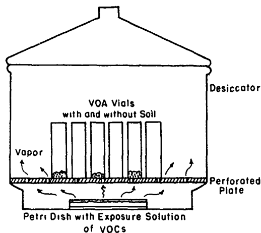
Figure 1. Vapor contamination chamber.
