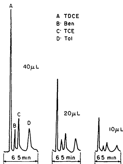
Figure 2. Chromatograms of the four volatile organic compounds tested.
