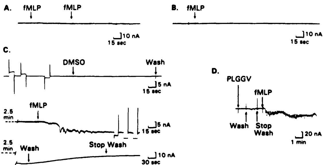
Fig.1. Acquired FPCR induced whole cell currents in Xenopus oocytes. Oocytes were injected with: (A) 50 nl of water (holding potential ( V_h ) = -75 mV). Arrows indicate the times of addition of 10^{-6} M fMLP; (B) 50 ng of poly(A) ^+ RNA from undifferentiated HL60 cells ( V_h = -56 mV). 10^{-6} M fMLP was added at arrow; (C) 50 ng of poly(A) ^+ RNA from differentiated HL60 cells ( V_h = -65 mV). DMSO 0.01% and 10^{-6} M fMLP were added where indicated. Current responses to voltage steps used to measure I - V relationships before and after addition of fMLP are shown; (D) 50 ng of fraction 12 (see fig.3) poly(A) ^+ RNA from differentiated HL60 cells ( V_h = -60 mV). Phe-Leu-Glu-Glu-Val (PLGGV) and fMLP were added at 3 \times 10^{-7} M. Downward deflection indicates inward current.
