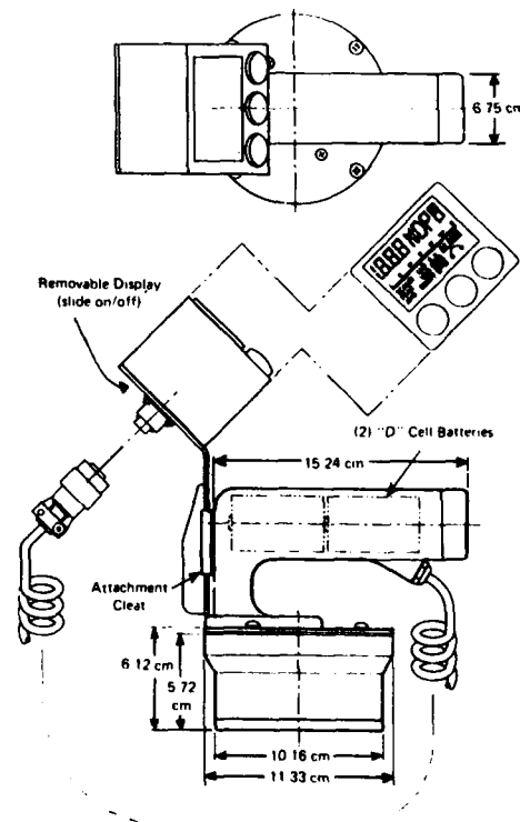
Fig. 1. Alpha radiac with removable stand-alone display unit.
