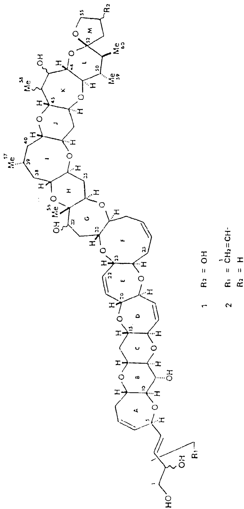
STRUCTURES OF CTX ISOLATED FROM MORAY EEL (1) AND ITS CONGENER FROM THE CAUSATIVE DINOFLAGELLATE Gambierdiscus toxicus (2)
