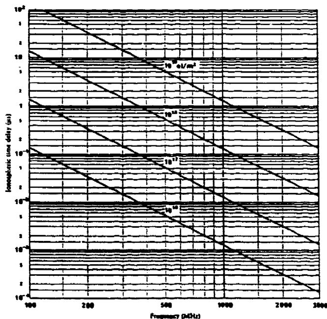
Figure 3.3.1.1 Ionospheric time delay versus frequency for various values of electron content
