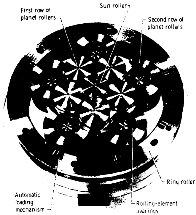
(a) Experimental traction drive transmission.
