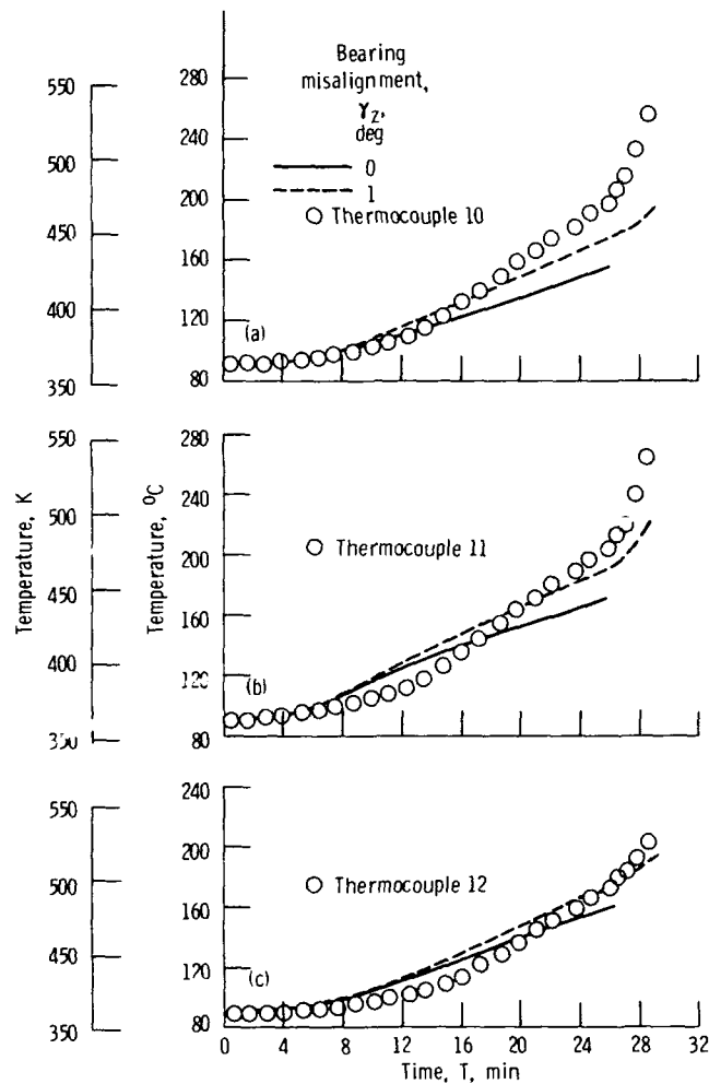
Figure 15. - Computer simulation of loss of lubricant in the OH-58 transmission. Predicted transient temperatures compared to experimental data, output shaft area. Drain plug removed at T = 0 ; oil pressure to zero at t = 1.5 minutes.
