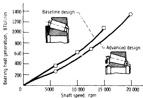
Figure 10. - Advanced design for tapered roller bearings provides cooler operation at high speed.
