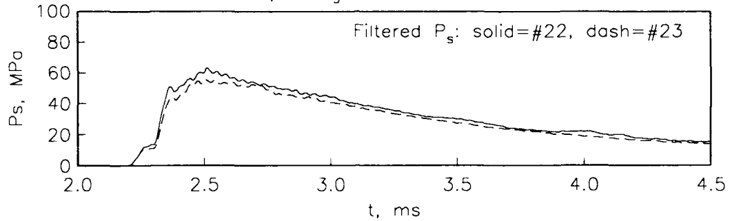
T4 shot 1007, Straight Combustor 100mm x 47mm
