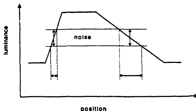
Fig. 3 Noise in the system with identical amplitude (e.g. receptor-noise; vertical arrows) leads to a larger positional error (horizontal arrows) in the determination of horizontal position of shallow luminance gradients (right side) than of steeper ones (left side).
