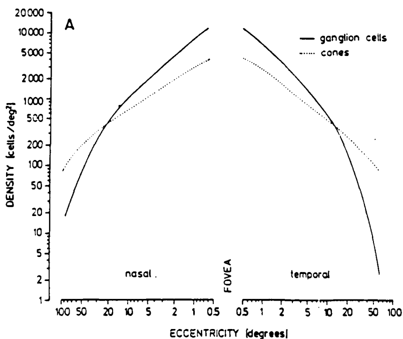
Fig. 8 Cone and ganglion cell density at different retinal positions (modified from Wässle et al., 1990).
