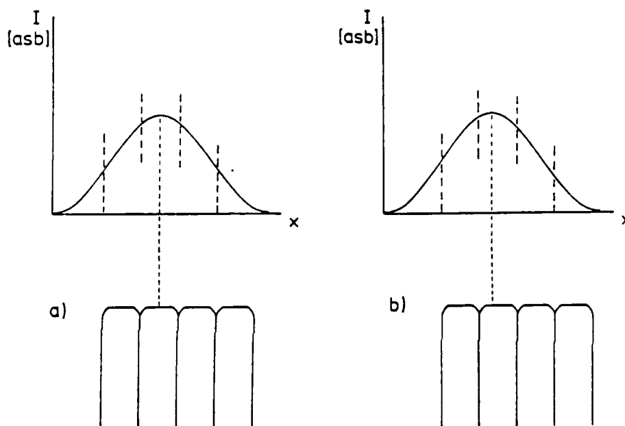
Fig.2 The optics of the eye transforms even the smallest point into a luminance distribution on the retina with a half-width of at least 20 arcsec, as indicated in the upper part. Thus, every retinal image will extend over several photoreceptors (receptors are schematized in the lower part). In (a), a bright point is located exactly on the middle of the photoreceptor and all surrounding photoreceptors are equally stimulated. If the point is moved even by a fraction of a receptor diameter, the neighbor on this side will be more strongly stimulated than the one on the opposite side (b). The ensemble of neighboring receptors can provide positional information beyond the receptor diameter.
