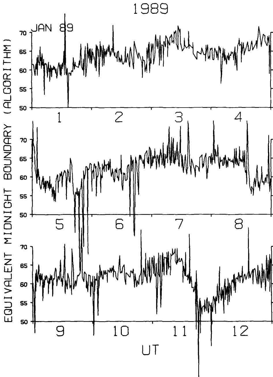
Figure 1. Midnight equivalent auroral boundary created by using all boundary crossings and the regression coefficients in Table 3
