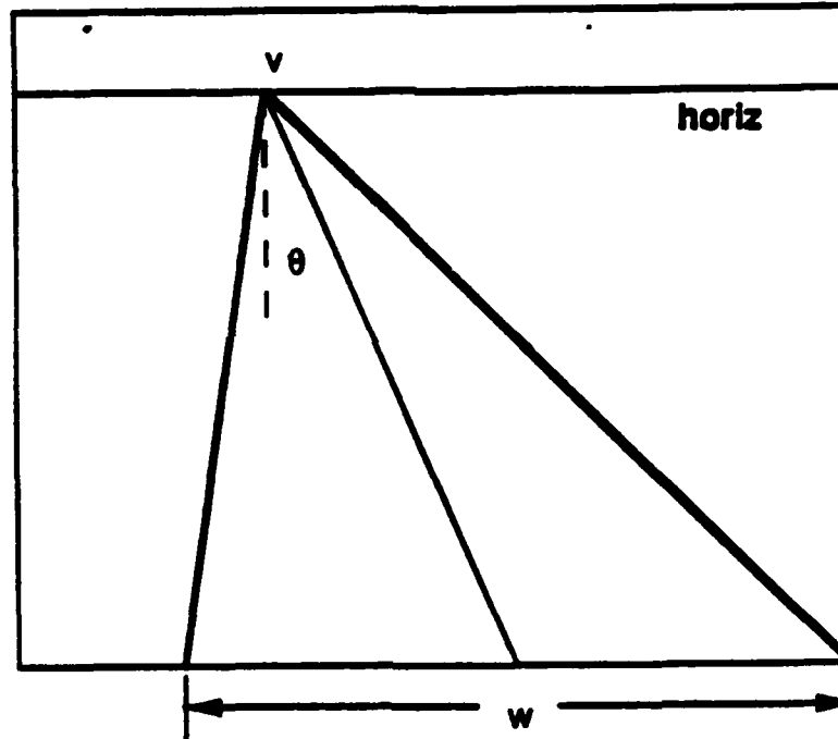
Figure 4.3: Road Hough
