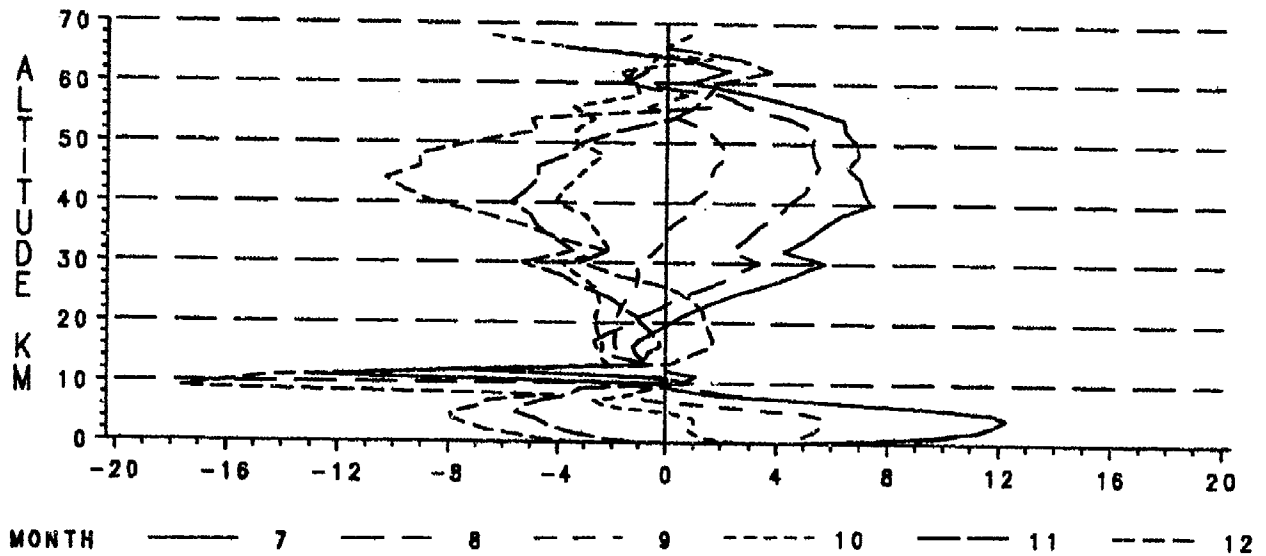
Figure F-16 Delta Temperature (K), July-December.
