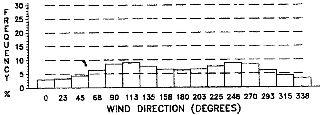
Figure E-4. Wind Direction Frequency, January, 30 KM.
