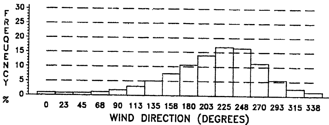
Figure E-2. Wind Direction Frequency, January, 12 KM.
