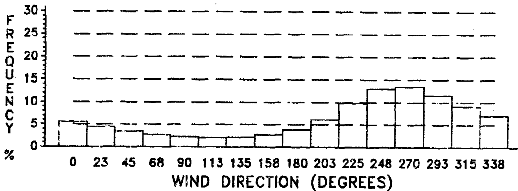
Figure E-9. Wind Direction Frequency, July, 4 KM.
