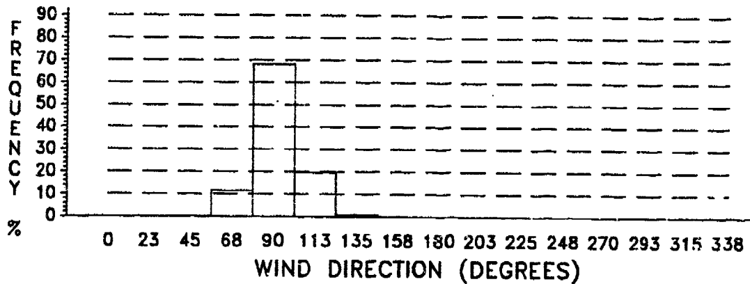
Figure E-12. Wind Direction Frequency, July, 30 KM.
