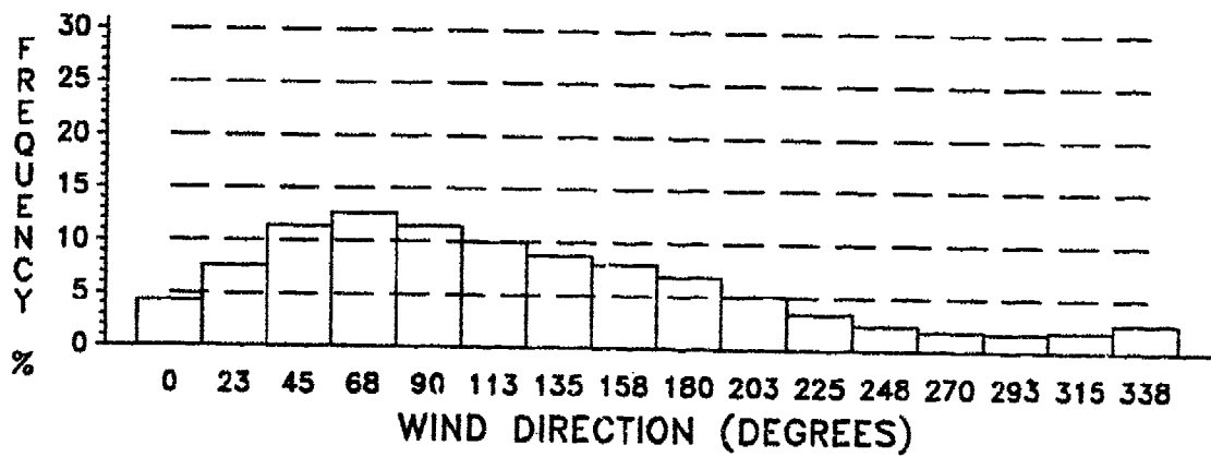
Figure E-11. Wind Direction Frequency, July, 20 KM.
