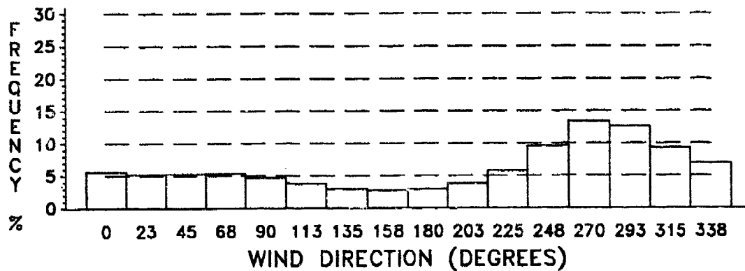
Figure E-6. Wind Direction Frequency, January, 50 KM.
