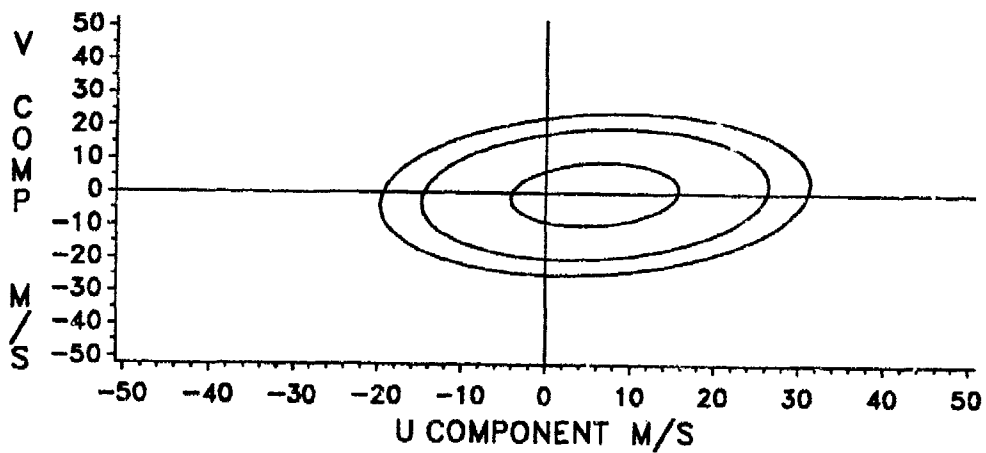
Figure E-41. Wind Probability Ellipses, July, 4 KM.
