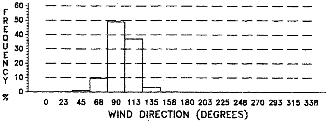
Figure E-14. Wind Direction Frequency, July, 50 KM.
