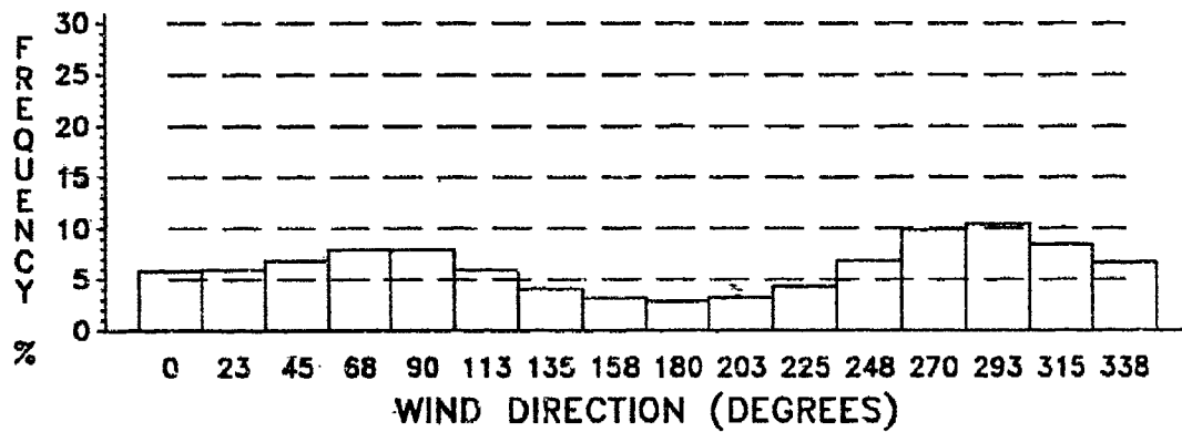
Figure E-5. Wind Direction Frequency, January, 40 KM.
