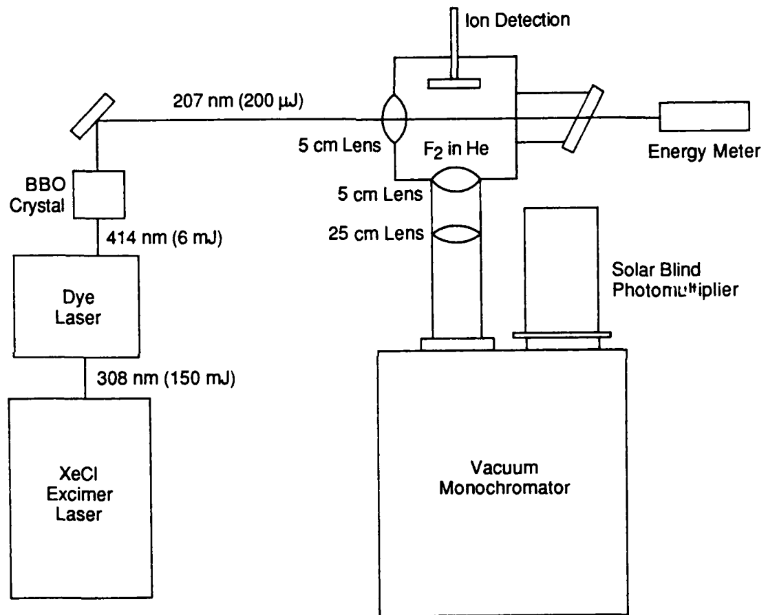
Figure 2. Experimental schematic for F 2 detection.
