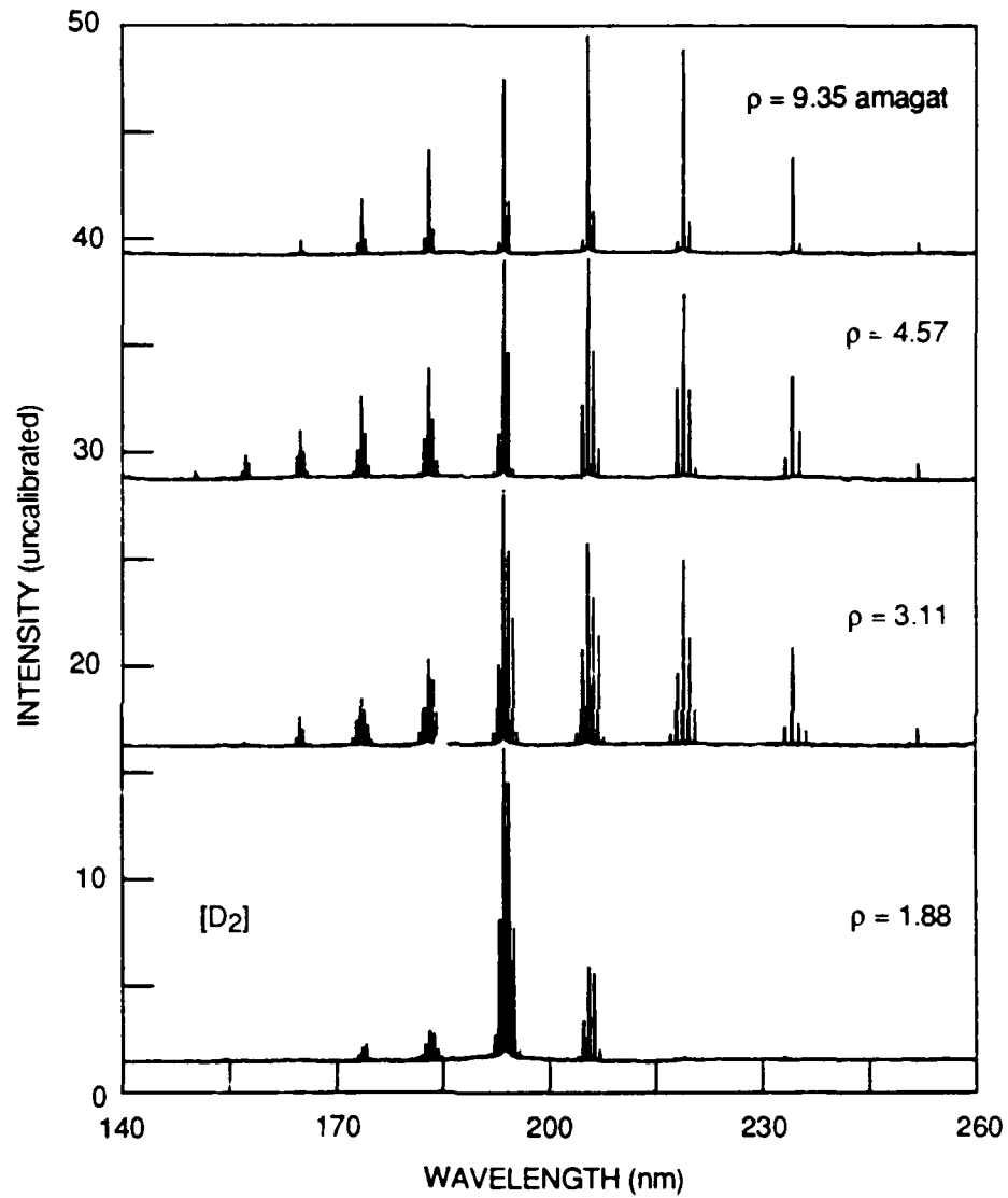
Figure 14. Raman orders in D_2 as a function of density at 77 K.
