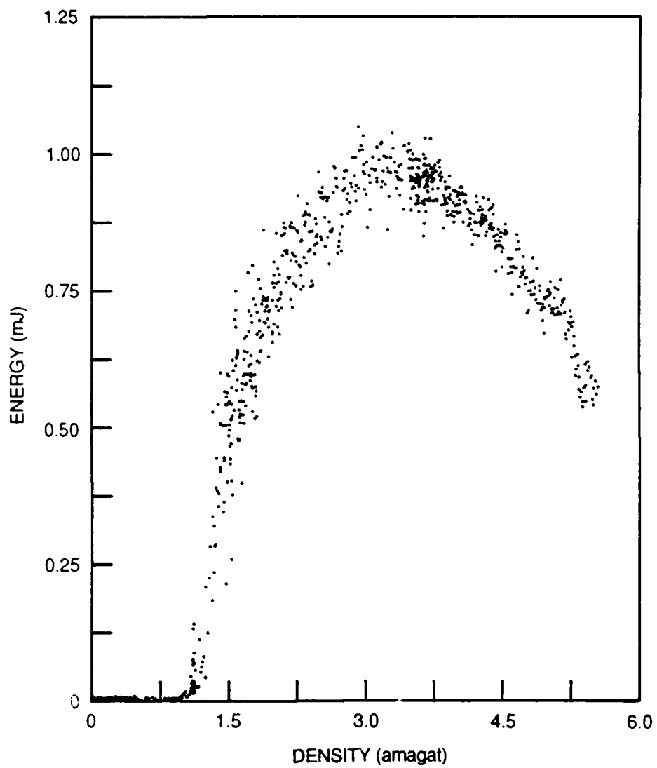
Figure 15. Density dependence of the second anti-Stokes radiation in HD.
