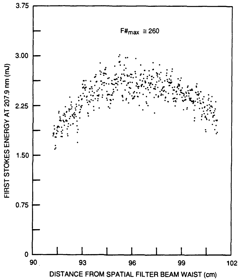
Figure 10. Dependence of first Stokes energy on lens position.
