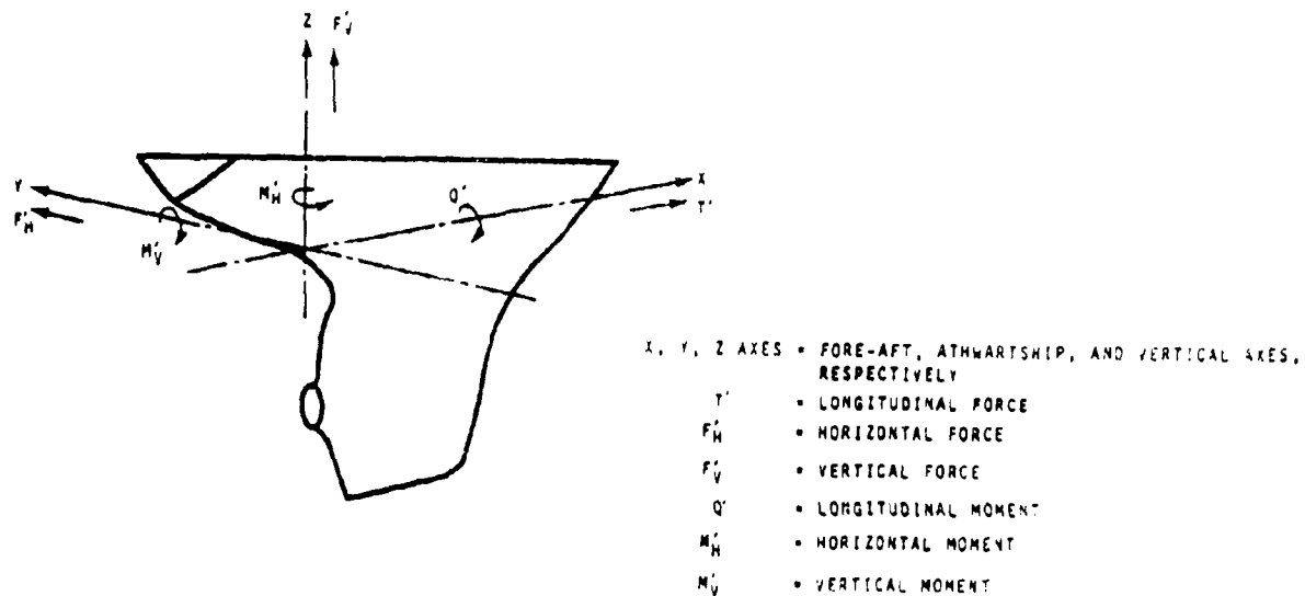
Figure 1-4 Description of Hull Pressure Forces and Moments
