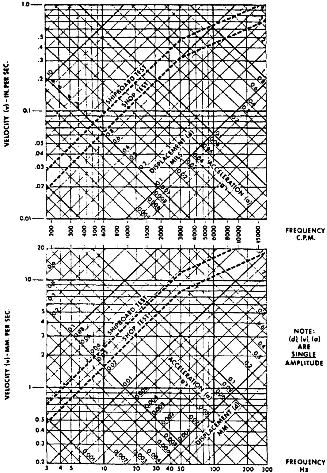
Figure 2-8 Main Propulsion Units - Shaft Vibration Limits
