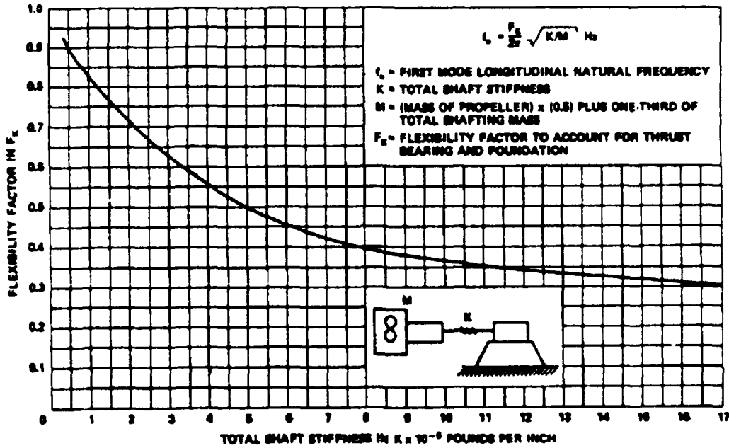
Figure 20 Preliminary Method for Determining First-Mode Longitudinal Frequency
