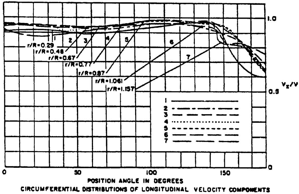
Figure 3-4 Afterbody Configuration and Wake Characteristics of an Open-Stern Single-Screw Ship
