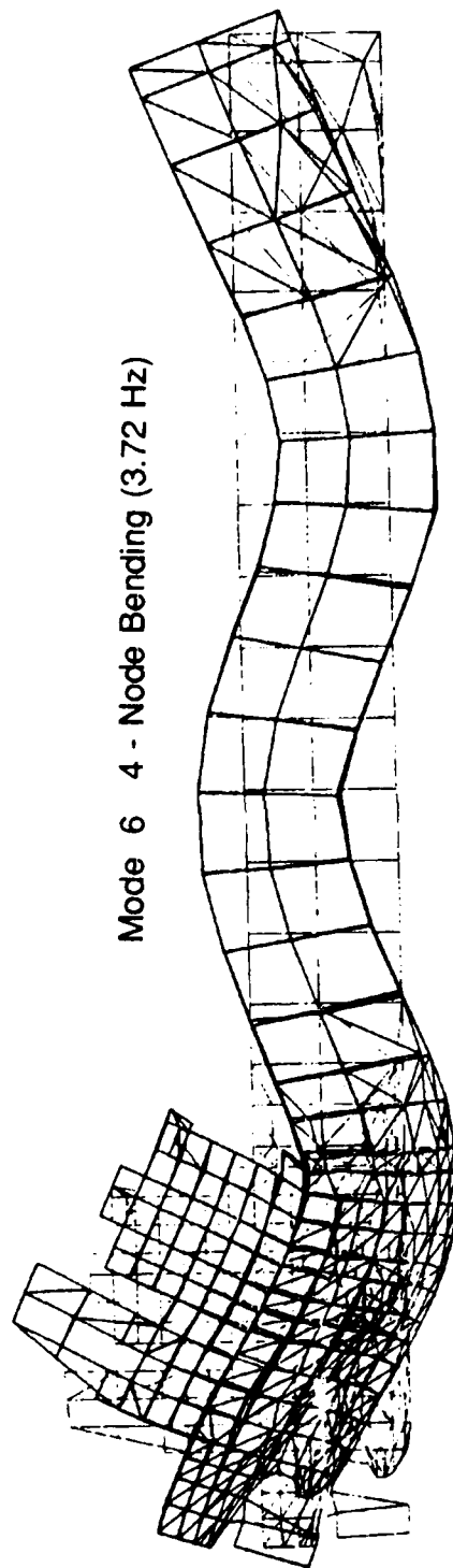
Figure 4-7 Eigenmodes in Full Load Condition
