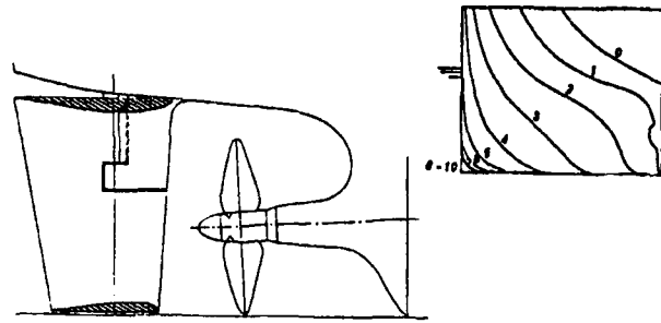
MODEL 4147 - Conventional Stern
