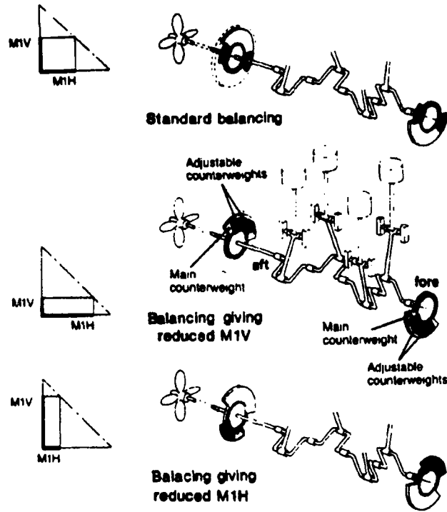
Figure 5-3 Balancing of First Order Moments [5-5]
