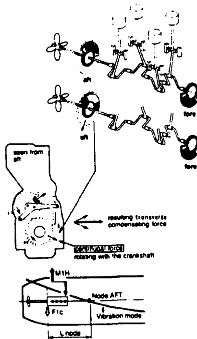
Figure 5-4 Additional Balancing of First Horizontal Moments [5-5]
