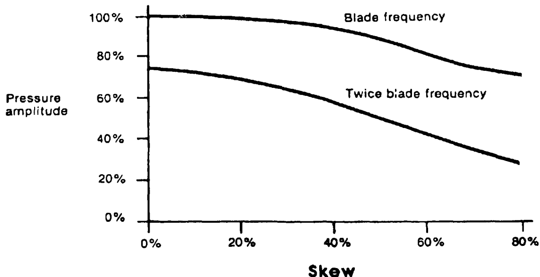
Figure 3-35 Effect of Blade Skew on Hull Pressure
