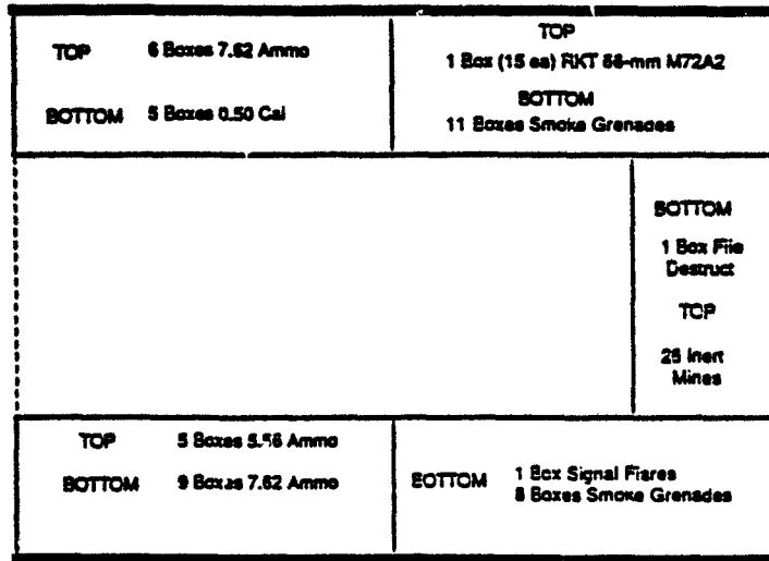
Figure 11. Ammunition in the Acceptor Container, Test 10.
