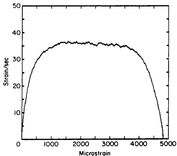
b. Computed strain rate from records in Figure 19a.
