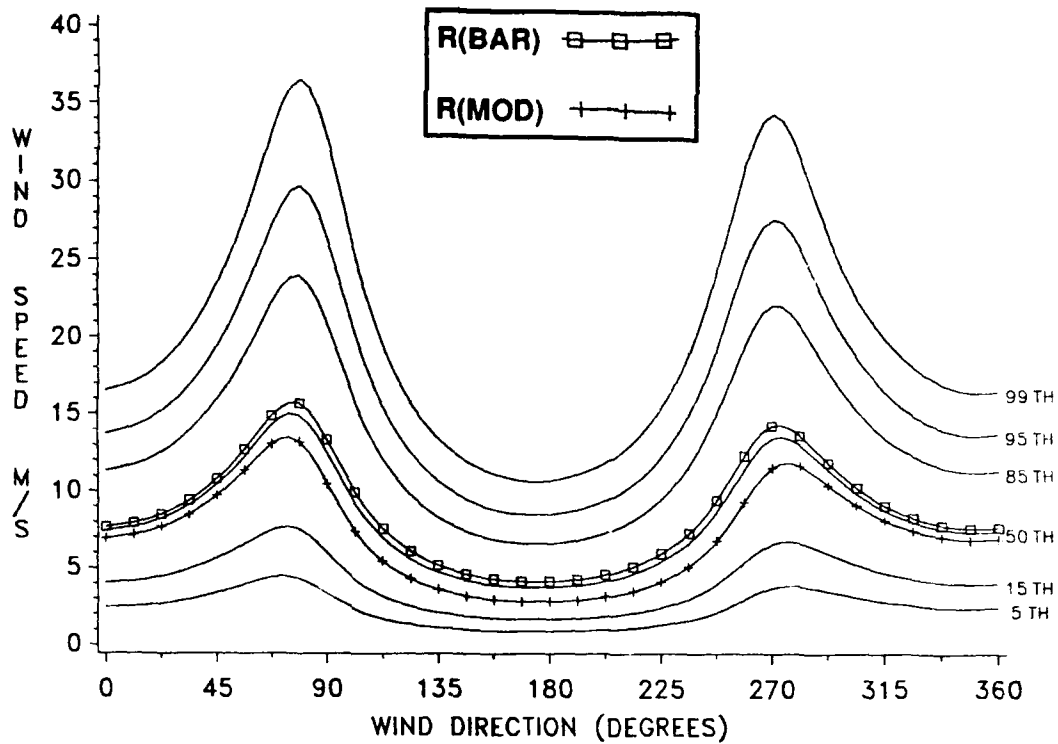
Figure E-61. Conditional Wind Speed Given Direction, January, 24 KM.
