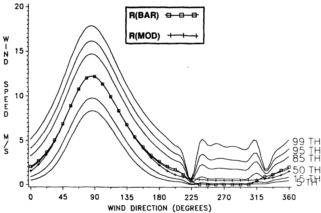
Figure E-70. Conditional Wind Speed Given Direction, July, 24 KM.
