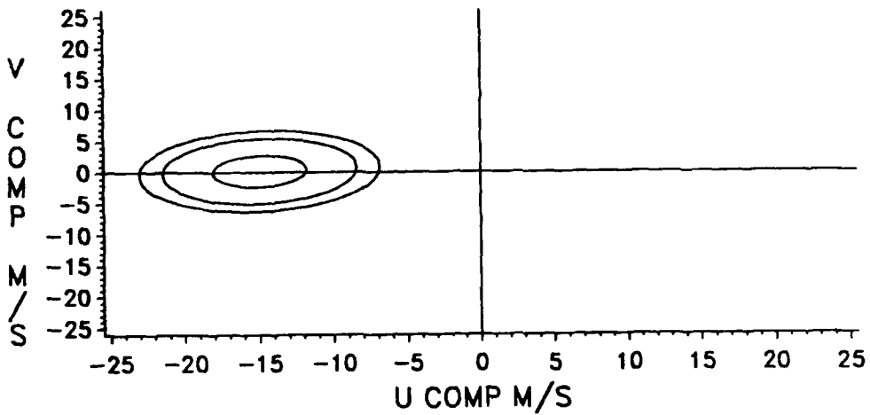
Figure E-53. Wind Probability Ellipses, July, 28 KM.
