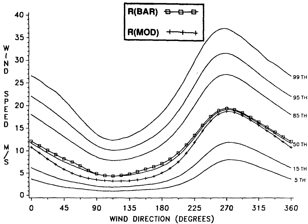
Figure E-59. Conditional Wind Speed Given Direction, January, 16 KM.
