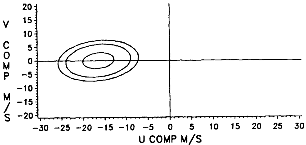
Figure E-54. Wind Probability Ellipses, July, 30 KM.
