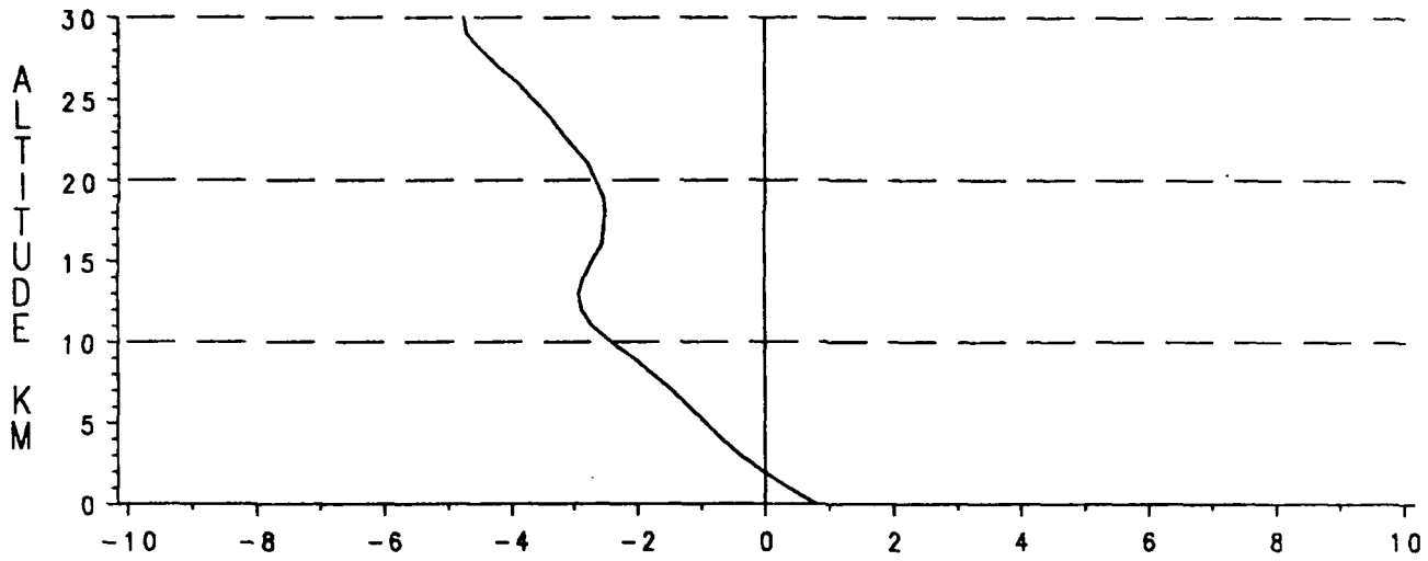
Figure F-1. Delta Percent Relative to Annual Pressure, January.
