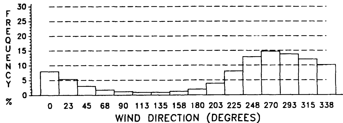
Figure E-3. Wind Direction Frequency, January, 8 KM.
