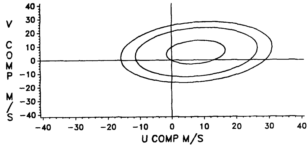
Figure E-48. Wind Probability Ellipses, July, 8 KM.
