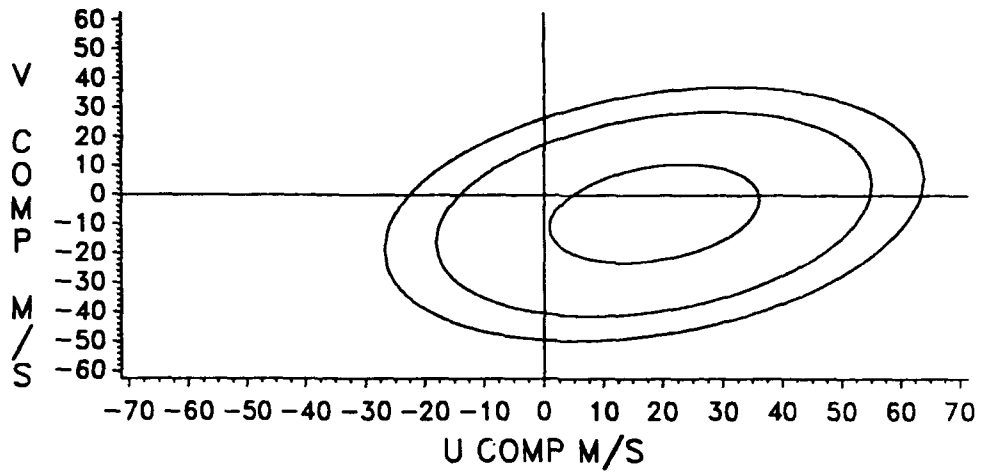
Figure E-40. Wind Probability Ellipses, January, 12 KM.
