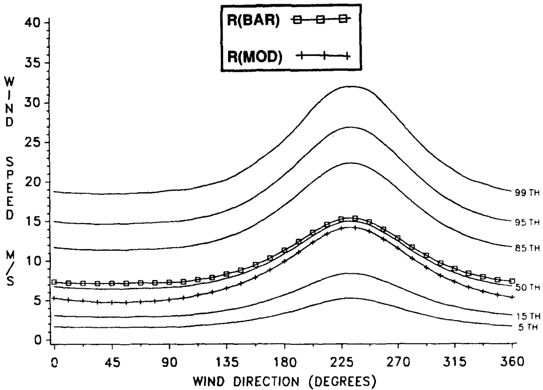
Figure E-66. Conditional Wind Speed Given Direction, July, 8 KM.
