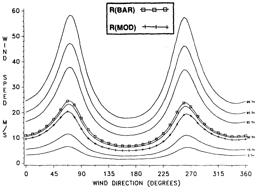
Figure E-62. Conditional Wind Speed Given Direction, January, 28 KM.
