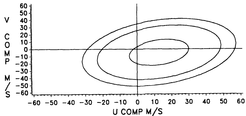
Figure E-39. Wind Probability Ellipses, January, 8 KM.
