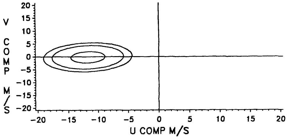
Figure E-52. Wind Probability Ellipses, July, 24 KM.
