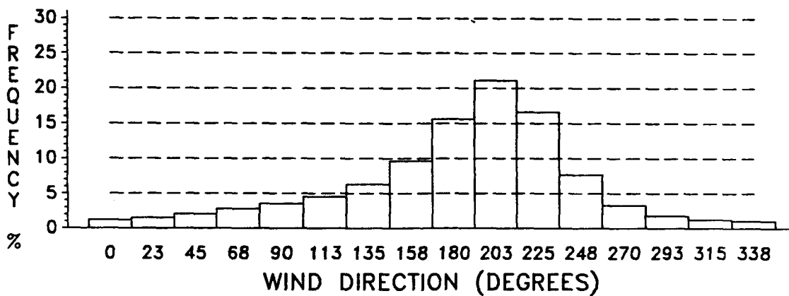
Figure E-11. Wind Direction Frequency, July, 4 KM.
