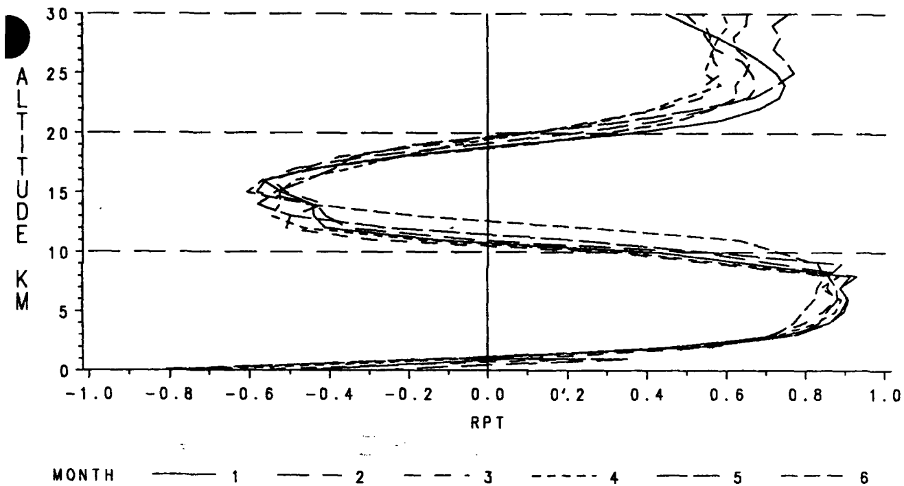
Figure F-29. Correlation Coefficients for Pressure & Temperature, January-June.
