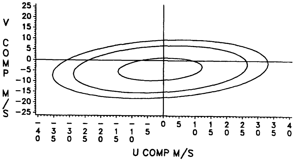
Figure E-43. Wind Probability Ellipses, January, 24 KM.
