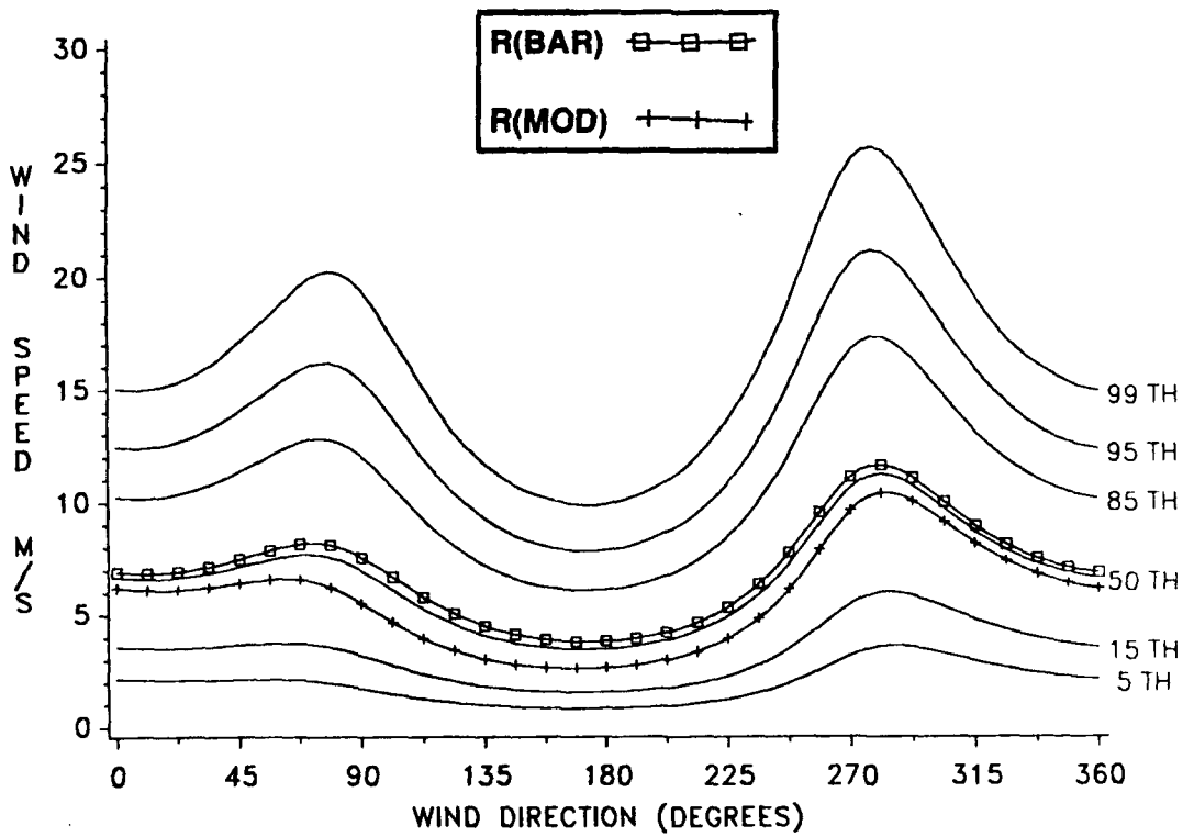
Figure E-60. Conditional Wind Speed Given Direction, January, 20 KM.
