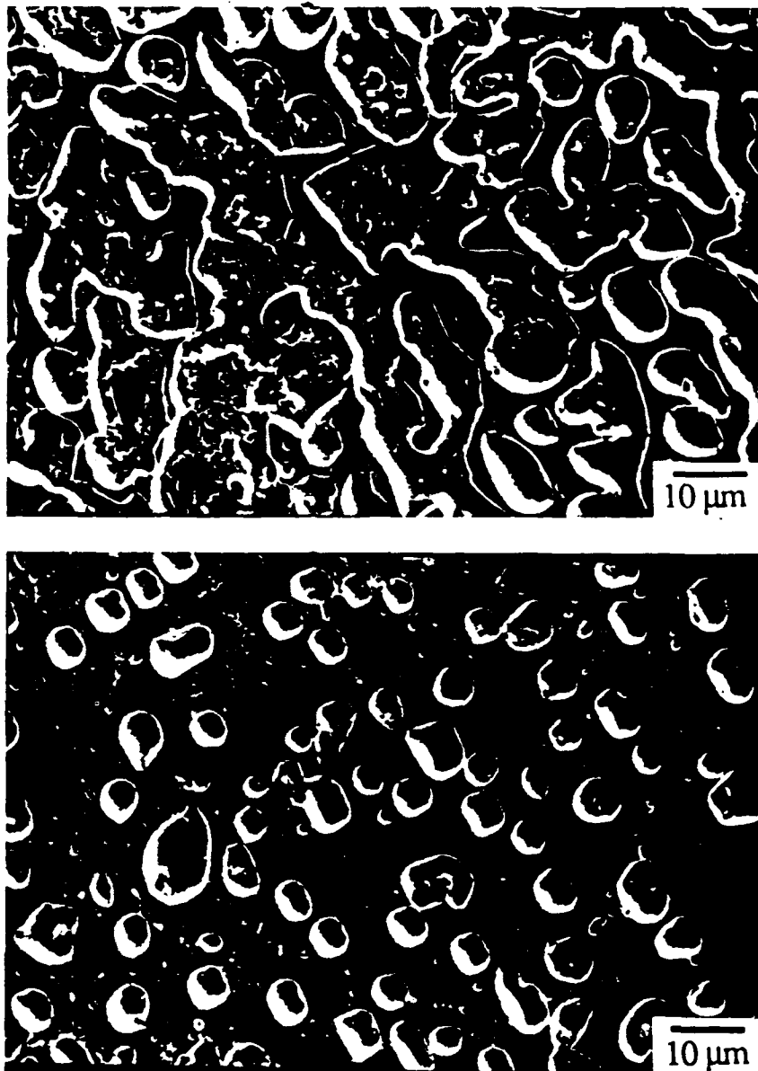
Figure 3. Pores on the copper surface of a single crystal copper-sapphire specimen held under a tensile stress of 2.64 MPa at 700°C for 48 hours. The upper photograph was taken near the edge of the specimen whereas the lower was taken closer to the middle of the same specimen.
