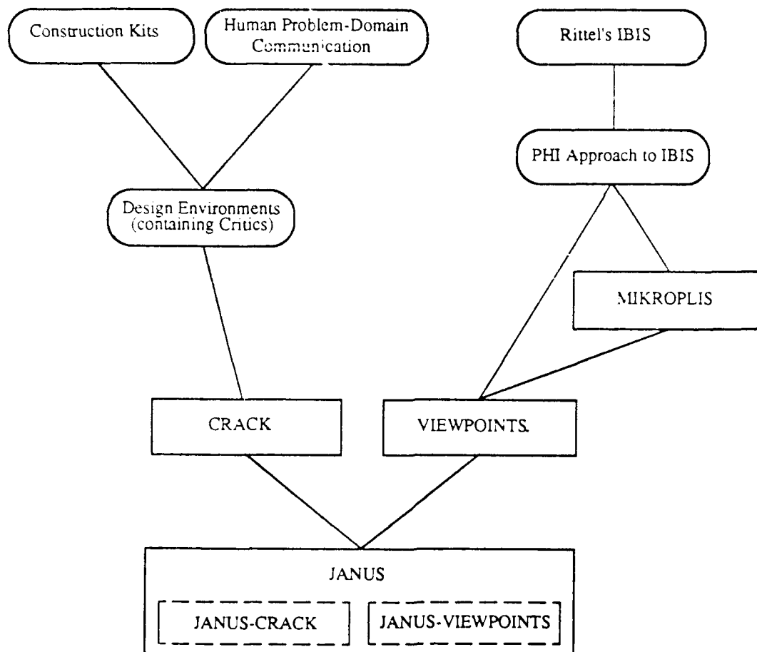
FIGURE 1. Conceptual frameworks (in ovals) and systems-building efforts (in rectangles) leading to JANUS.
