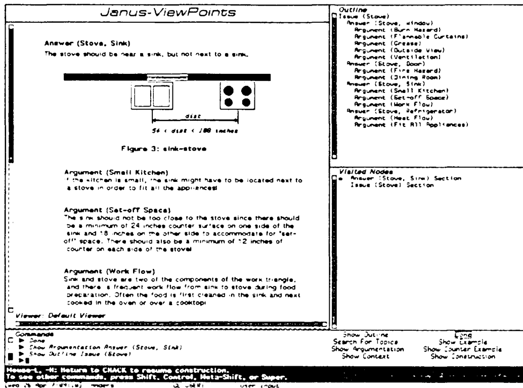
FIGURE 6. A screen image from JANUS-VIEWPOINTS.
