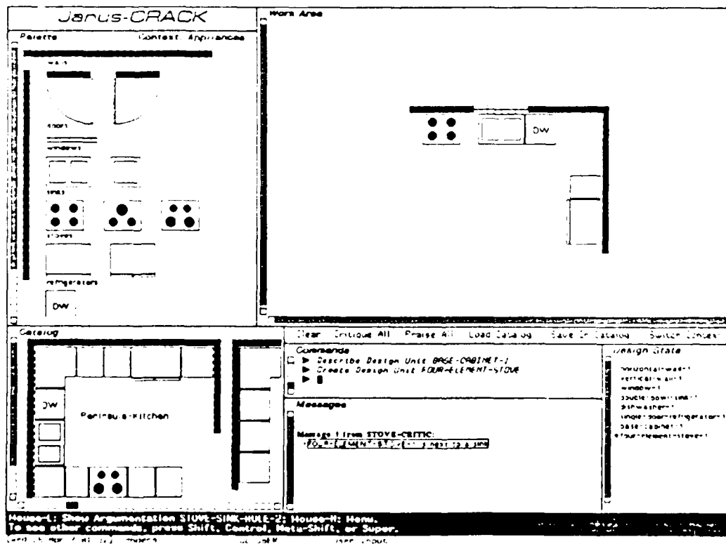
FIGURE 5. A screen image from JANUS-CRACK.
