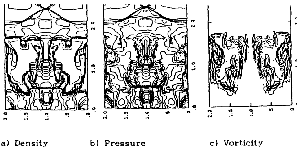
11. Field Contours 6" Downstream from Injector Discharge
