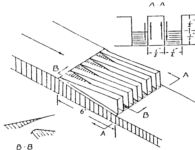
8. Configuration for Hypersonic Hydrogen Injector
