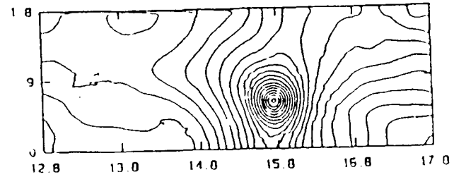
Pressure, 2.19 ms
