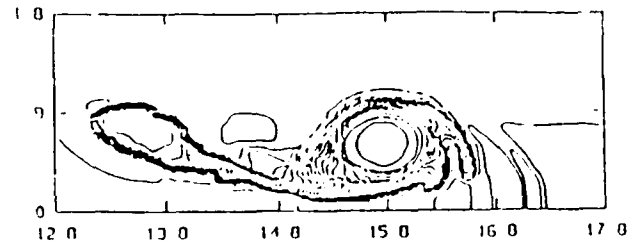
Density, 2.19 ms
