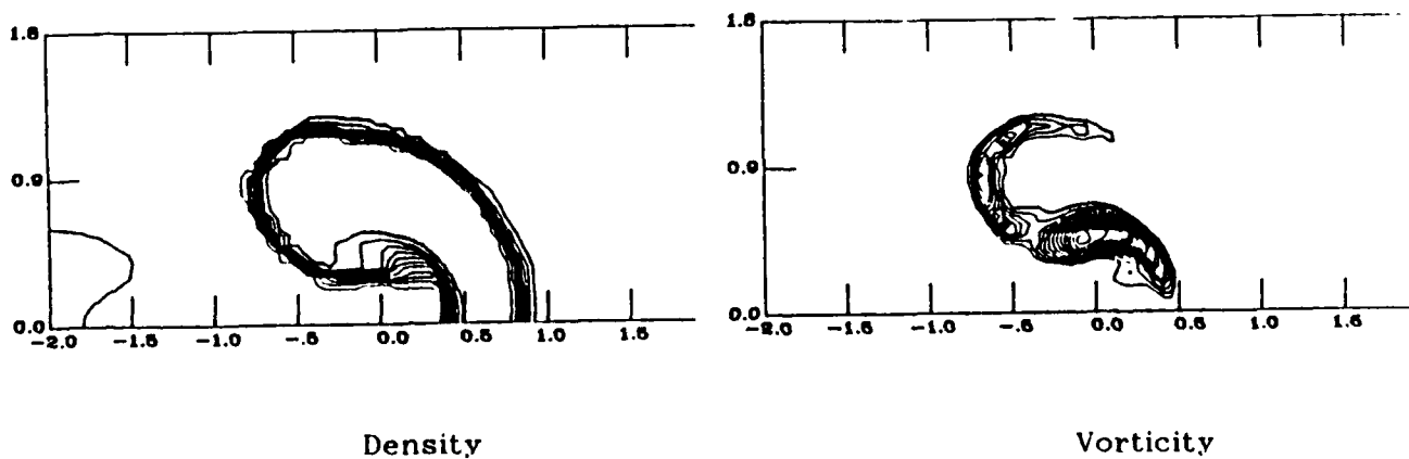
12. Density and Vorticity Contours .29 ms after Shock Impingement different manners; the vorticity-free region mixes rapidly whereas the material
