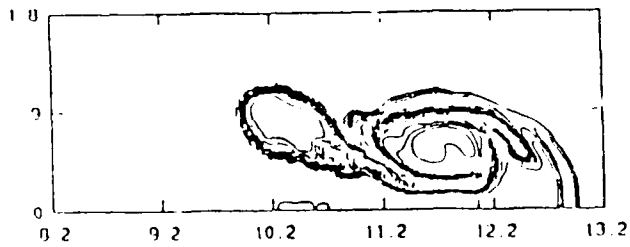
Density, 1.46 ms
