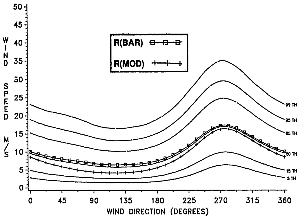
Figure E-57. Conditional Wind Speed Given Direction, January, 8 KM.
