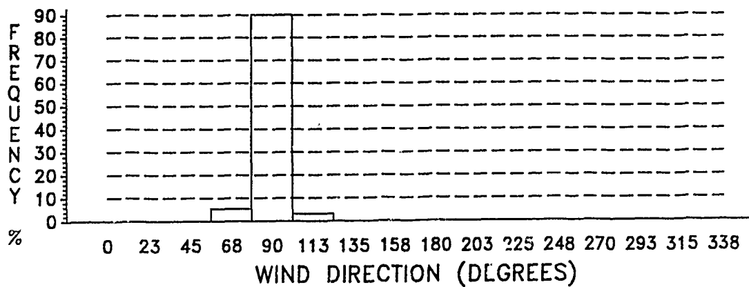
Figure E-15. Wind Direction Frequency, July, 20 KM.
