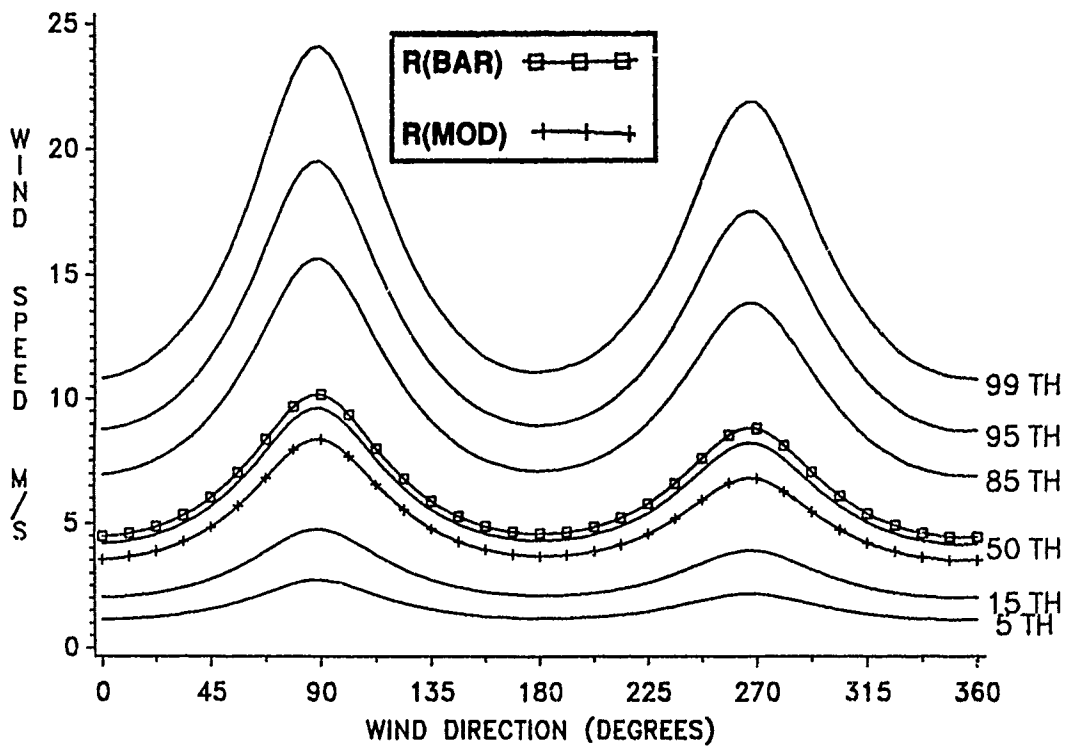
Figure E-62. Conditional Wind Speed Given Direction, January, 28 KM.
