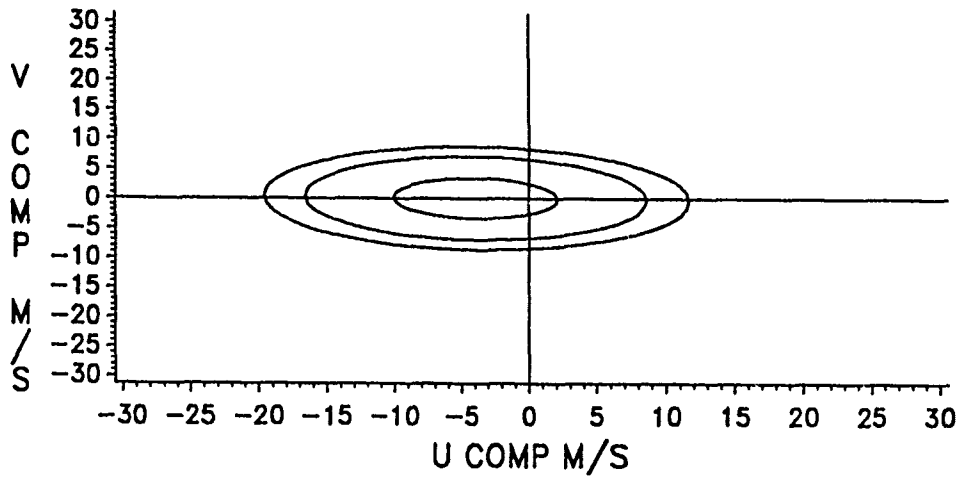
Figure E-43. Wind Probability Ellipses, January, 24 KM.
