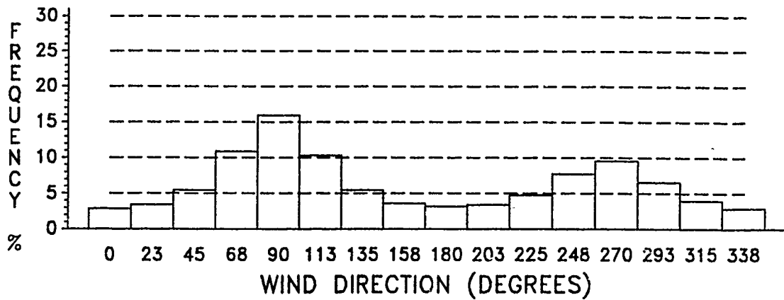
Figure E-8. Wind Direction Frequency, January, 28 KM.
