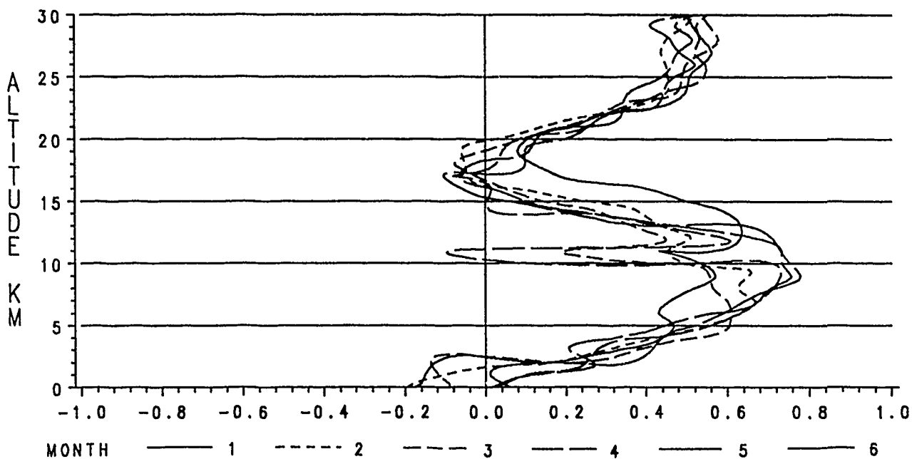
Figure F-29. Correlation Coefficients for Pressure & Temperature, January-June.
