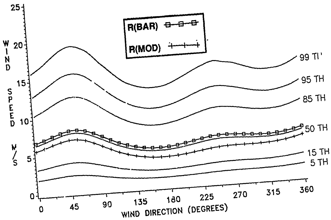
Figure E-66. Conditional Wind Speed Given Direction, July, 8 KM.
