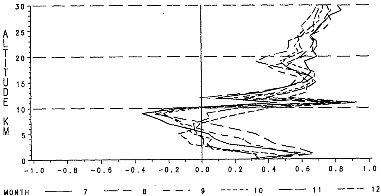
Figure F-28. Correlation Coefficients for Pressure & Density, July-December.
