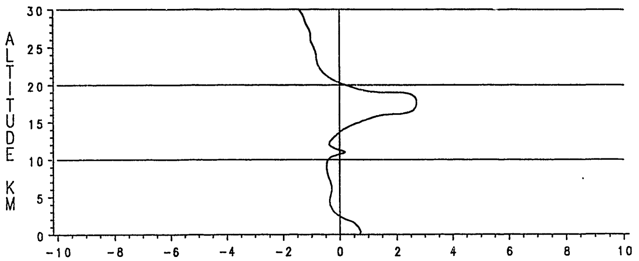
Figure F-2. Delta Percent Relative to Annual Density, January.
