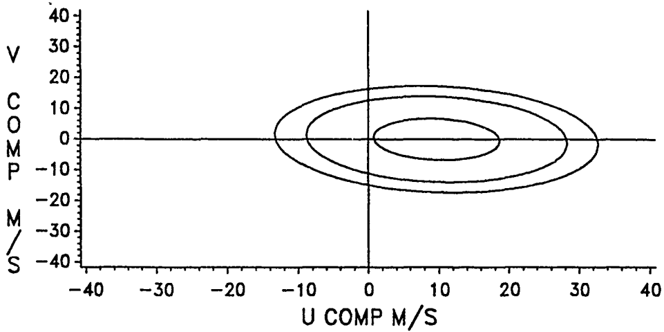
Figure E-41. Wind Probability Ellipses, January, 16 KM.
