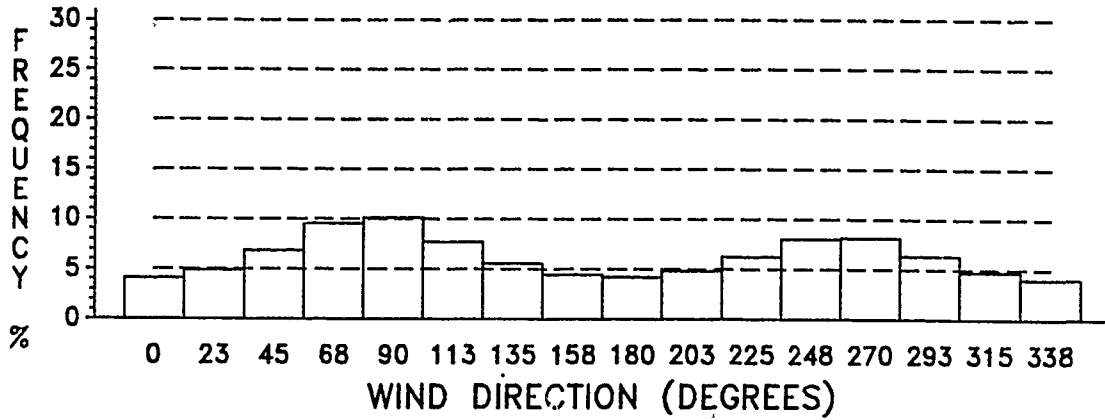
Figure E-1. Wind Direction Frequency, January, 2 KM.
