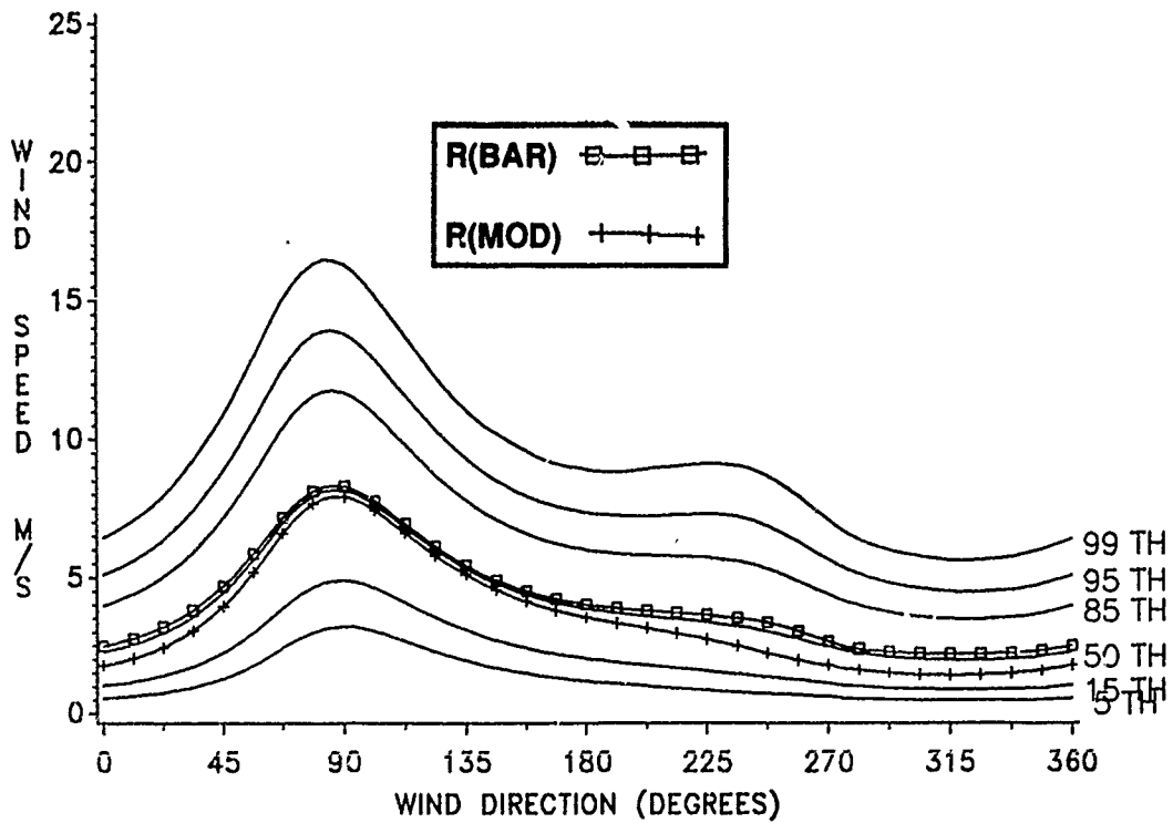
Figure E-64. Conditional Wind Speed Given Direction, July, 2 KM.
