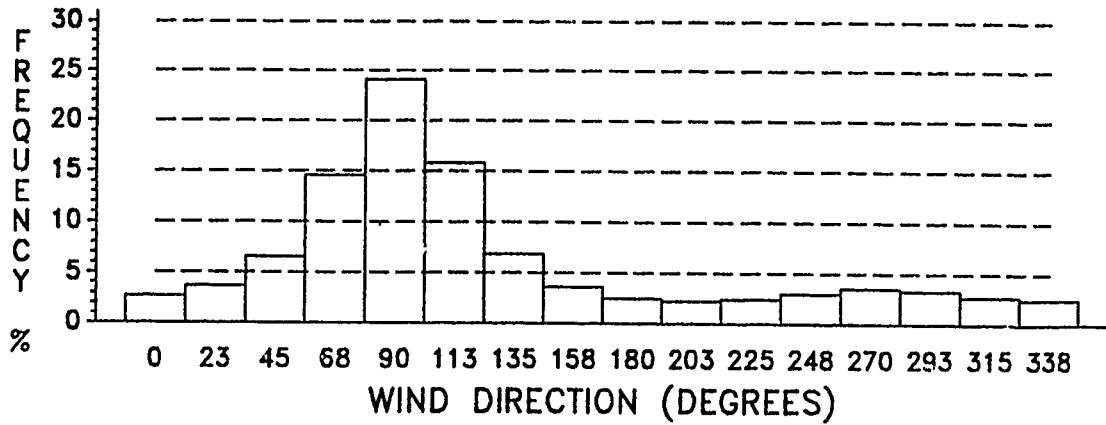
Figure E-7. Wind Direction Frequency, January, 24 KM.
