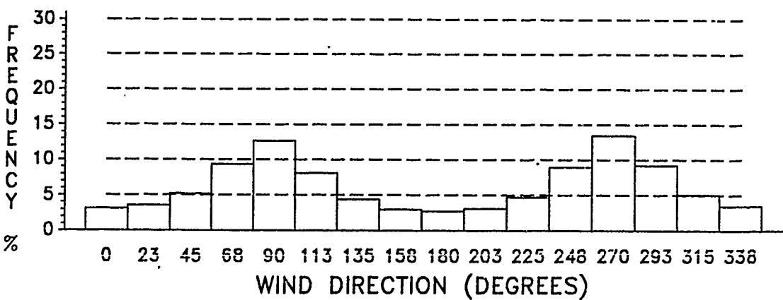
Figure E-9. Wind Direction Frequency, January, 30 KM.
