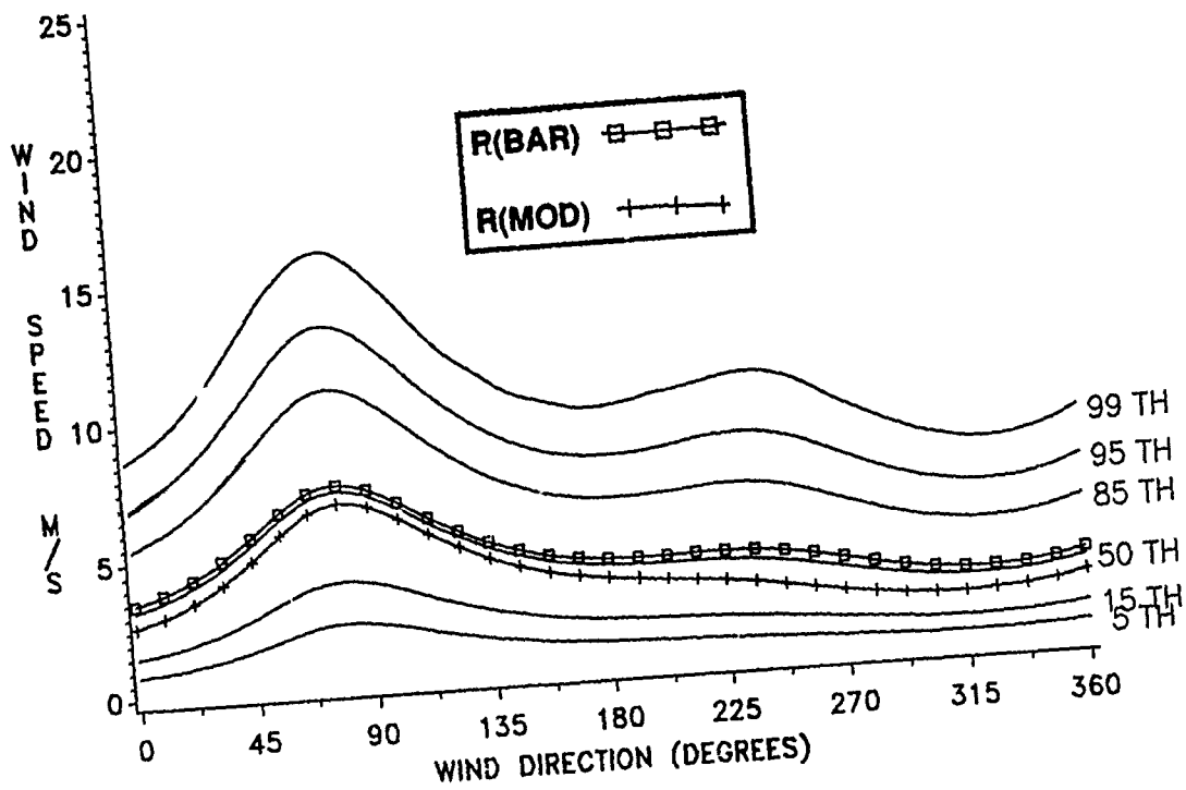
Figure E-65. Conditional Wind Speed Given Direction, July, 4 KM.
