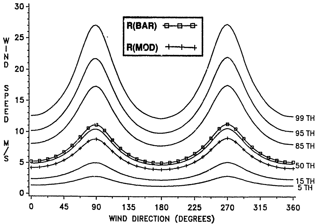
Figure E-63. Conditional Wind Speed Given Direction, January, 30 KM.
