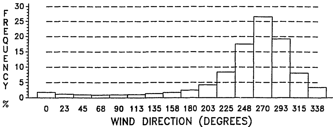
Figure E-5. Wind Direction Frequency, January, 16 KM.
