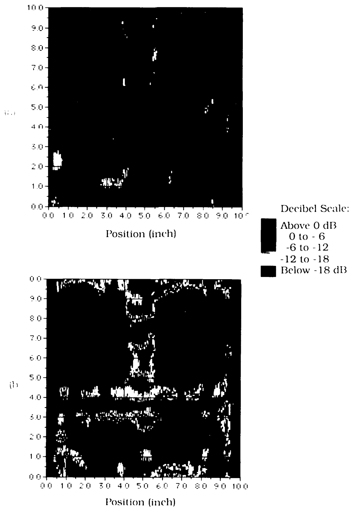
Fig. 7. C-Scans of SRMU PTS-T-2B-6. Ratio of E_{L/P} to E_{C/I} in dB vs position at (a) 0.5 MHz, and (b) 0.5 MHz.
