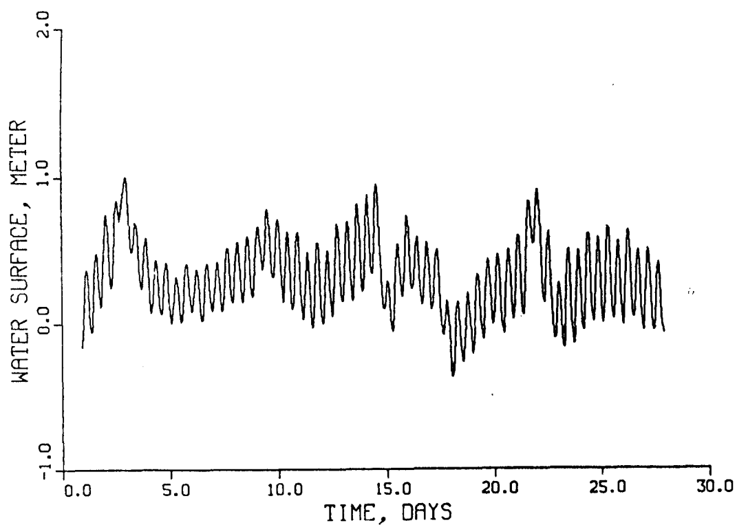
Figure 116. Tide at Colonial Beach, VA, corrected at NGVD during April 1983
