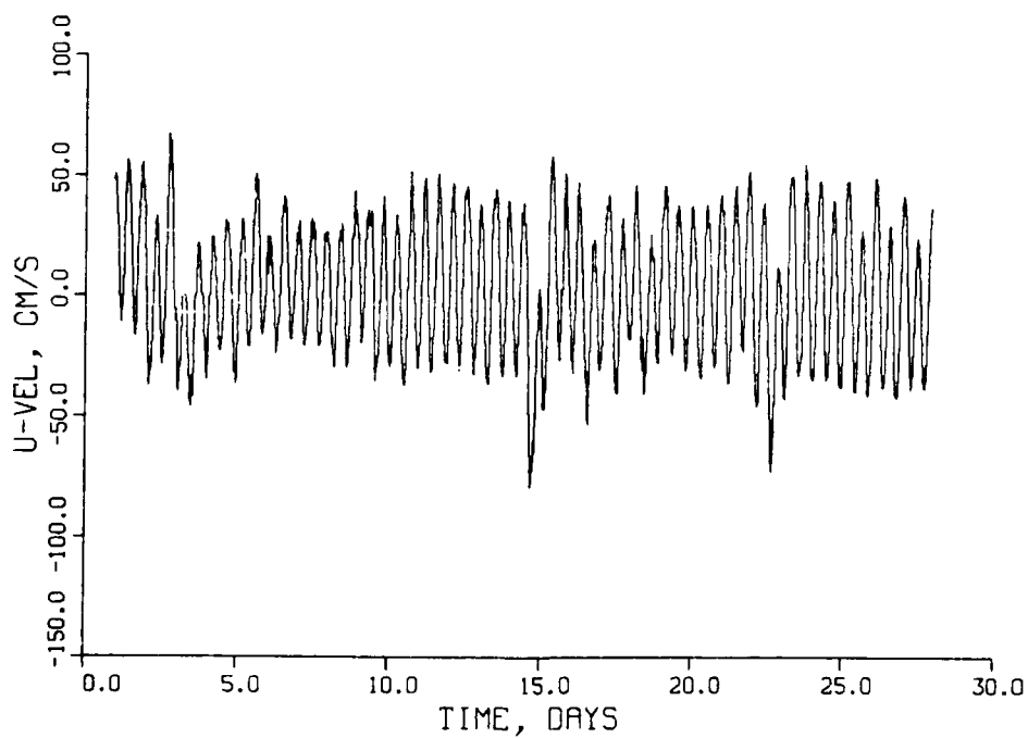
Figure 88. U-velocity at station WT during April 1983
