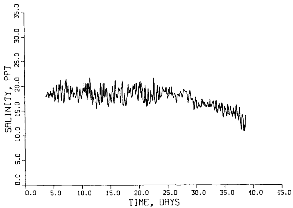
Figure 55. Salinity at station WT3 at a depth of 9 ft from CRIMP data
