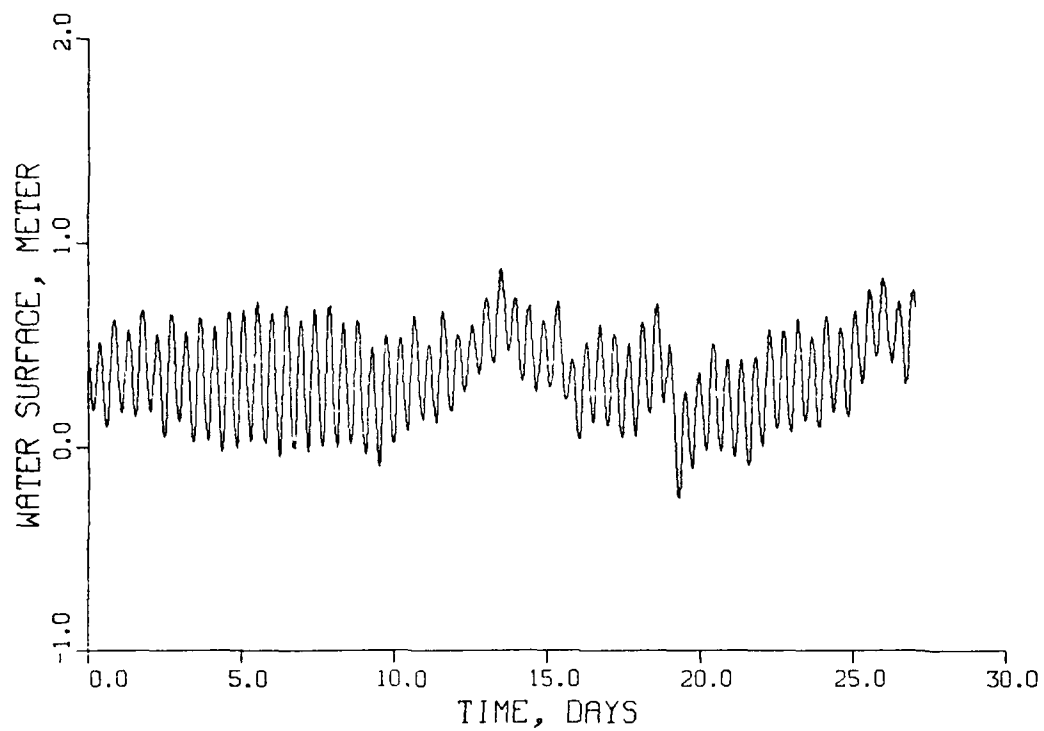
Figure 142. Tide at Colonial Beach, VA, corrected to NGVD during September 1983
