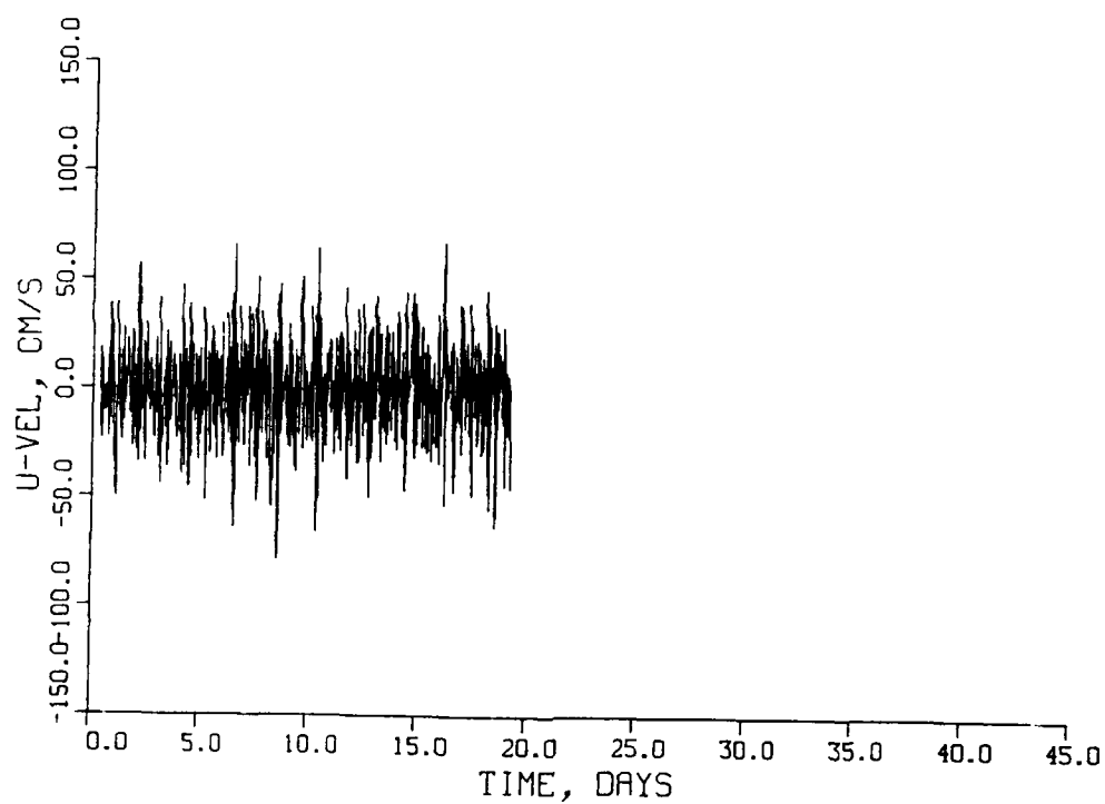
Figure 40. U-velocity at station BB1 at a depth of 9 ft from CRIMP data
