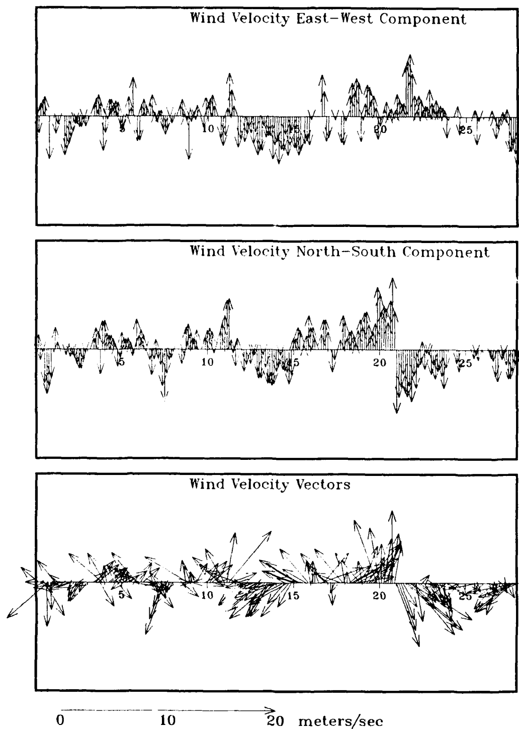
Figure 136. Wind data at Patuxent River Naval Air Station during September 1983
