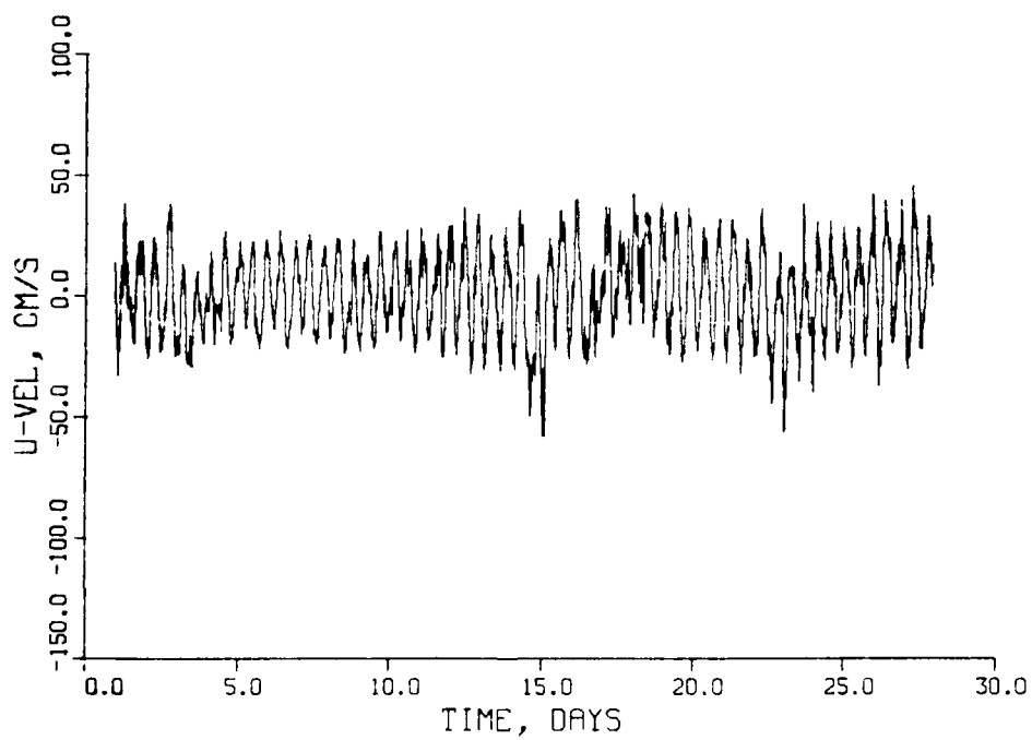
Figure 86. U-velocity at station BE during April 1983
