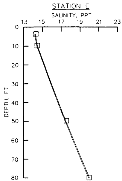
Figure 8. Salinity from physical model during steady-state testing conditions
