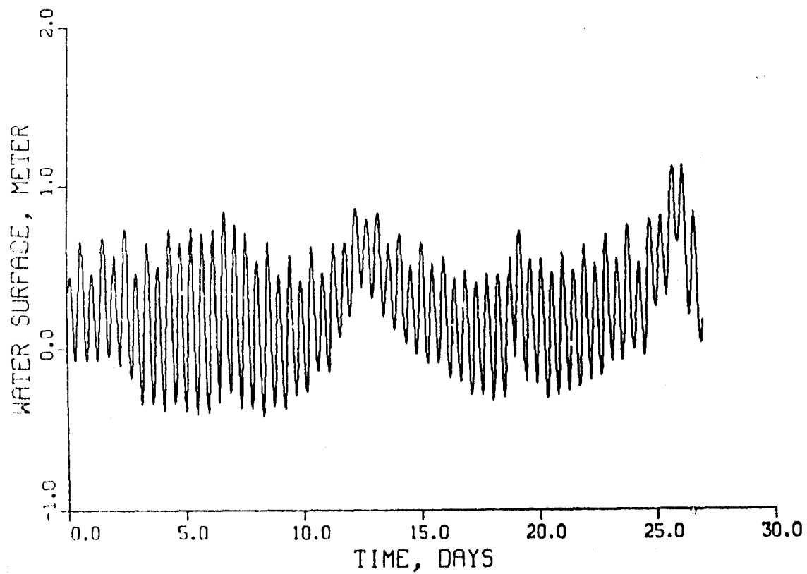
Figure 140. Tide at Chesapeake Bay Tunnel corrected to NGVD during September 1983
