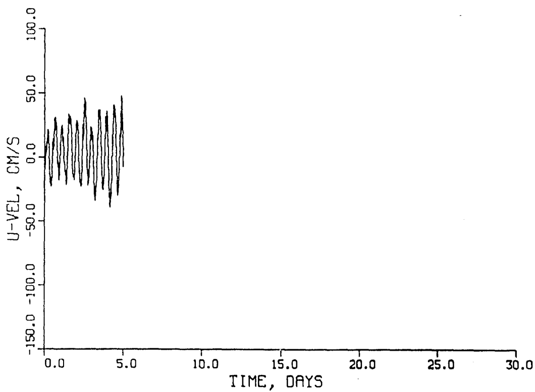
Figure 122. U-velocity at station WT during September 1983
