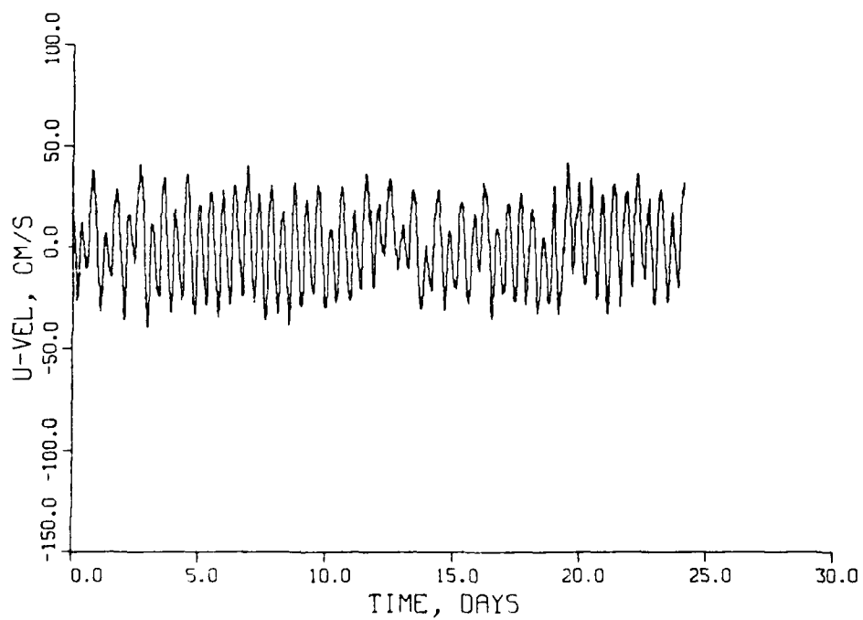
Figure 124. U-velocity at station MB during September 1983
