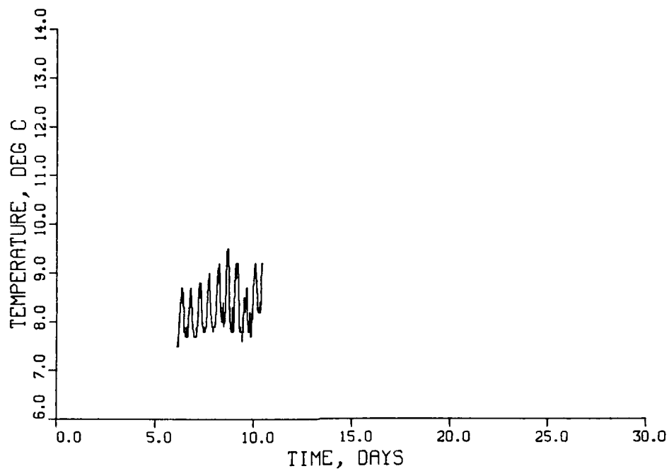
Figure 108. Temperature at Pooles Island at a depth of 5.5 m during April 1983
