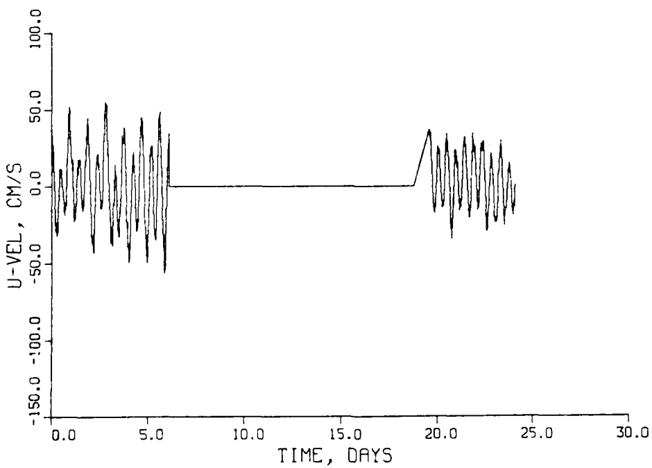
Figure 126. U-velocity at station BB during September 1983 (Continued)
