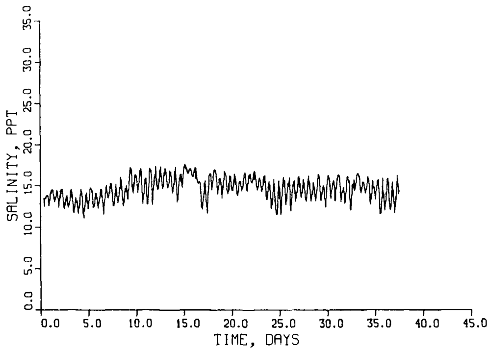
Figure 60. Salinity at station BB1 from CRIMP data
