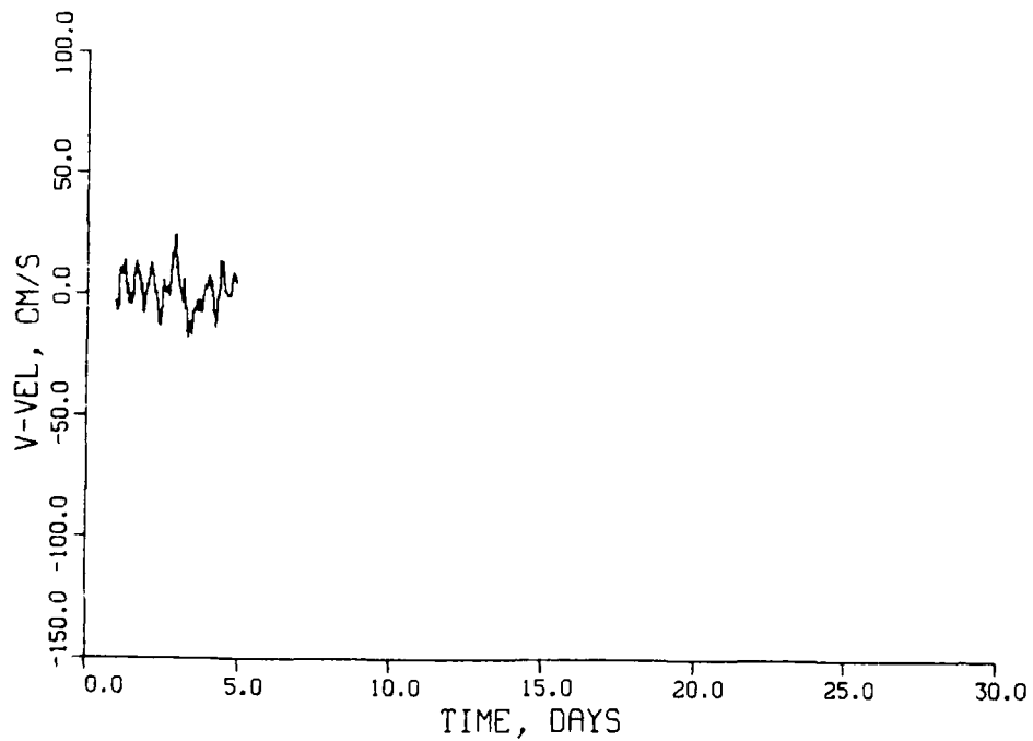
Figure 91. V-velocity at station MB during April 1983
