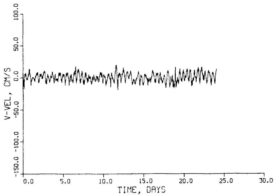
Figure 125. V-velocity at station MB during September 1983
