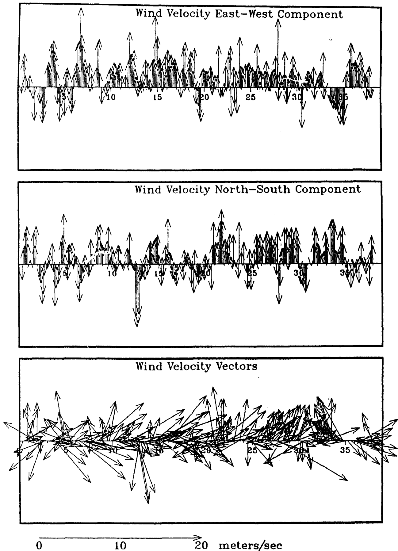
Figure 78. Wind data at Baltimore-Washington International Airport from CRIMP data
