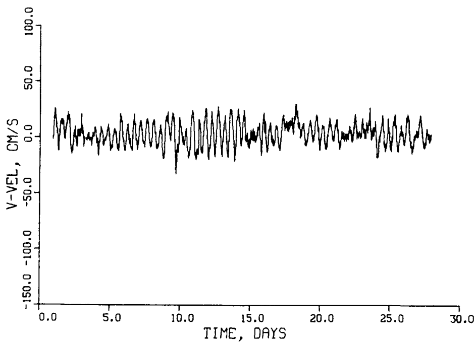
Figure 89. V-velocity at station WT during April 1983
