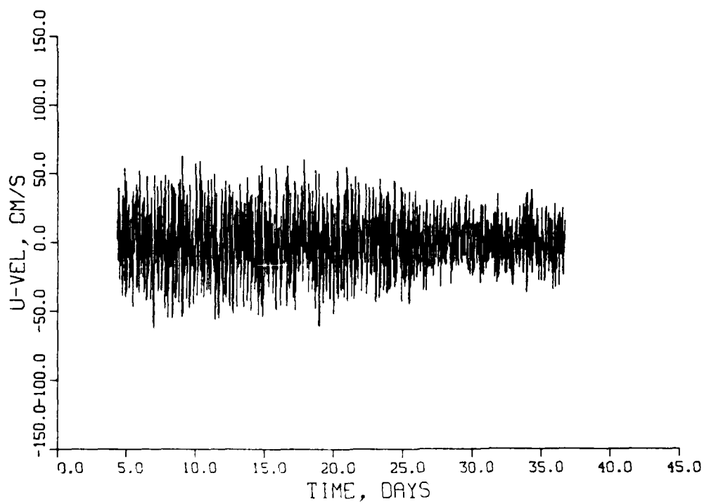
Figure 28. U-velocity at station TS1 from CRIMP data (Continued)
