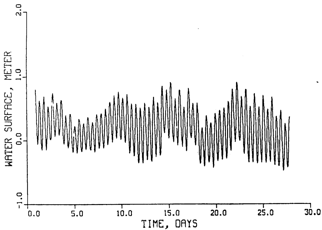
Figure 114. Tide at Chesapeake Bay Tunnel corrected at NGVD during April 1983
