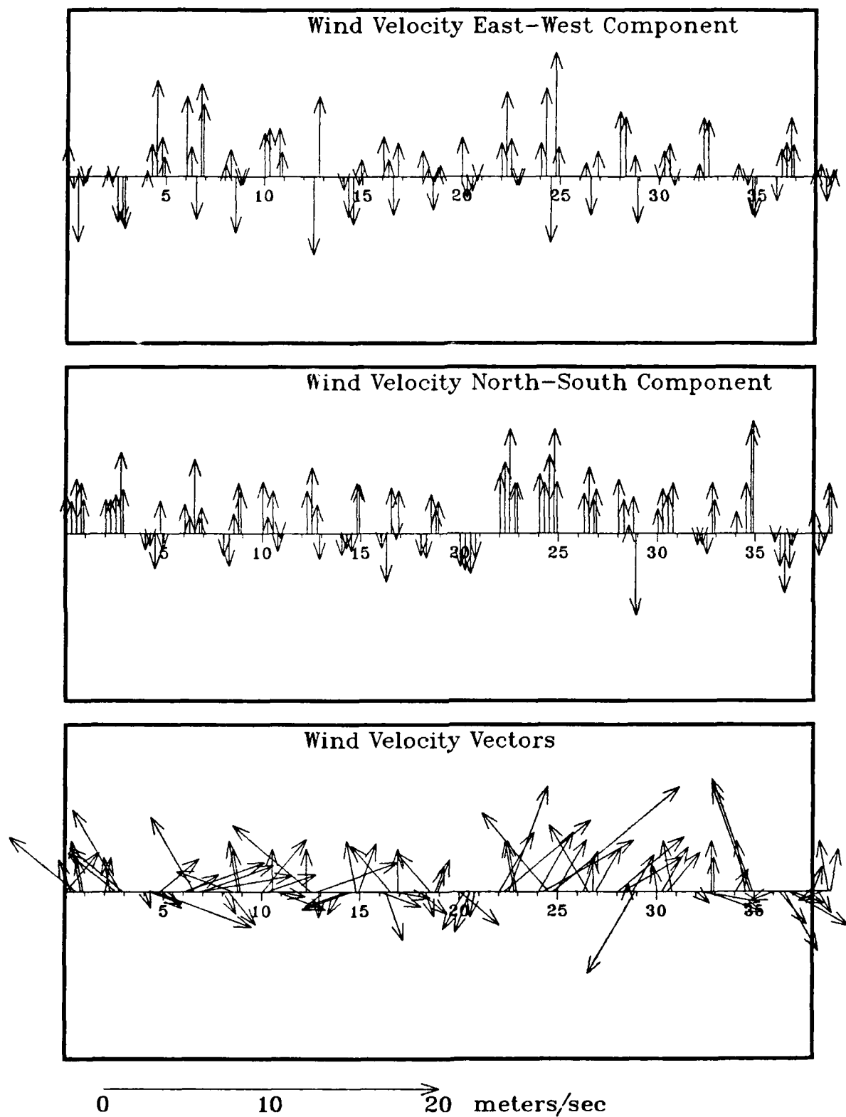
Figure 76. Wind data at the Patuxent Naval Air Station from CRIMP data
