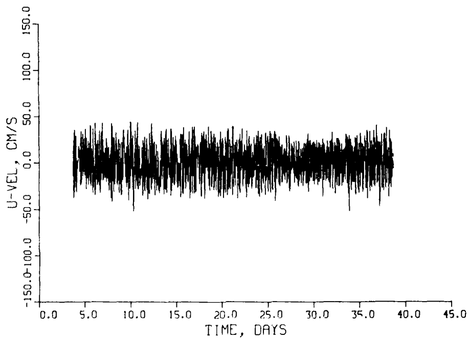
Figure 26. U-velocity at station WT5 from CRIMP data
