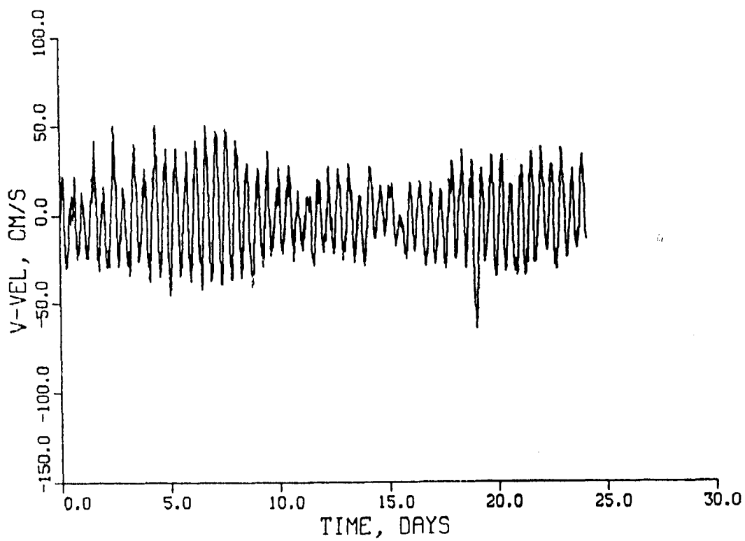
Figure 121. V-velocity at station BE during September 1983
