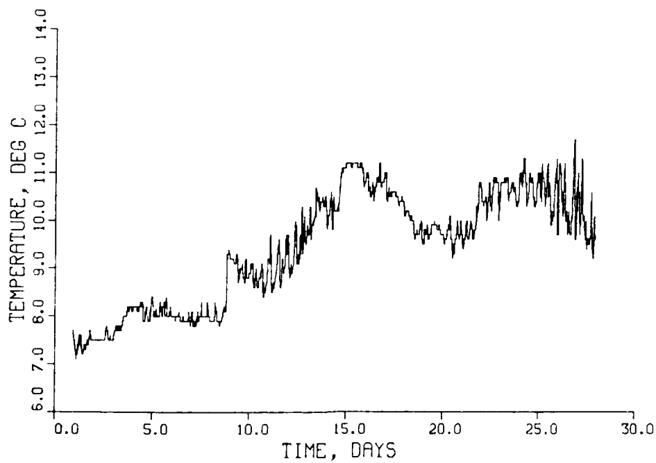
Figure 104. Temperature at station BE during April 1983
