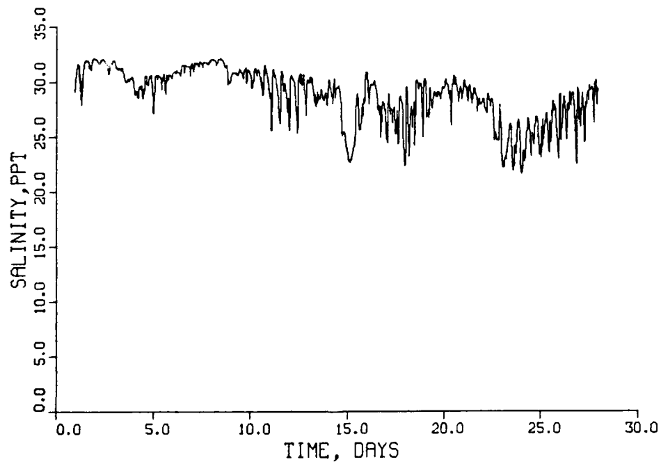
Figure 98. Salinity at station BE during April 1983
