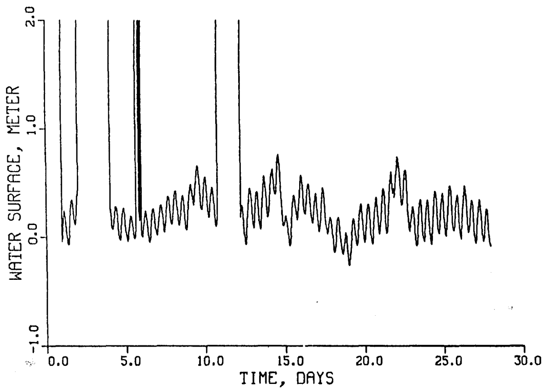
Figure 117. Tide at Solomons, MD, corrected to NGVD during April 1983
