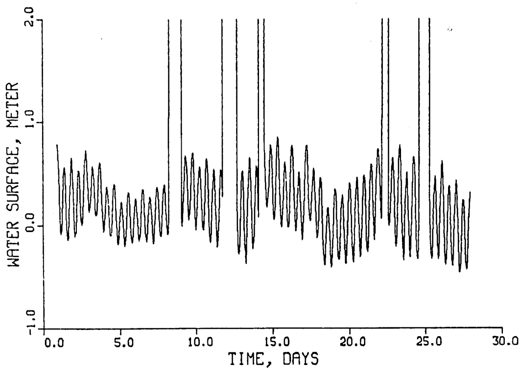
Figure 115. Tide at Hampton Roads, VA, corrected to NGVD during April 1983
