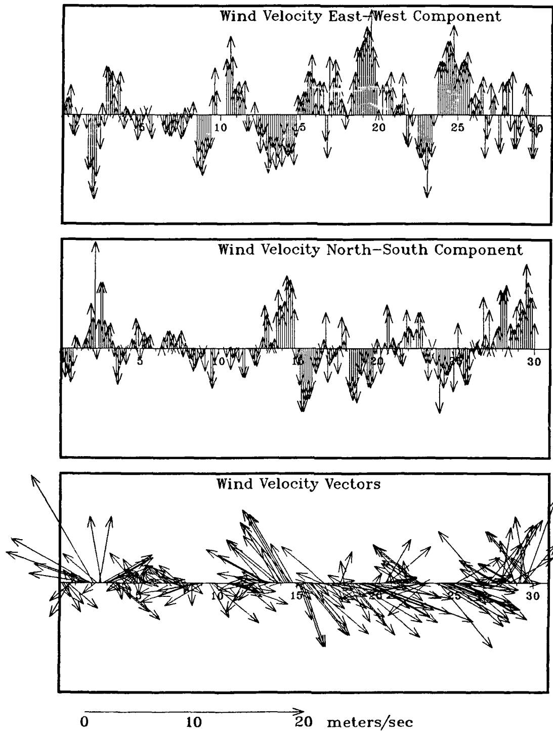
Figure 110. Wind data at Patuxent River Naval Air Station during April 1983
