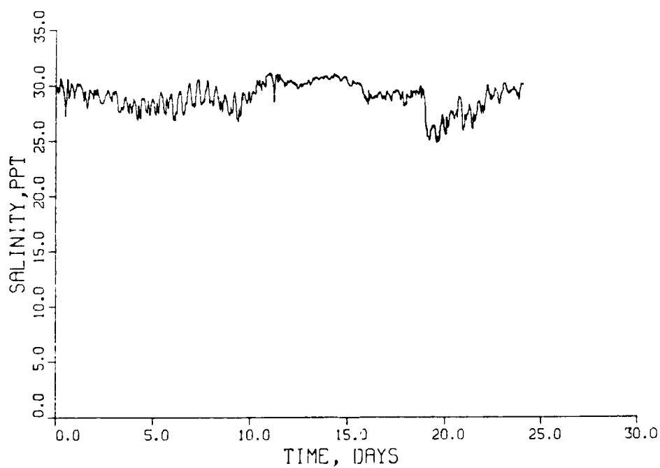
Figure 128. Salinity at station BE during September 1983
