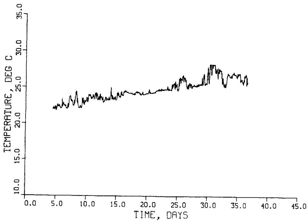
Figure 71. Temperature at station SP2 from CRIMP data
