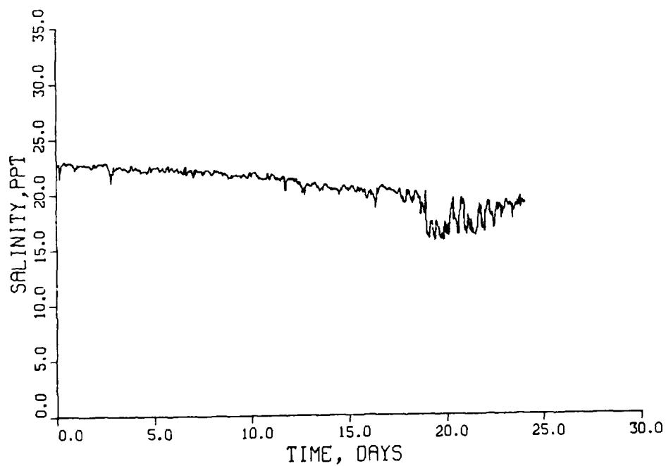
Figure 130. Salinity at station MB during September 1983
