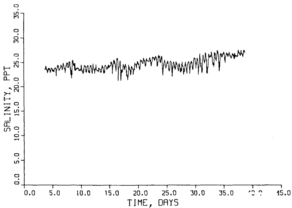
Figure 56. Salinity at station WT4 from CRIMP data
