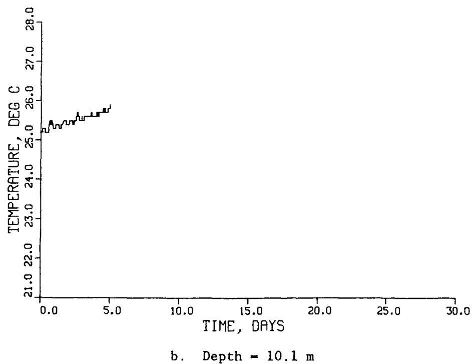
Figure 133. Temperature at station WT during September 1983
