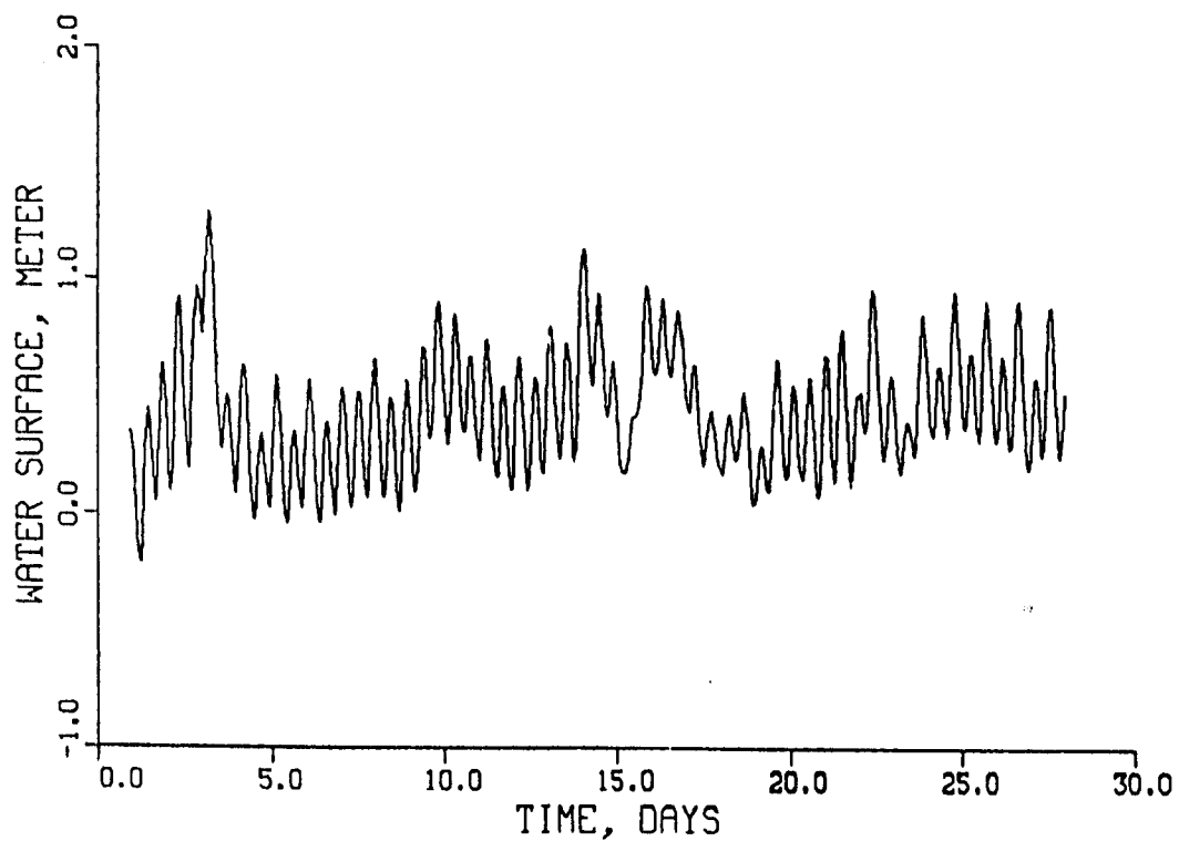
Figure 119. Tide at Havre de Grace, MD, corrected to NGVD during April 1983
