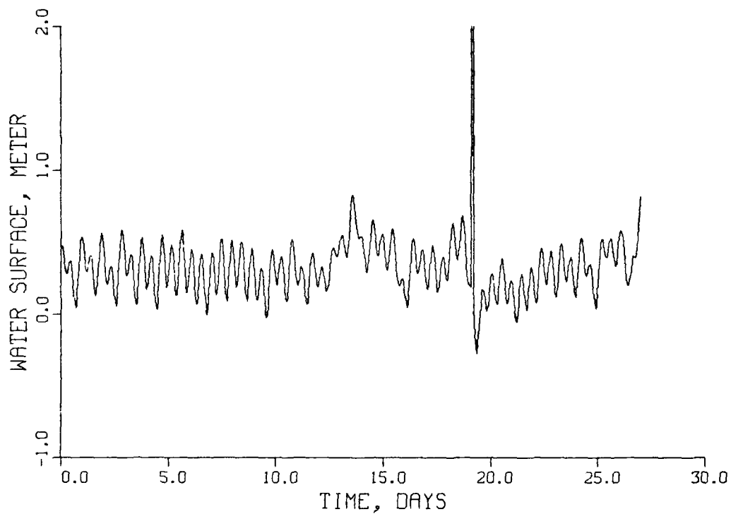
Figure 144. Tide at Annapolis, MD, corrected to NGVD during September 1983
