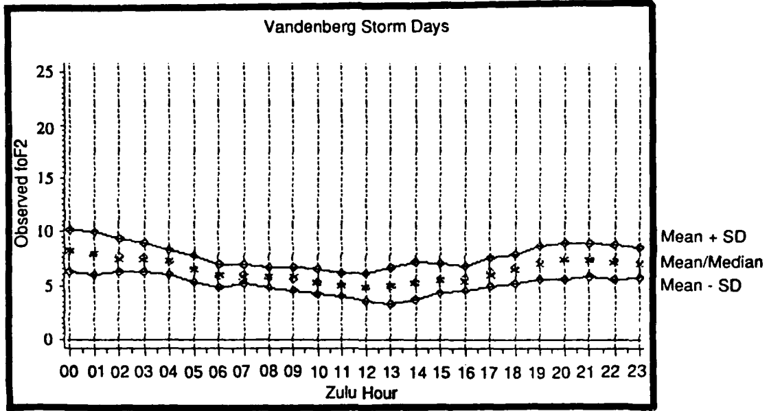
Figure 5b. Hourly Distributions of Observed foF2 (MHz) for Vandenberg, Storm Days.
