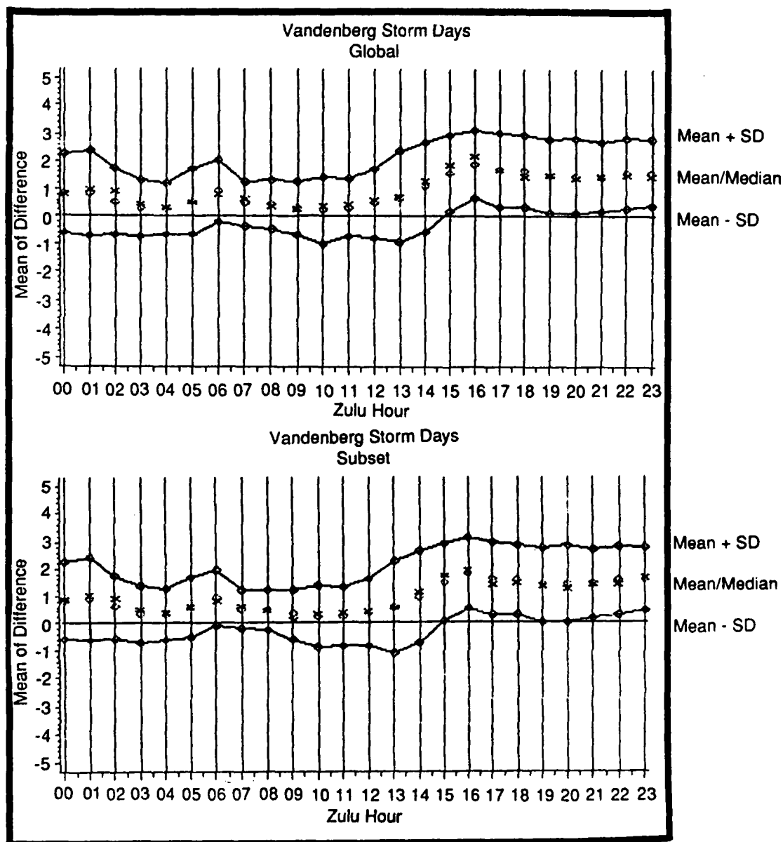
Figure 4a. Means ( \bar{x} ), Medians ( \hat{\phi} ), and Standard Deviations of Distributions of Modeled-Observed Storm-Days foF2 (MHz) for Vandenberg by Zulu Hour.
