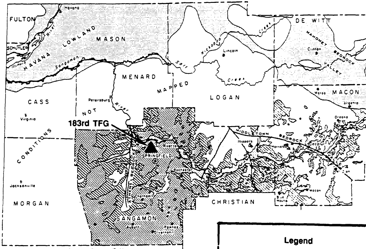
Figure 12 Groundwater Conditions at the Base and West-Central Illinois
