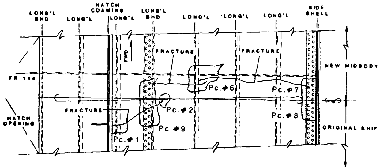
PLAN OF SPAR DECK
