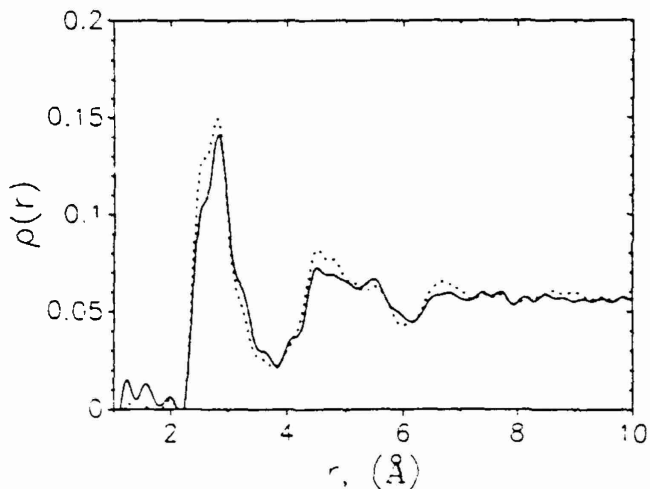
FIG. 3. Total pair density function of Al 90 Fe 5 Ce 3 (solid line) and Al 90 Fe 7 Ce 3 (dashed line) derived from the neutron scattering experiment.
