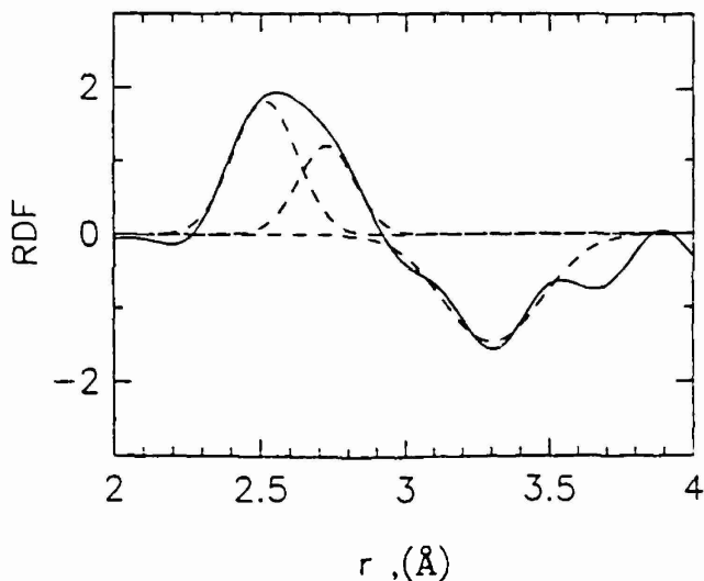
FIG. 5. Difference between the radial distribution function of Al 90 Fe 7 Ce 3 and the radial distribution function of Al 90 Fe 5 Ce 3 , fitted by three Gaussian functions (dashed lines). Areas and positions of the three Gaussian functions are listed in Table II.
