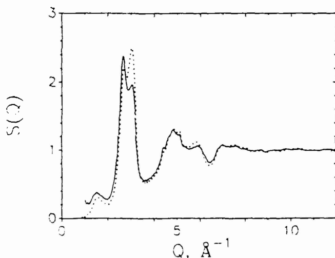
FIG. 1. Total structure factor, S(Q) , of amorphous Al 90 Fe 5 Ce 5 (solid line) and Al 90 Fe 7 Ce 3 (dashed line) determined by the pulsed neutron scattering experiment.
