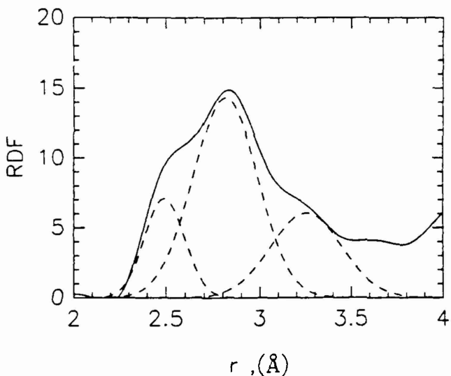
FIG. 4. The first peak of the radial distribution function of Al 90 Fe 7 Ce 3 , fitted by three Gaussian functions (dashed lines). Areas and positions of the three Gaussian functions are listed in Table II.
