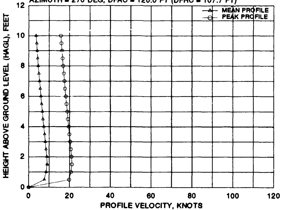
FIGURE J-2 ISHIDA TW-68 MEAN AND PEAK VELOCITY PROFILES FOR EIGHT 270 DEGREE AZIMUTH RADIAL STATIONS AT A WHEEL HEIGHT OF 15 FEET AND A GROSS WEIGHT OF 12,500 POUNDS (Concluded)
