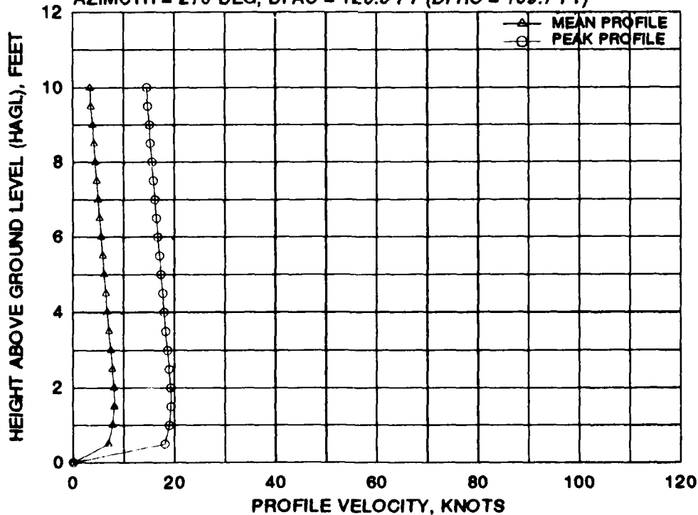
FIGURE I-2 CANADAIR CL-84 MEAN AND PEAK VELOCITY PROFILES FOR EIGHT 270 DEGREE AZIMUTH RADIAL STATIONS AT A WHEEL HEIGHT OF 15 FEET AND A GROSS WEIGHT OF 12,200 POUNDS (Concluded)
