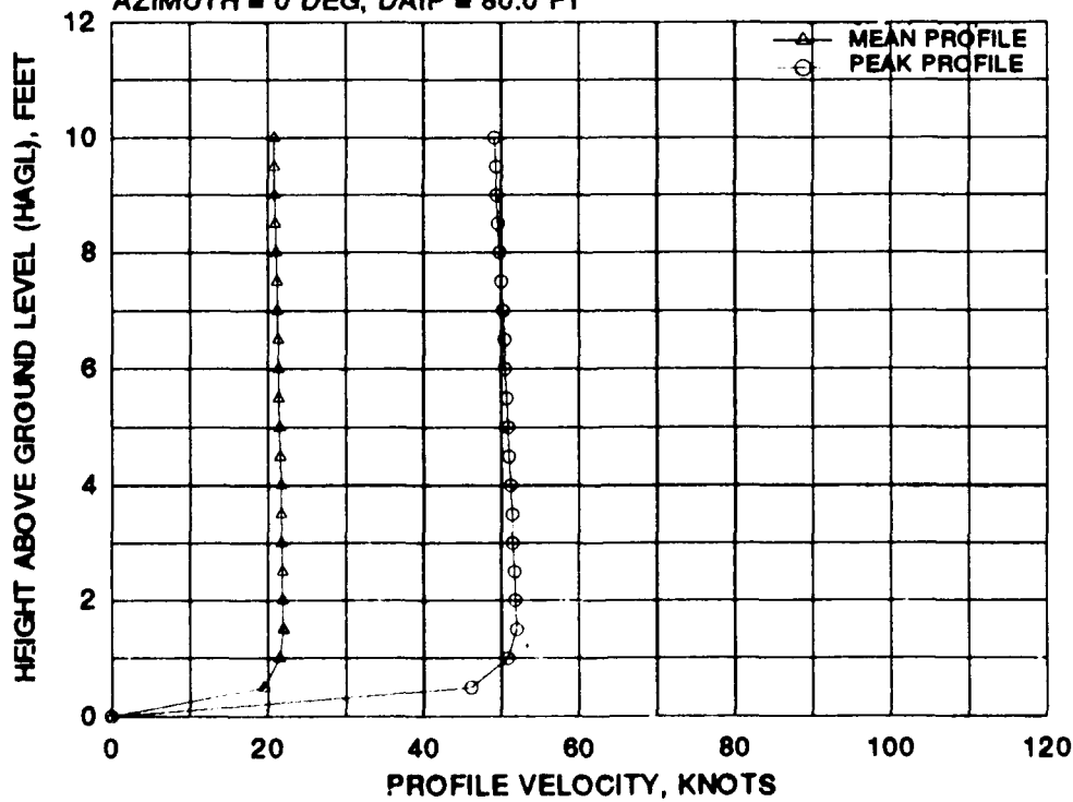
FIGURE A-3 BELL XV-15 MEAN AND PEAK VELOCITY PROFILES FOR EIGHT 0 DEGREE AZIMUTH RADIAL STATIONS AT A WHEEL HEIGHT OF 20 FEET AND A GROSS WEIGHT OF 13,000 POUNDS (Continued)
