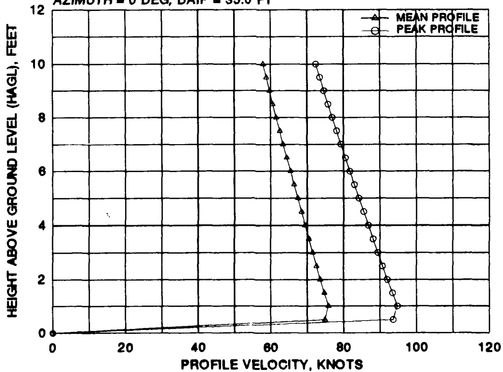
FIGURE B-9 BELL/BOEING MV-22 MEAN AND PEAK VELOCITY PROFILES FOR NINE 0 DEGREE AZIMUTH RADIAL STATIONS AT A WHEEL HEIGHT OF 30 FEET AND A GROSS WEIGHT OF 47,500 POUNDS
