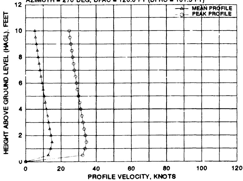
FIGURE E-2 CTR-1900 MEAN AND PEAK VELOCITY PROFILES FOR EIGHT 270 DEGREE AZIMUTH RADIAL STATIONS AT A WHEEL HEIGHT OF 30 FEET AND A GROSS WEIGHT OF 22,800 POUNDS (Continued)
