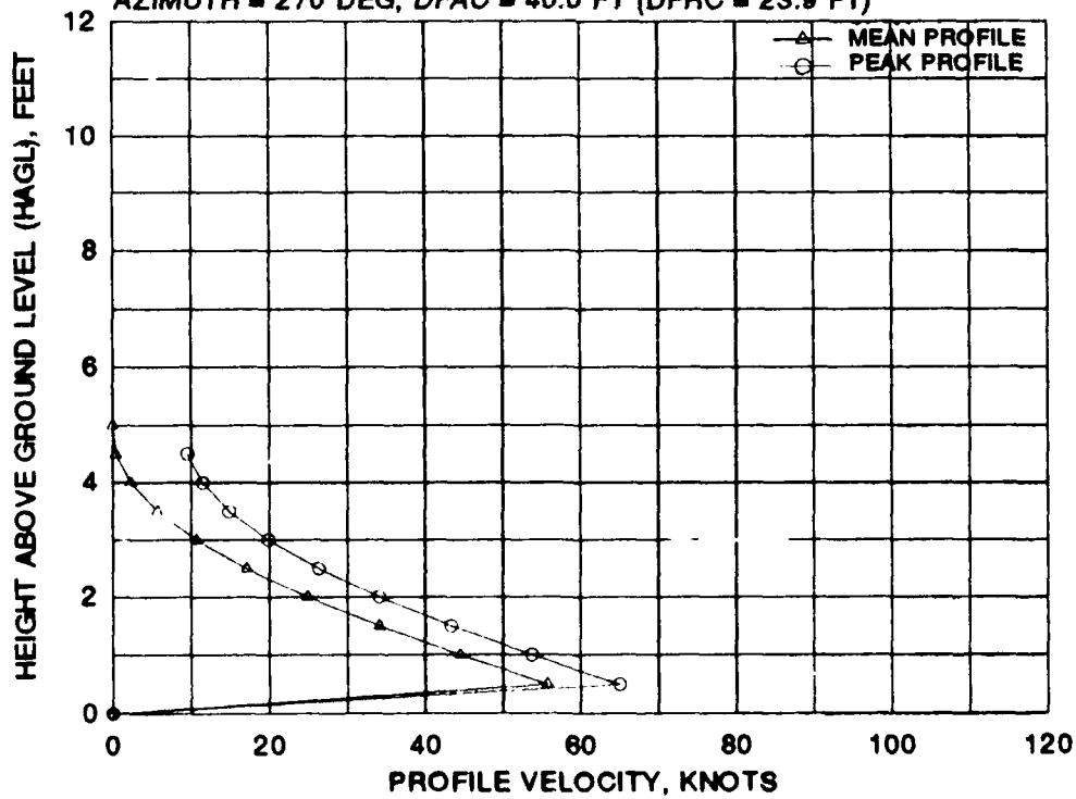
FIGURE A-2 BELL XV-15 MEAN AND PEAK VELOCITY PROFILES FOR EIGHT 270 DEGREE AZIMUTH RADIAL STATIONS AT A WHEEL HEIGHT OF 20 FEET AND A GROSS WEIGHT OF 13,000 POUNDS
