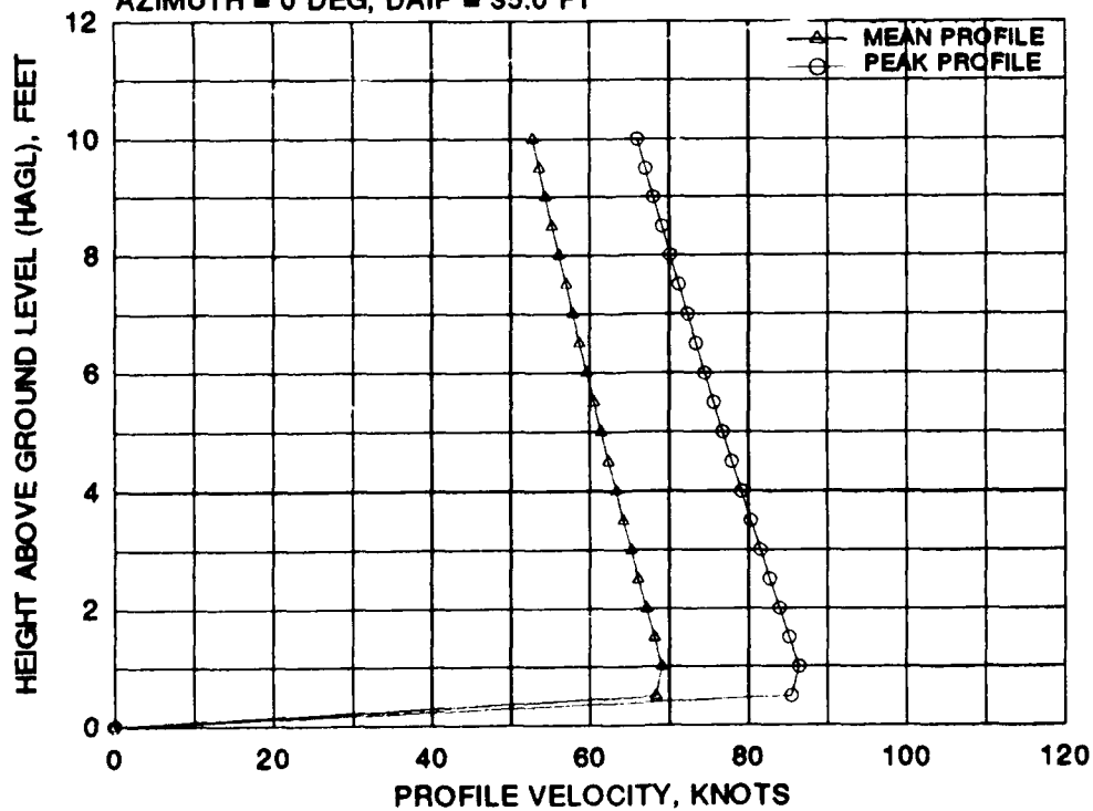
FIGURE B-6 BELL/BOEING MV-22 MEAN AND PEAK VELOCITY PROFILES FOR NINE 0 DEGREE AZIMUTH RADIAL STATIONS AT A WHEEL HEIGHT OF 5 FEET AND A GROSS WEIGHT OF 40,000 POUNDS
