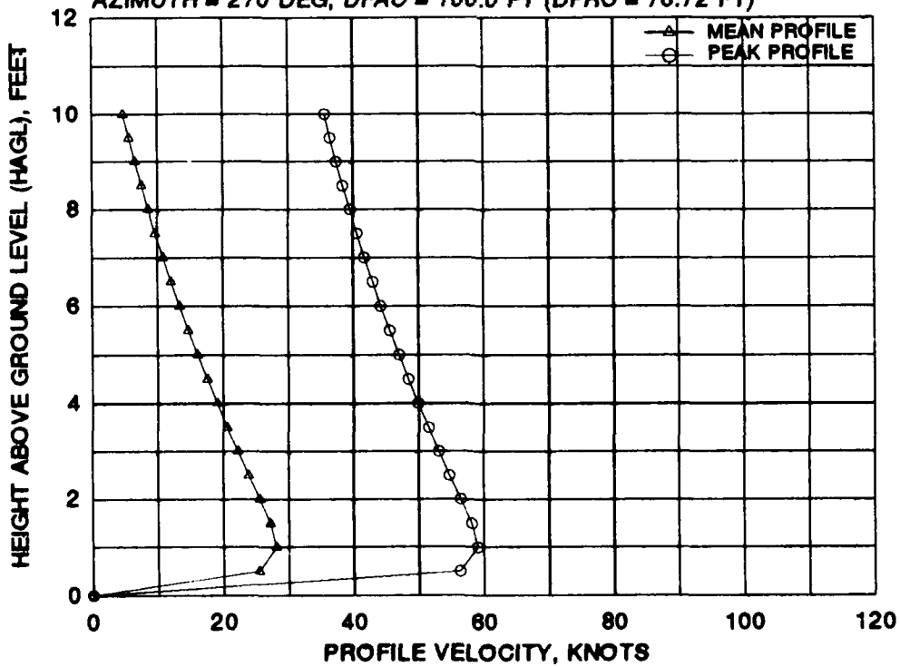
FIGURE B-2 BELL/BOEING MV-22 MEAN AND PEAK VELOCITY PROFILES FOR EIGHT 270 DEGREE AZIMUTH RADIAL STATIONS AT A WHEEL HEIGHT OF 5 FEET AND A GROSS WEIGHT OF 40,000 POUNDS (Continued)
