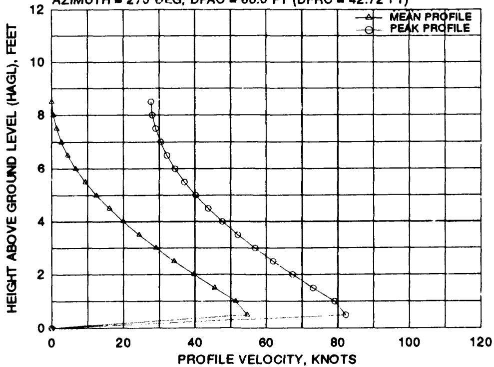
FIGURE B-3 BELL/BOEING MV-22 MEAN AND PEAK VELOCITY PROFILES FOR EIGHT 270 DEGREE AZIMUTH RADIAL STATIONS AT A WHEEL HEIGHT OF 30 FEET AND A GROSS WEIGHT OF 40,000 POUNDS
