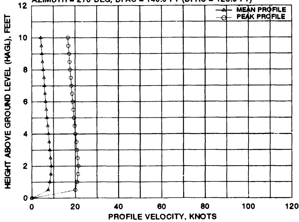
FIGURE A-2 BELL XV-15 MEAN AND PEAK VELOCITY PROFILES FOR EIGHT 270 DEGREE AZIMUTH RADIAL STATIONS AT A WHEEL HEIGHT OF 20 FEET AND A GROSS WEIGHT OF 13,000 POUNDS (Concluded)
