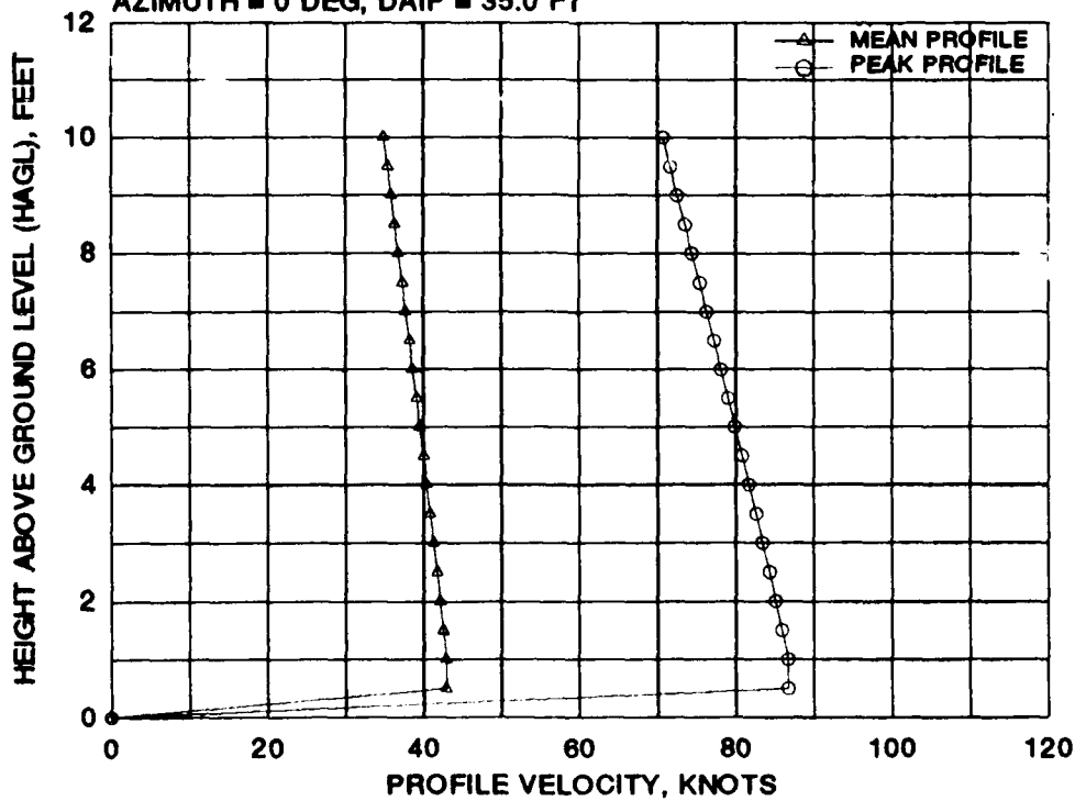
FIGURE I-3 CANADAIR CL-84 MEAN AND PEAK VELOCITY PROFILES FOR EIGHT 0 DEGREE AZIMUTH RADIAL STATIONS AT A WHEEL HEIGHT OF 15 FEET AND A GROSS WEIGHT OF 12,200 POUNDS (Continued)
