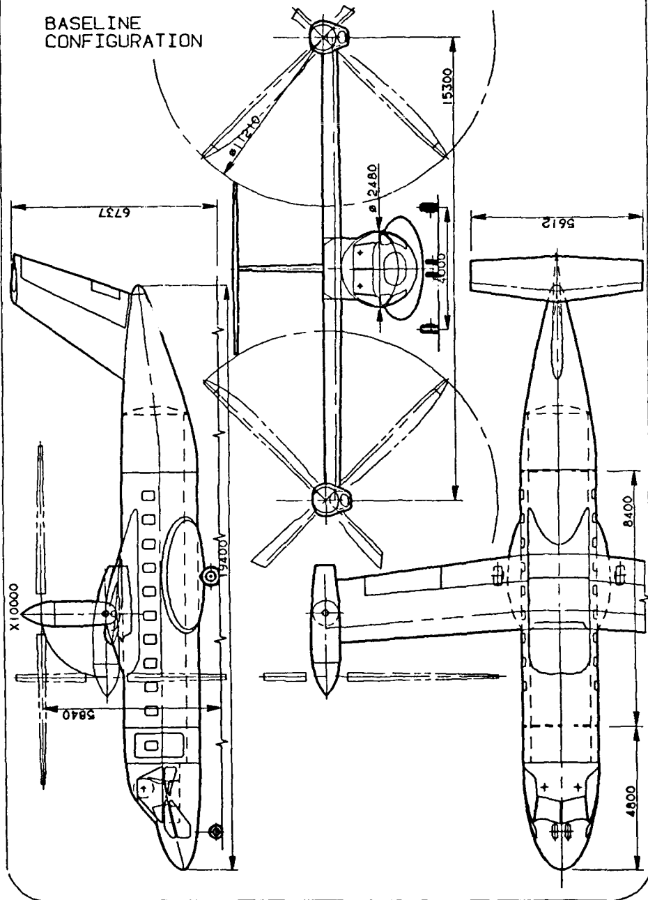
FIGURE H-1 THREE-VIEW DRAWING OF THE EUROFAR TILTROTOR
