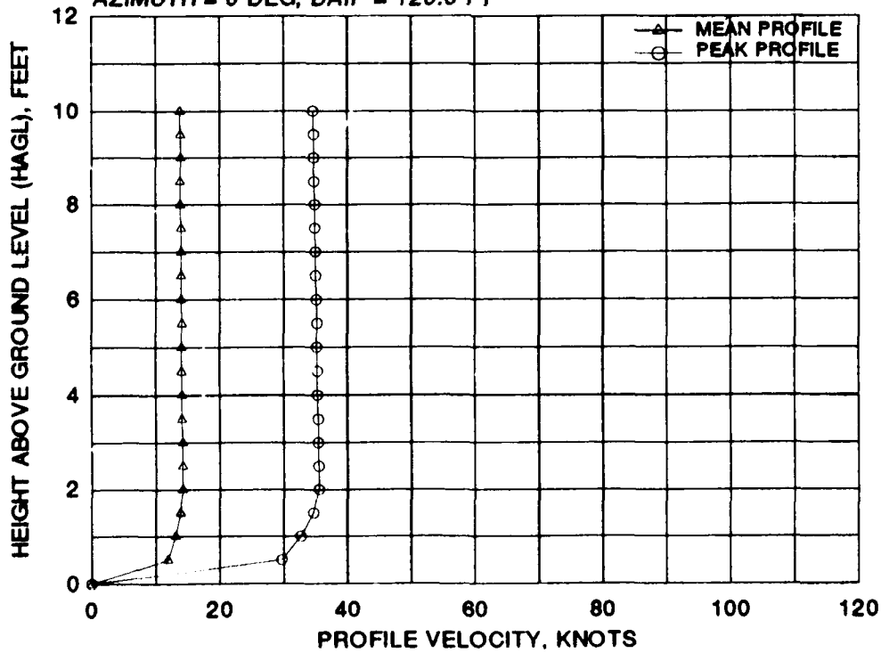
FIGURE A-3 BELL XV-15 MEAN AND PEAK VELOCITY PROFILES FOR EIGHT 0 DEGREE AZIMUTH RADIAL STATIONS AT A WHEEL HEIGHT OF 20 FEET AND A GROSS WEIGHT OF 13,000 POUNDS (Concluded)
