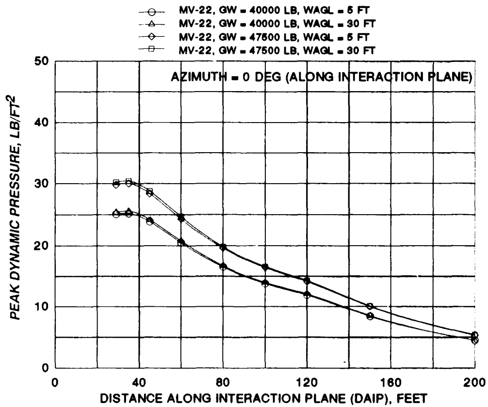
FIGURE 23 PEAK PROFILE VELOCITY AND DYNAMIC PRESSURE COMPARISONS FOR SEVERAL BELL/BOEING MV-22 CONFIGURATIONS ALONG THE 0 DEGREE AZIMUTH
