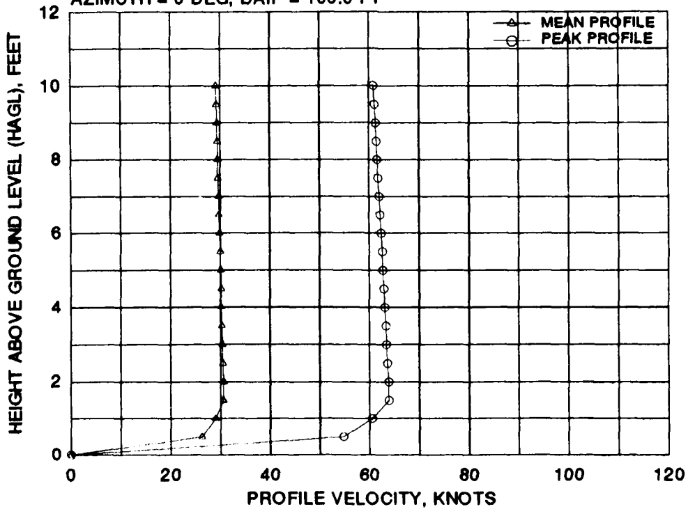
FIGURE B-6 BELL/BOEING MV-22 MEAN AND PEAK VELOCITY PROFILES FOR NINE 0 DEGREE AZIMUTH RADIAL STATIONS AT A WHEEL HEIGHT OF 5 FEET AND A GROSS WEIGHT OF 40,000 POUNDS (Continued)
