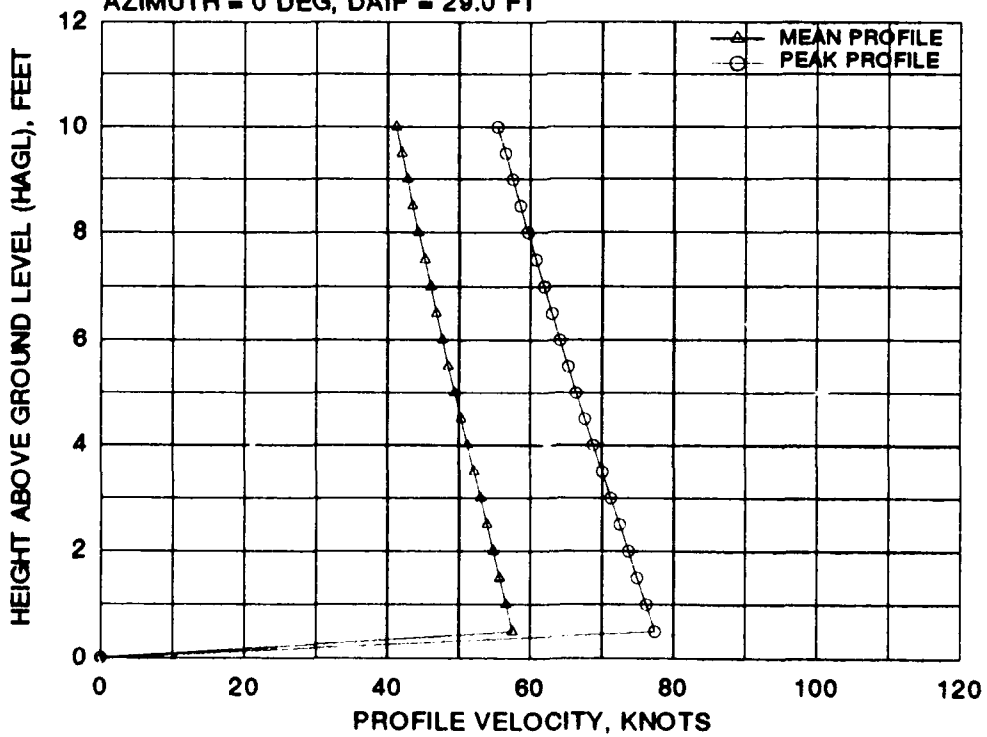
FIGURE D-3 CTR-800 MEAN AND PEAK VELOCITY PROFILES FOR EIGHT 0 DEGREE AZIMUTH RADIAL STATIONS AT A WHEEL HEIGHT OF 20 FEET AND A GROSS WEIGHT OF 15,750 POUNDS
