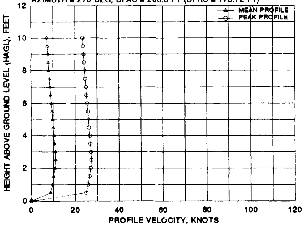
FIGURE B-3 BELL/BOEING MV-22 MEAN AND PEAK VELOCITY PROFILES FOR EIGHT 270 DEGREE AZIMUTH RADIAL STATIONS AT A WHEEL HEIGHT OF 30 FEET AND A GROSS WEIGHT OF 40,000 POUNDS (Concluded)
