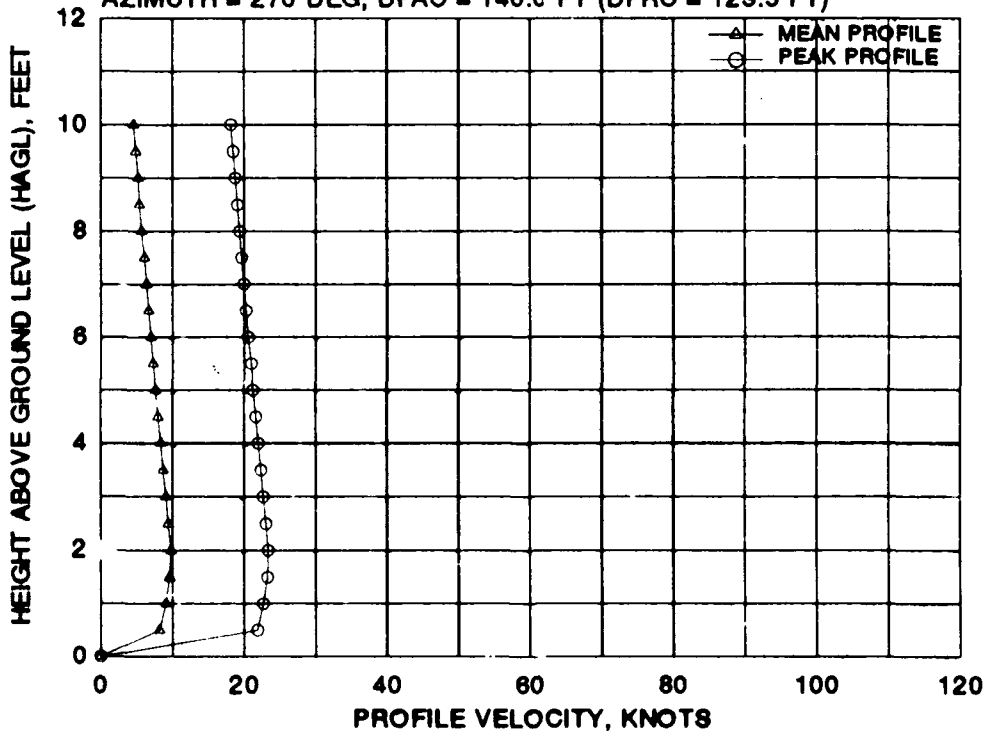
FIGURE D-2 CTR-800 MEAN AND PEAK VELOCITY PROFILES FOR EIGHT 270 DEGREE AZIMUTH RADIAL STATIONS AT A WHEEL HEIGHT OF 20 FEET AND A GROSS WEIGHT OF 15,750 POUNDS (Concluded)
