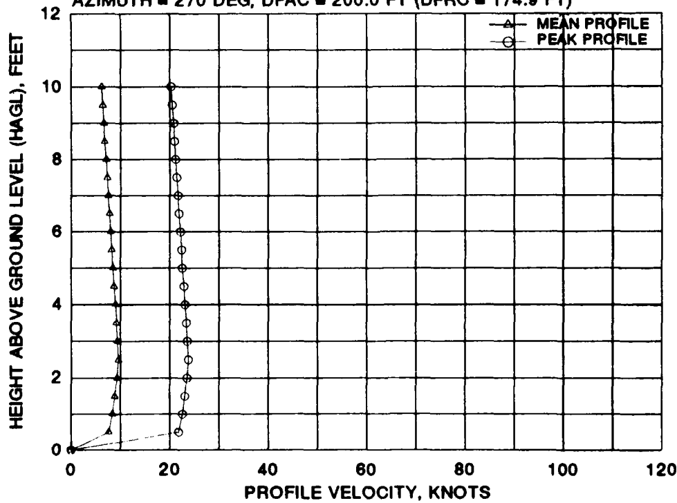
FIGURE H-2 EUROFAR TILTROTOR MEAN AND PEAK VELOCITY PROFILES FOR EIGHT 270 DEGREE AZIMUTH RADIAL STATIONS AT A WHEEL HEIGHT OF 30 FEET AND A GROSS WEIGHT OF 30,089 POUNDS (Concluded)
