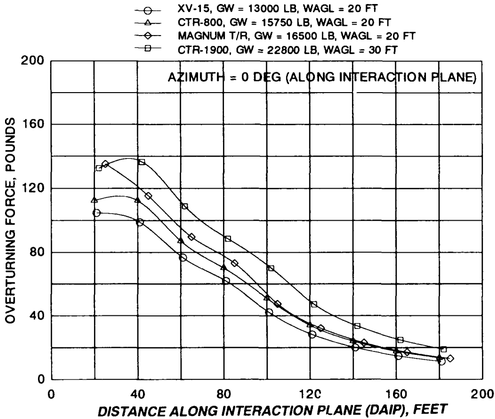
FIGURE 27 PERSONNEL OVERTURNING FORCES FOR SMALL TILTROTOR CONFIGURATIONS
