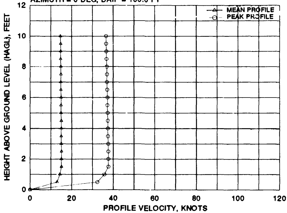
FIGURE J-3 ISHIDA TW-68 MEAN AND PEAK VELOCITY PROFILES FOR EIGHT 0 DEGREE AZIMUTH RADIAL STATIONS AT A WHEEL HEIGHT OF 15 FEET AND A GROSS WEIGHT OF 12,500 POUNDS (Concluded)
