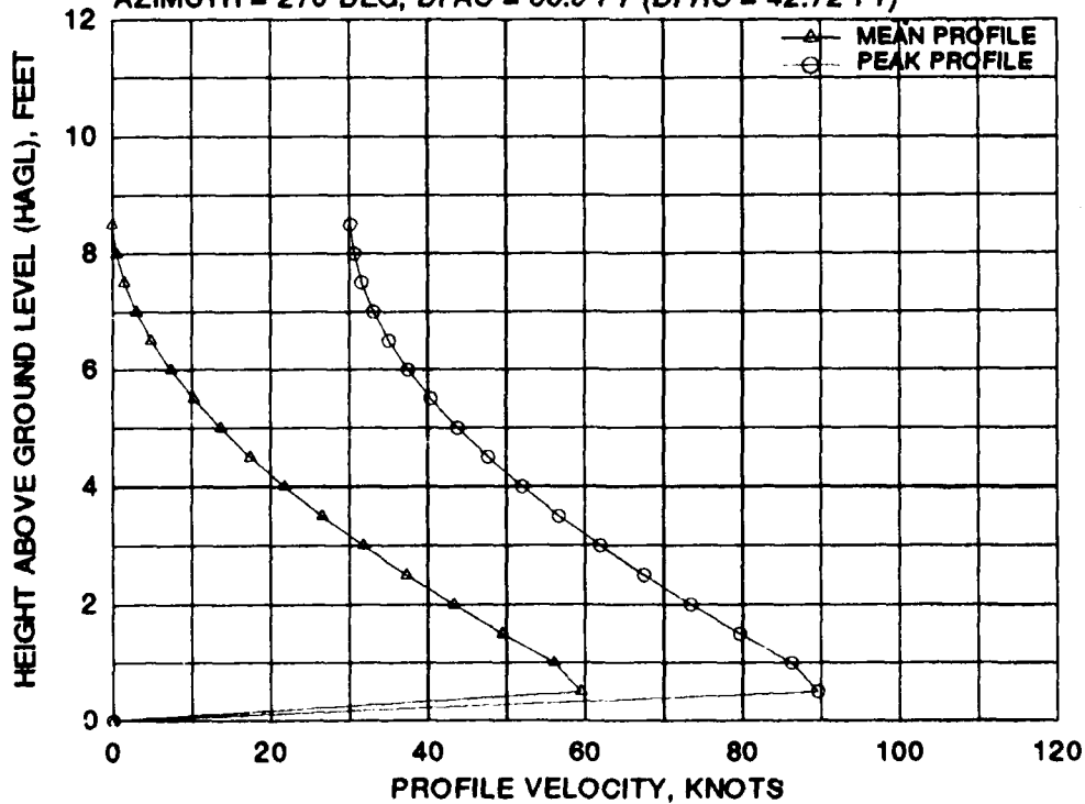
FIGURE B-5 BELL/BOEING MV-22 MEAN AND PEAK VELOCITY PROFILES FOR EIGHT 270 DEGREE AZIMUTH RADIAL STATIONS AT A WHEEL HEIGHT OF 30 FEET AND A GROSS WEIGHT OF 47,500 POUNDS
