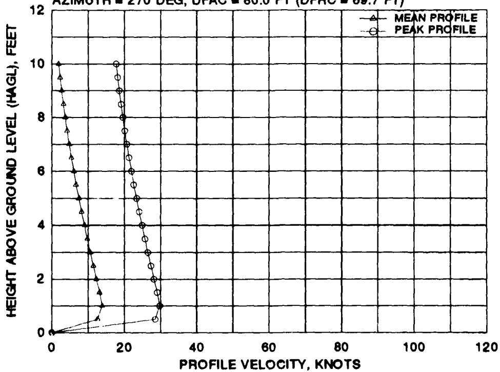
FIGURE I-2 CANADAIR CL-84 MEAN AND PEAK VELOCITY PROFILES FOR EIGHT 270 DEGREE AZIMUTH RADIAL STATIONS AT A WHEEL HEIGHT OF 15 FEET AND A GROSS WEIGHT OF 12,200 POUNDS (Continued)
