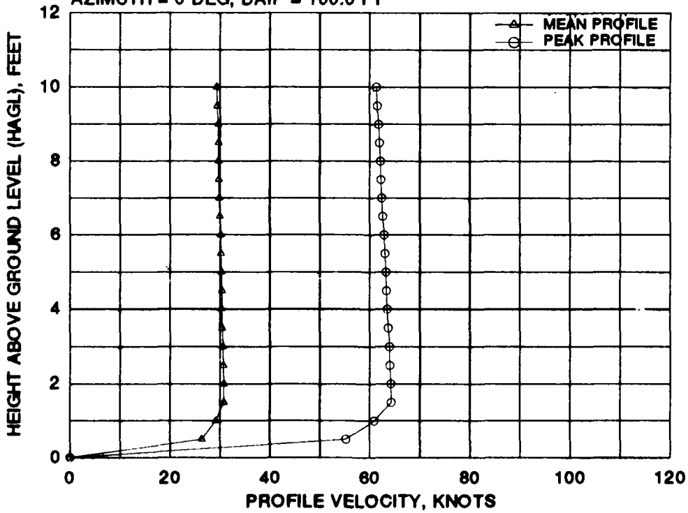
FIGURE B-7 BELL/BOEING MV-22 MEAN AND PEAK VELOCITY PROFILES FOR NINE 0 DEGREE AZIMUTH RADIAL STATIONS AT A WHEEL HEIGHT OF 30 FEET AND A GROSS WEIGHT OF 40,000 POUNDS (Continued)
