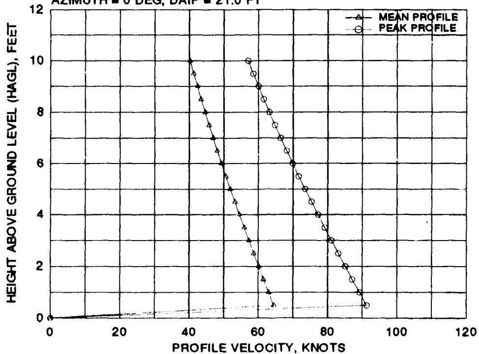
FIGURE J-3 ISHIDA TW-68 MEAN AND PEAK VELOCITY PROFILES FOR EIGHT 0 DEGREE AZIMUTH RADIAL STATIONS AT A WHEEL HEIGHT OF 15 FEET AND A GROSS WEIGHT OF 12,500 POUNDS
