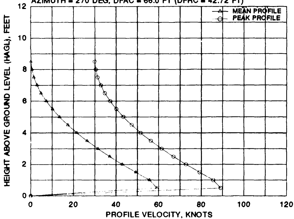
FIGURE B-4 BELL/BOEING MV-22 MEAN AND PEAK VELOCITY PROFILES FOR EIGHT 270 DEGREE AZIMUTH RADIAL STATIONS AT A WHEEL HEIGHT OF 5 FEET AND A GROSS WEIGHT OF 47,500 POUNDS
