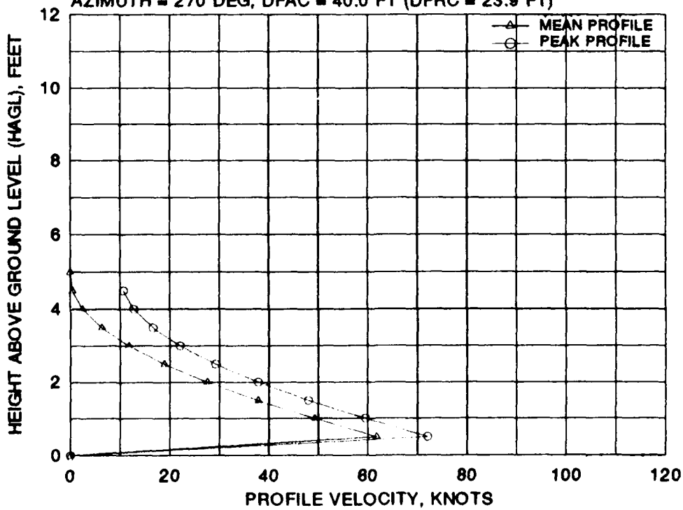
FIGURE G-2 MAGNUM TILTROTOR MEAN AND PEAK VELOCITY PROFILES FOR EIGHT 270 DEGREE AZIMUTH RADIAL STATIONS AT A WHEEL HEIGHT OF 20 FEET AND A GROSS WEIGHT OF 16,500 POUNDS
