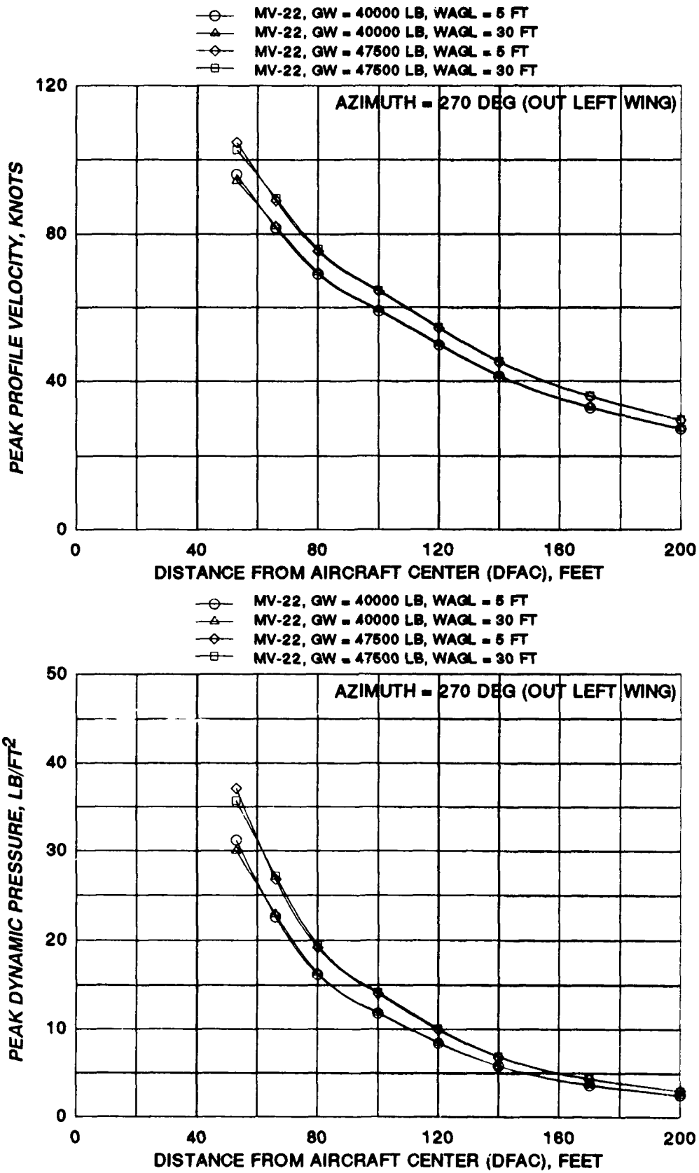
FIGURE 19 PEAK PROFILE VELOCITY AND DYNAMIC PRESSURE COMPARISONS FOR SEVERAL BELL/BOEING MV-22 CONFIGURATIONS ALONG THE 270 DEGREE AZIMUTH
