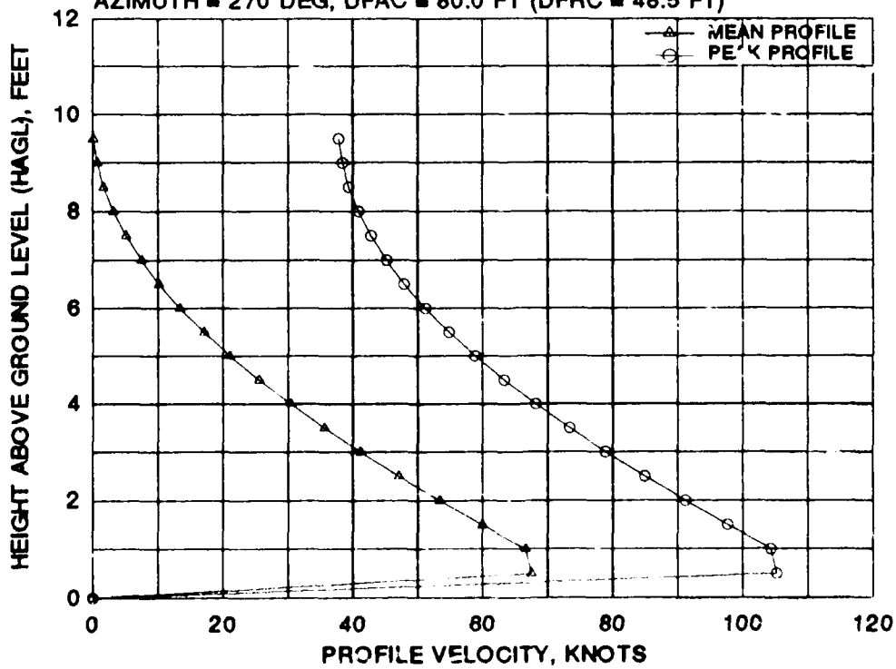
FIGURE F-2 CTR-7500 MEAN AND PEAK VELOCITY PROFILES FOR SEVEN 270 DEGREE AZIMUTH RADIAL STATIONS AT A WHEEL HEIGHT OF 30 FEET AND A GROSS WEIGHT OF 79,820 POUNDS
