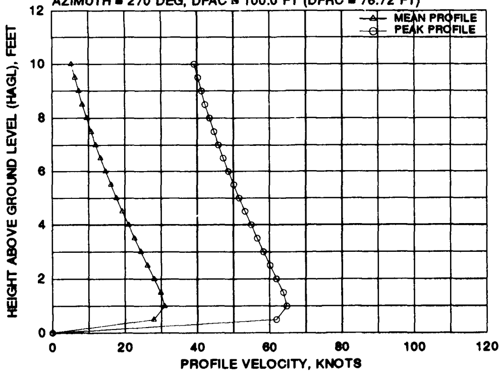
FIGURE B-5 BELL/BOEING MV-22 MEAN AND PEAK VELOCITY PROFILES FOR EIGHT 270 DEGREE AZIMUTH RADIAL STATIONS AT A WHEEL HEIGHT OF 30 FEET AND A GROSS WEIGHT OF 47,500 POUNDS (Continued)
