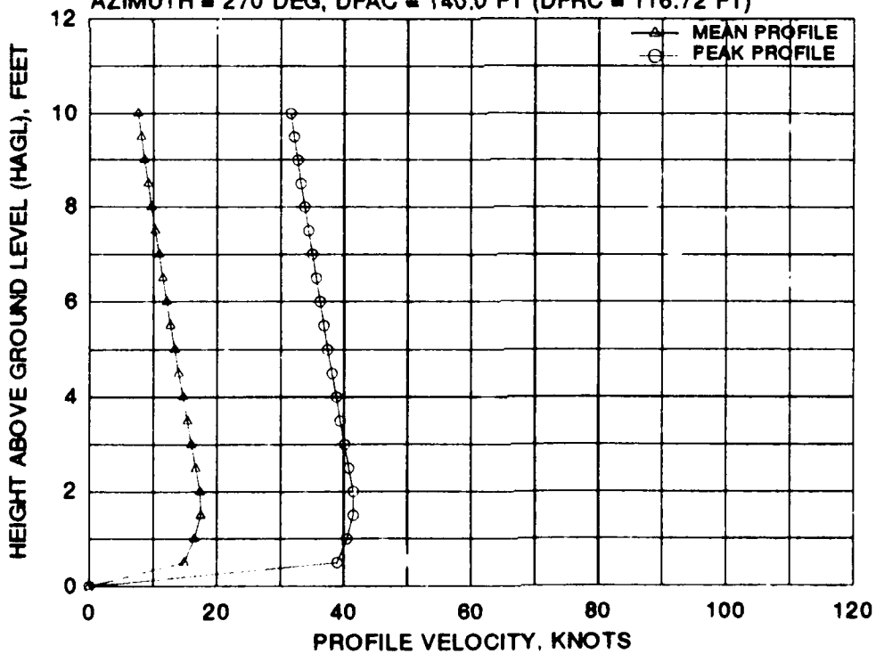
FIGURE B-3 BELL/BOEING MV-22 MEAN AND PEAK VELOCITY PROFILES FOR EIGHT 270 DEGREE AZIMUTH RADIAL STATIONS AT A WHEEL HEIGHT OF 30 FEET AND A GROSS WEIGHT OF 40,000 POUNDS (Continued)
