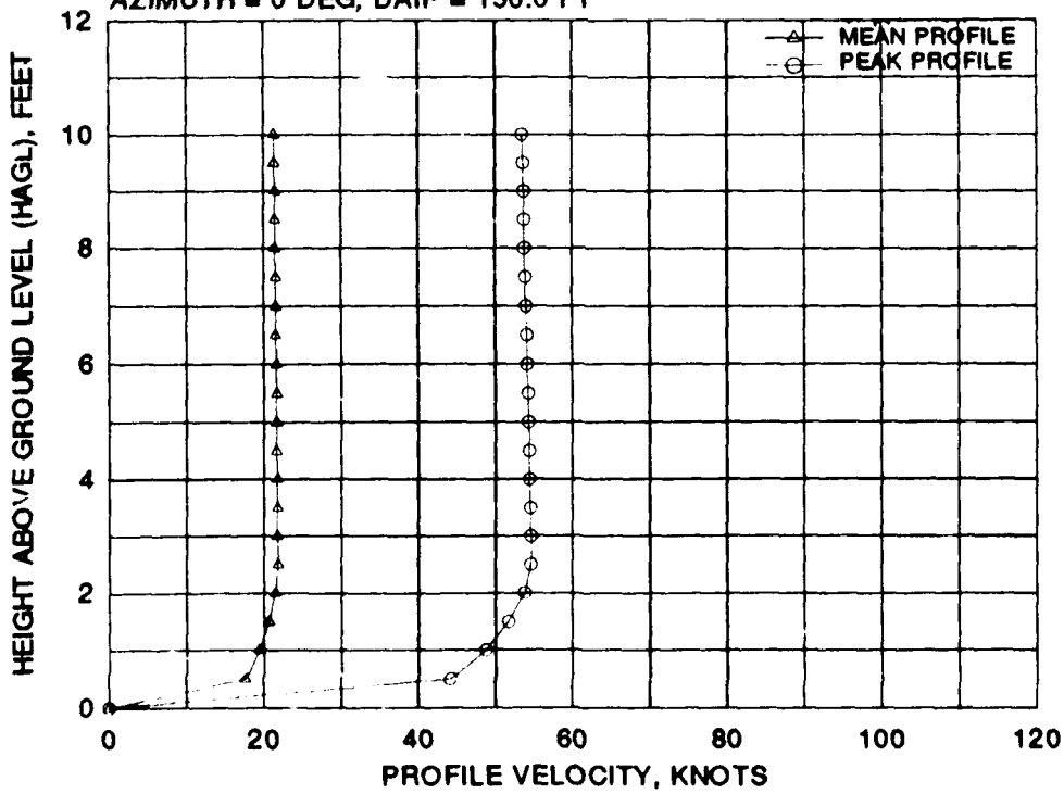
FIGURE B-9 BELL/BOEING MV-22 MEAN AND PEAK VELOCITY PROFILES FOR NINE 0 DEGREE AZIMUTH RADIAL STATIONS AT A WHEEL HEIGHT OF 30 FEET AND A GROSS WEIGHT OF 47,500 POUNDS (Continued)
