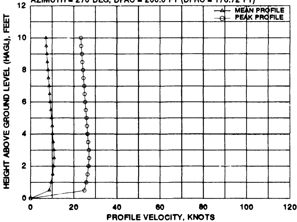
FIGURE B-2 BELL/BOEING MV-22 MEAN AND PEAK VELOCITY PROFILES FOR EIGHT 270 DEGREE AZIMUTH RADIAL STATIONS AT A WHEEL HEIGHT OF 5 FEET AND A GROSS WEIGHT OF 40,000 POUNDS (Concluded)
