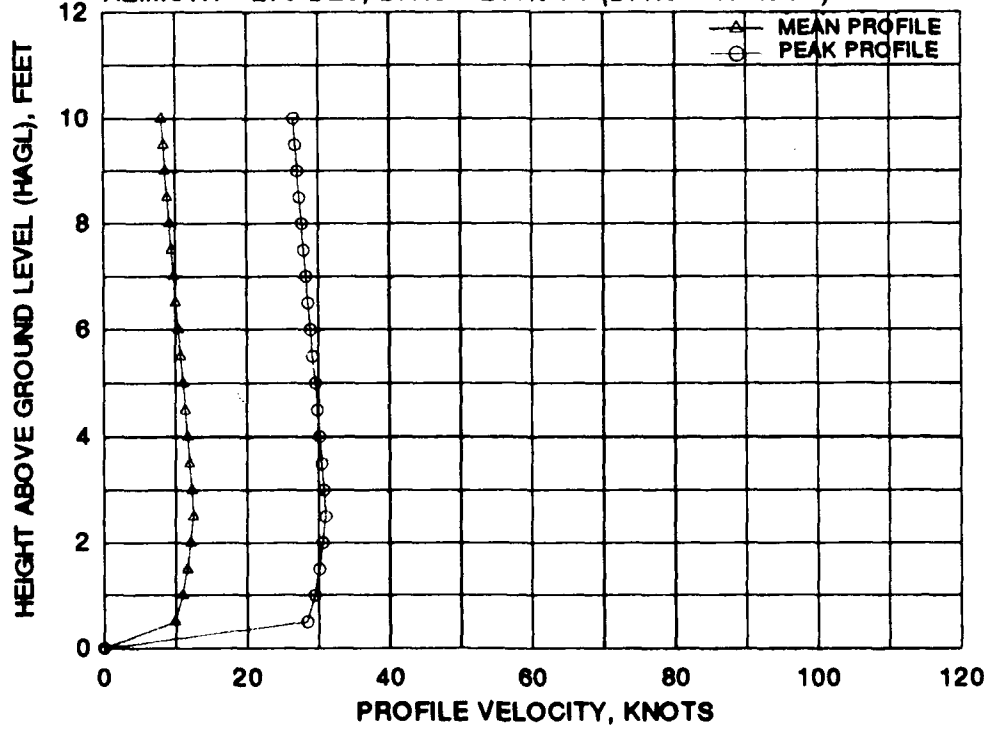
FIGURE C-2 CTR-22C/D MEAN AND PEAK VELOCITY PROFILES FOR EIGHT 270 DEGREE AZIMUTH RADIAL STATIONS AT A WHEEL HEIGHT OF 30 FEET AND A GROSS WEIGHT OF 51,670 POUNDS (Concluded)
