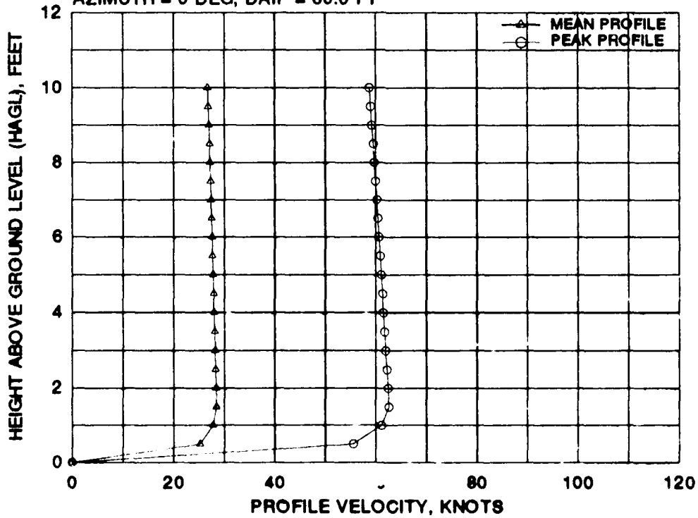
FIGURE E-3 CTR-1900 MEAN AND PEAK VELOCITY PROFILES FOR NINE 0 DEGREE AZIMUTH RADIAL STATIONS AT A WHEEL HEIGHT OF 30 FEET AND GROSS WEIGHT OF 22,800 POUNDS (Continued)
