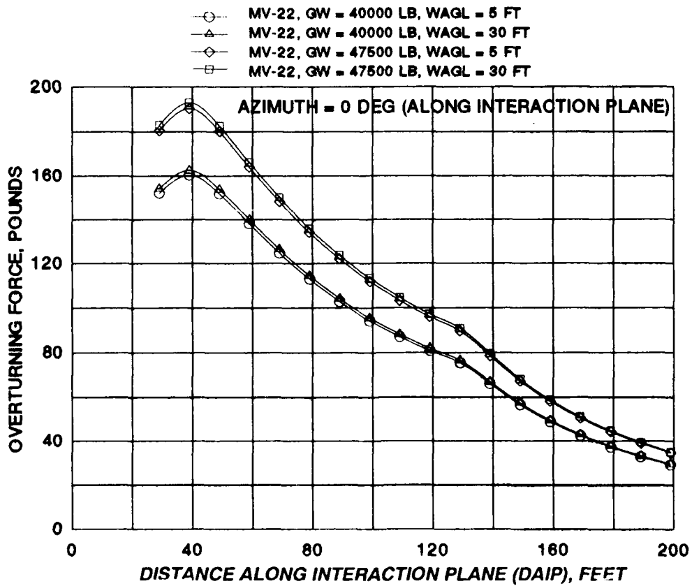
FIGURE 28 PERSONNEL OVERTURNING FORCES FOR VARIOUS MV-22 TILTROTOR CONFIGURATIONS
