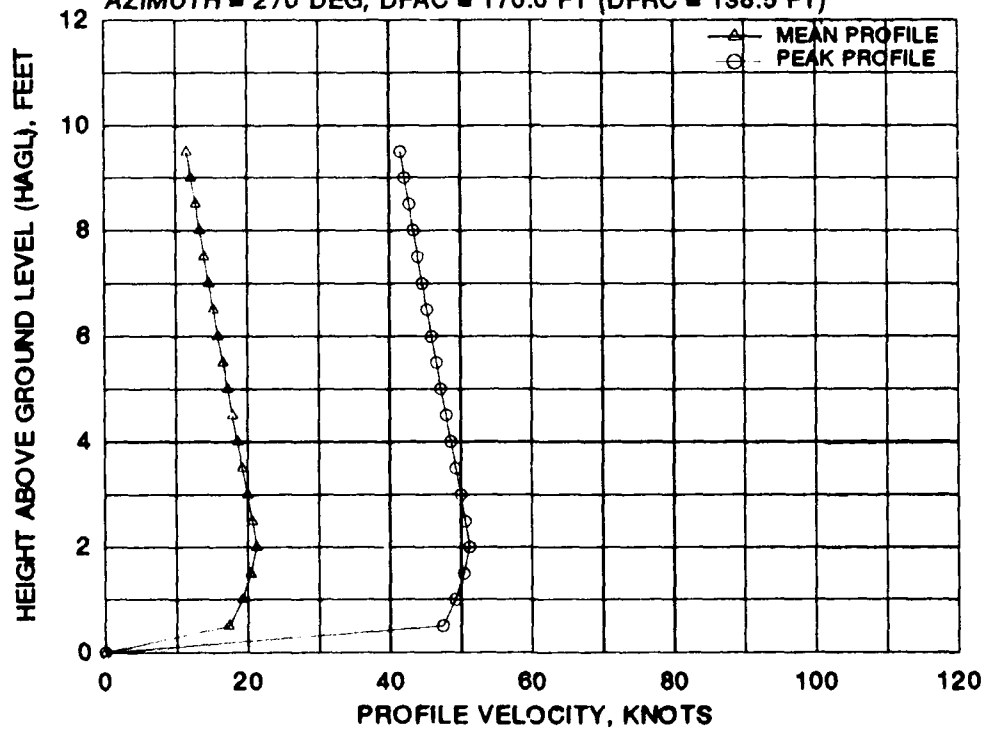
FIGURE F-2 CTR-7500 MEAN AND PEAK VELOCITY PROFILES FOR SEVEN 270 DEGREE AZIMUTH RADIAL STATIONS AT A WHEEL HEIGHT OF 30 FEET AND A GROSS WEIGHT OF 79,820 POUNDS (Continued)
