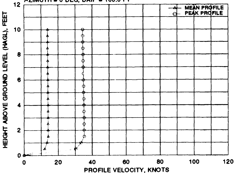
FIGURE I-3 CANADAIR CL-84 MEAN AND PEAK VELOCITY PROFILES FOR EIGHT 0 DEGREE AZIMUTH RADIAL STATIONS AT A WHEEL HEIGHT OF 15 FEET AND A GROSS WEIGHT OF 12,200 POUNDS (Concluded)
