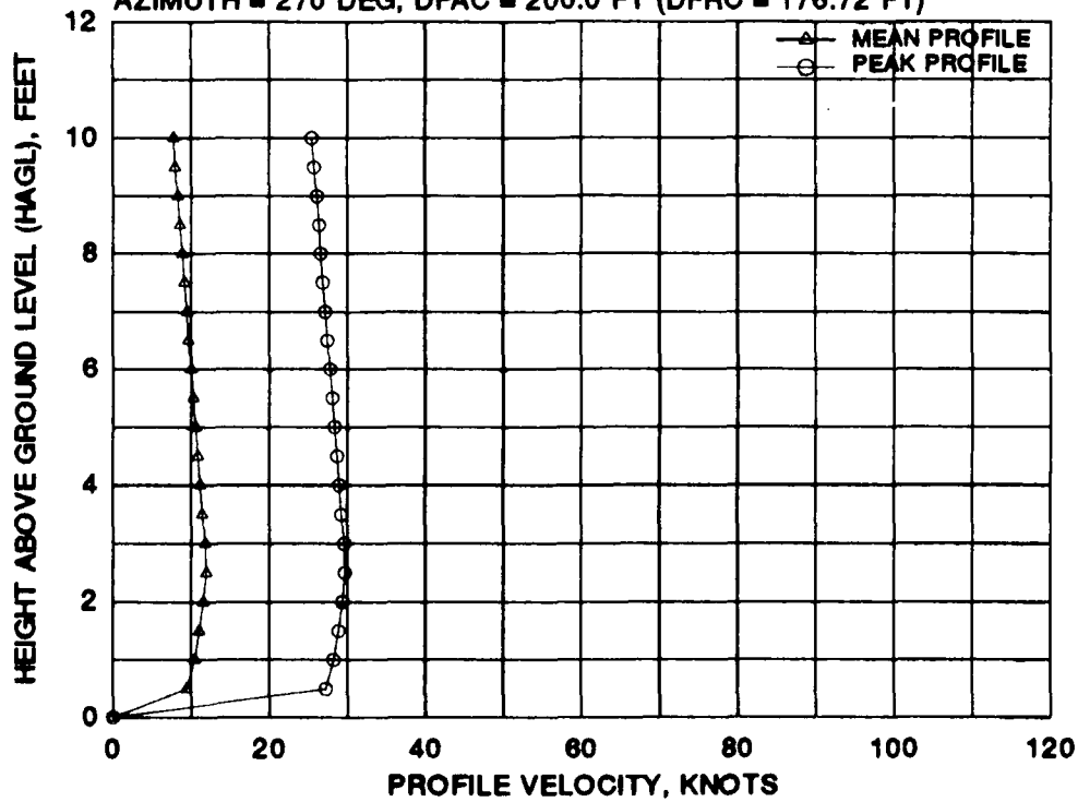
FIGURE B-5 BELL/BOEING MV-22 MEAN AND PEAK VELOCITY PROFILES FOR EIGHT 270 DEGREE AZIMUTH RADIAL STATIONS AT A WHEEL HEIGHT OF 30 FEET AND A GROSS WEIGHT OF 47,500 POUNDS (Concluded)
