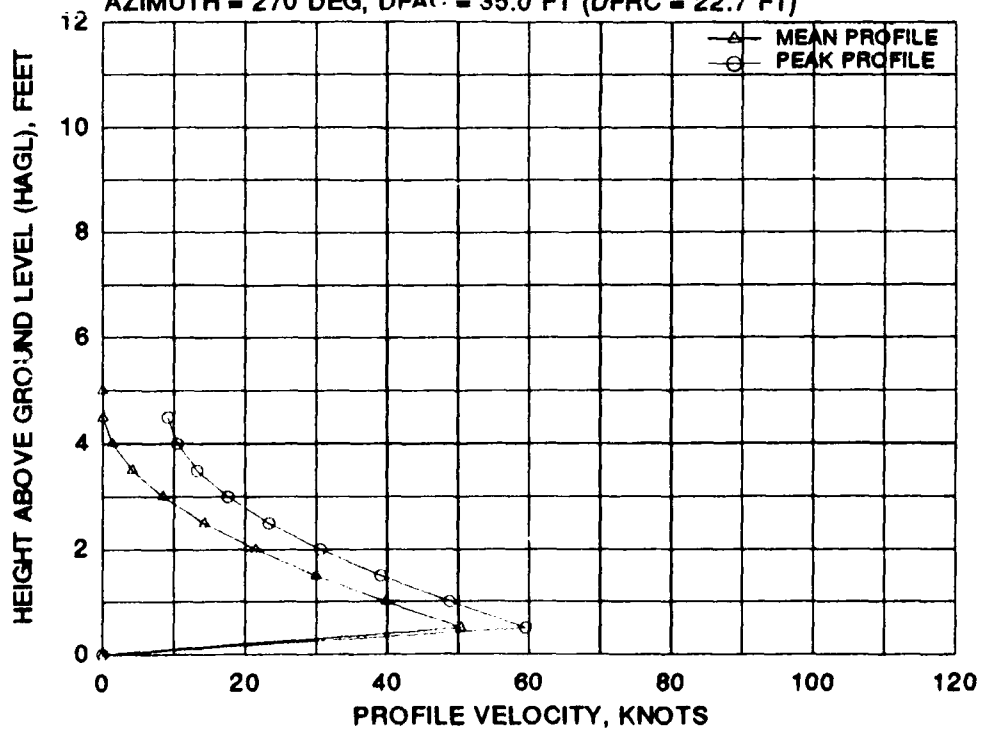
FIGURE J-2 ISHIDA TW-68 MEAN AND PEAK VELOCITY PROFILES FOR EIGHT 270 DEGREE AZIMUTH RADIAL STATIONS AT A WHEEL HEIGHT OF 15 FEET AND A GROSS WEIGHT OF 12,500 POUNDS
