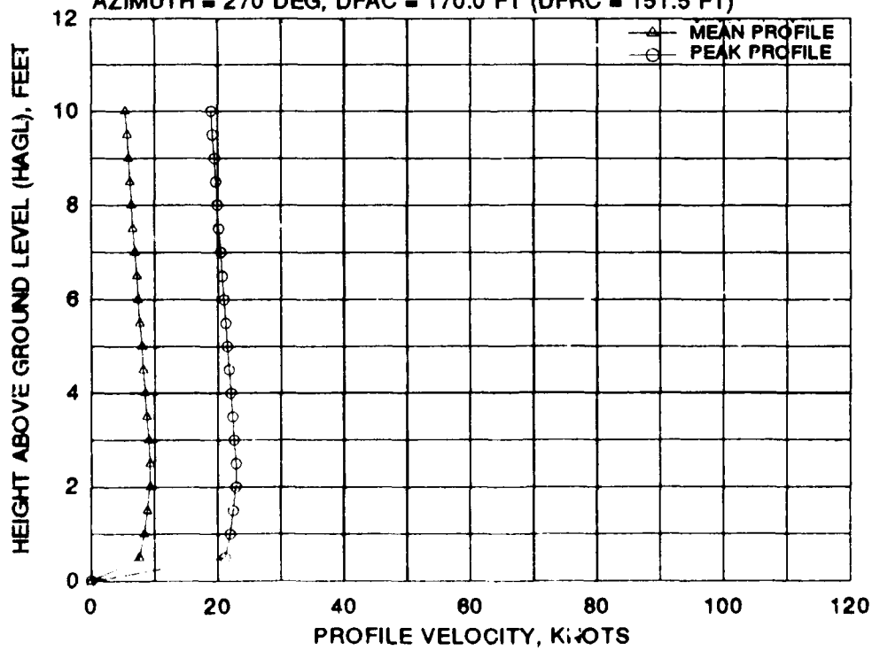
FIGURE E-2 CTR-1900 MEAN AND PEAK VELOCITY PROFILES FOR EIGHT 270 DEGREE AZIMUTH RADIAL STATIONS AT A WHEEL HEIGHT OF 30 FEET AND A GROSS WEIGHT OF 22,800 POUNDS (Concluded)
