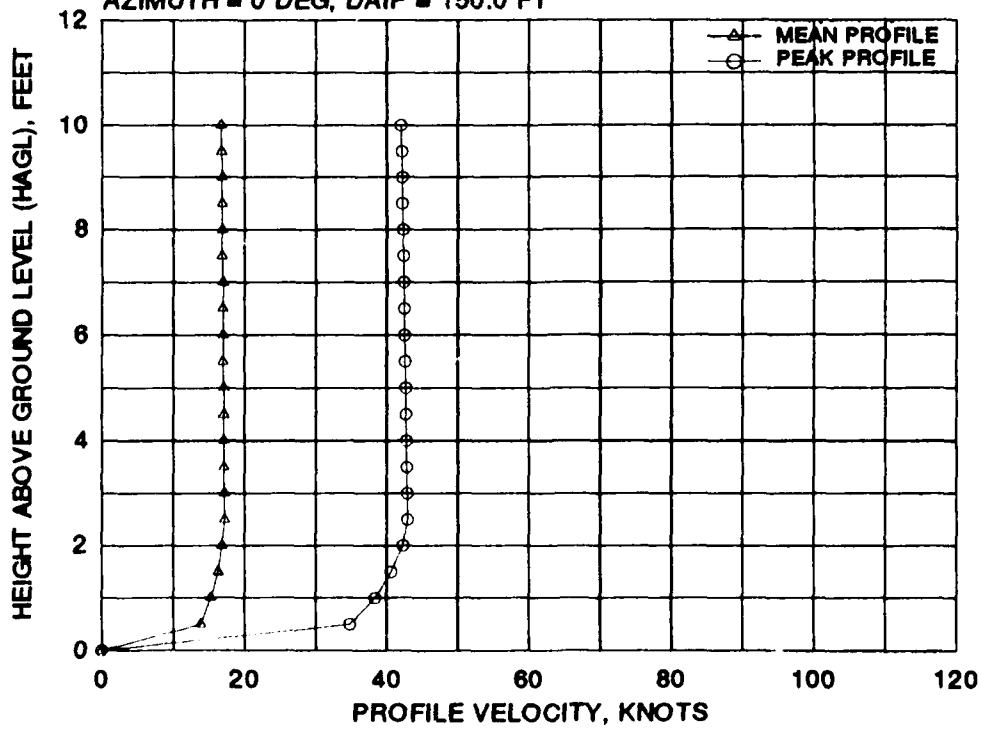
FIGURE H-3 EUROFAR TILTROTOR MEAN AND PEAK VELOCITY PROFILES FOR NINE 0 DEGREE AZIMUTH RADIAL STATIONS AT A WHEEL HEIGHT OF 30 FEET AND A GROSS WEIGHT OF 30,089 POUNDS (Continued)
