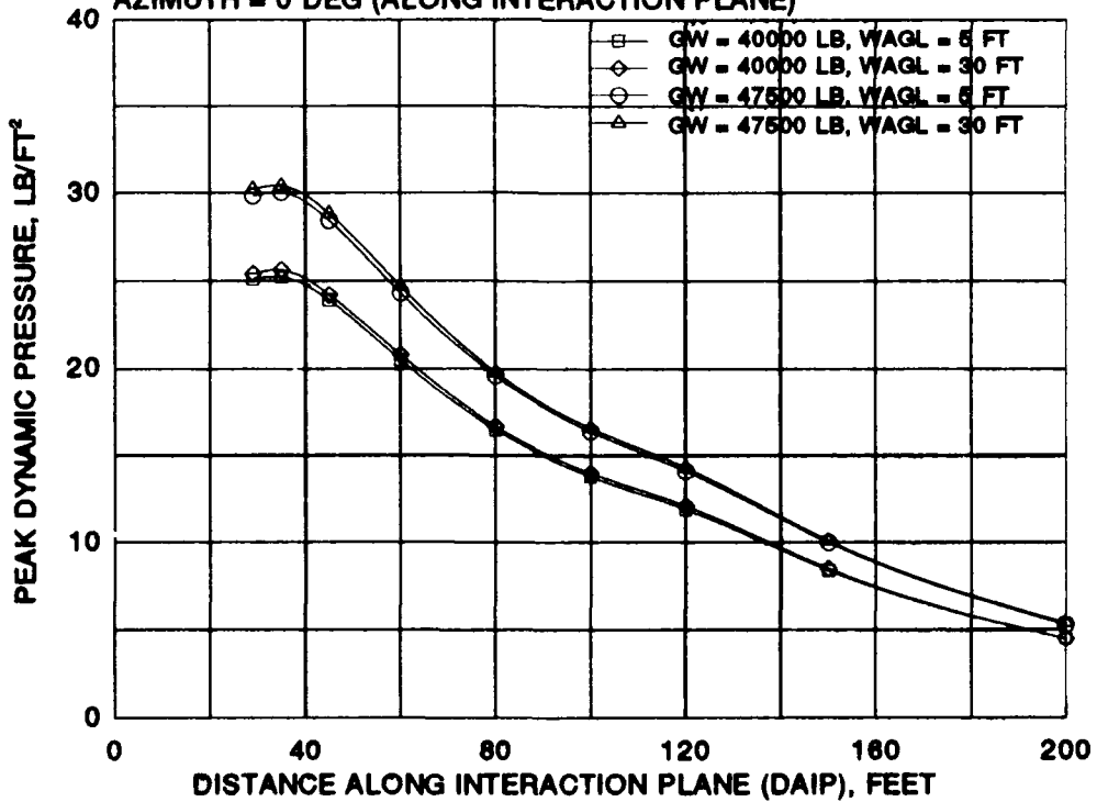
FIGURE B-11 BELL/BOEING MV-22 PEAK ROTORWASH VELOCITY AND DYNAMIC PRESSURE AS A FUNCTION OF DISTANCE ALONG THE INTERACTION PLANE (0 DEGREE AZIMUTH)
