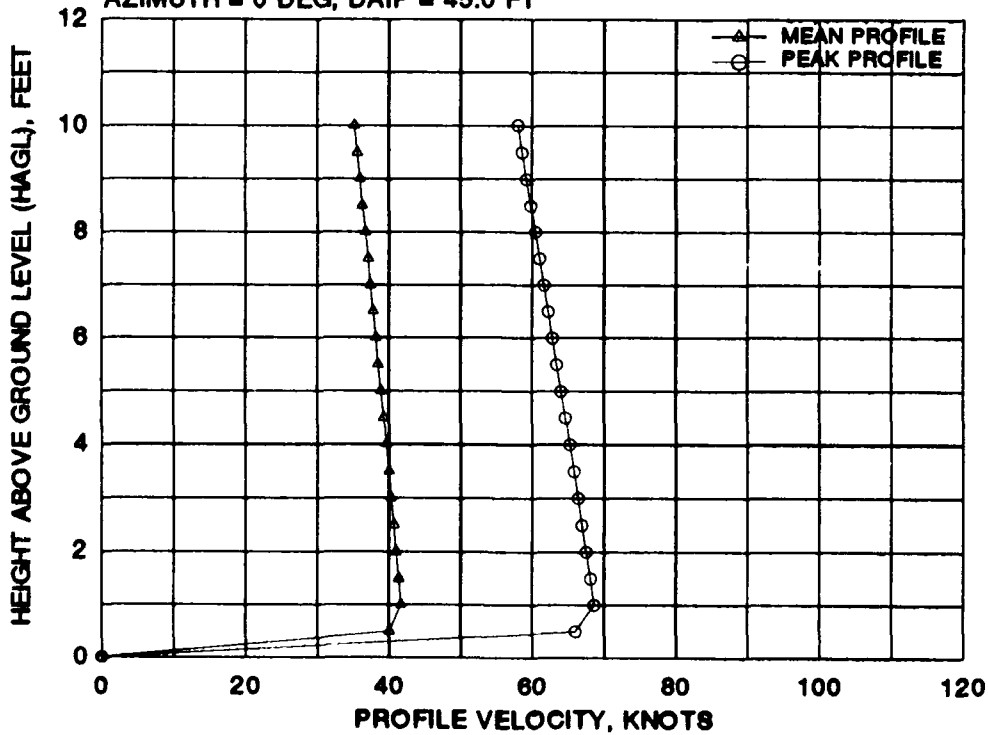
FIGURE D-3 CTR-800 MEAN AND PEAK VELOCITY PROFILES FOR EIGHT 0 DEGREE AZIMUTH RADIAL STATIONS AT A WHEEL HEIGHT OF 20 FEET AND A GROSS WEIGHT OF 15,750 POUNDS (Continued)
