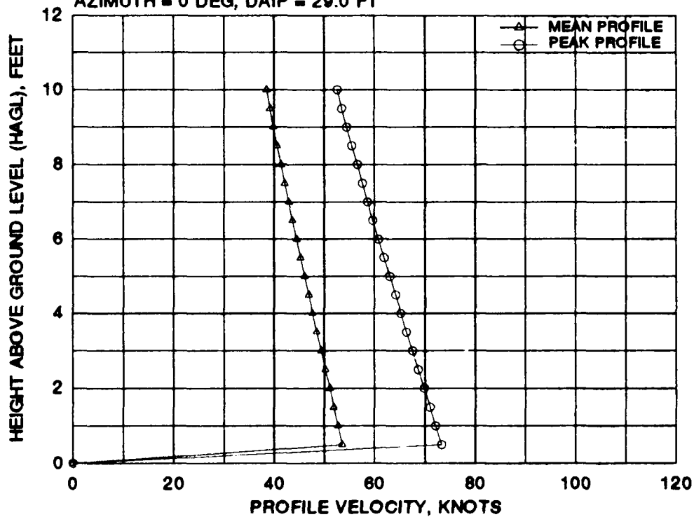
FIGURE A-3 BELL XV-15 MEAN AND PEAK VELOCITY PROFILES FOR EIGHT 0 DEGREE AZIMUTH RADIAL STATIONS AT A WHEEL HEIGHT OF 20 FEET AND A GROSS WEIGHT OF 13,000 POUNDS
