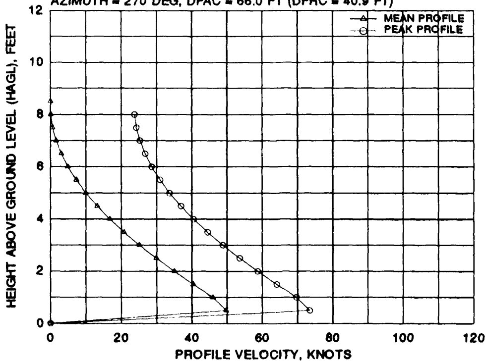
FIGURE H-2 EUROFAR TILTROTOR MEAN AND PEAK VELOCITY PROFILES FOR EIGHT 270 DEGREE AZIMUTH RADIAL STATIONS AT A WHEEL HEIGHT OF 30 FEET AND A GROSS WEIGHT OF 30,089 POUNDS
