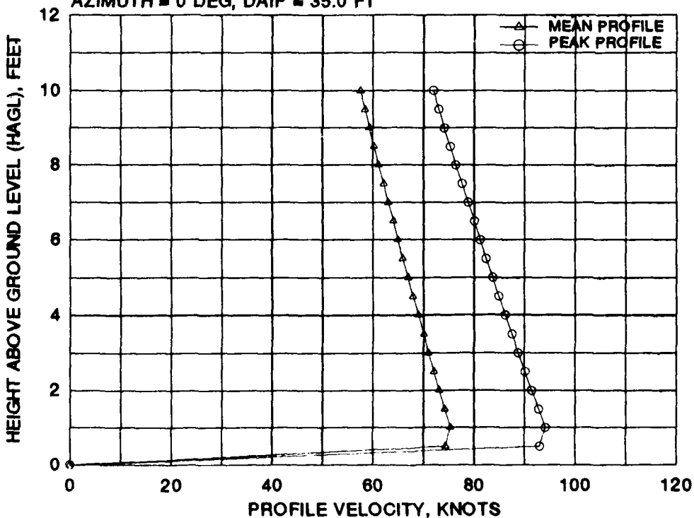
FIGURE B-8 BELL/BOEING MV-22 MEAN AND PEAK VELOCITY PROFILES FOR NINE 0 DEGREE AZIMUTH RADIAL STATIONS AT A WHEEL HEIGHT OF 5 FEET AND A GROSS WEIGHT OF 47,500 POUNDS
