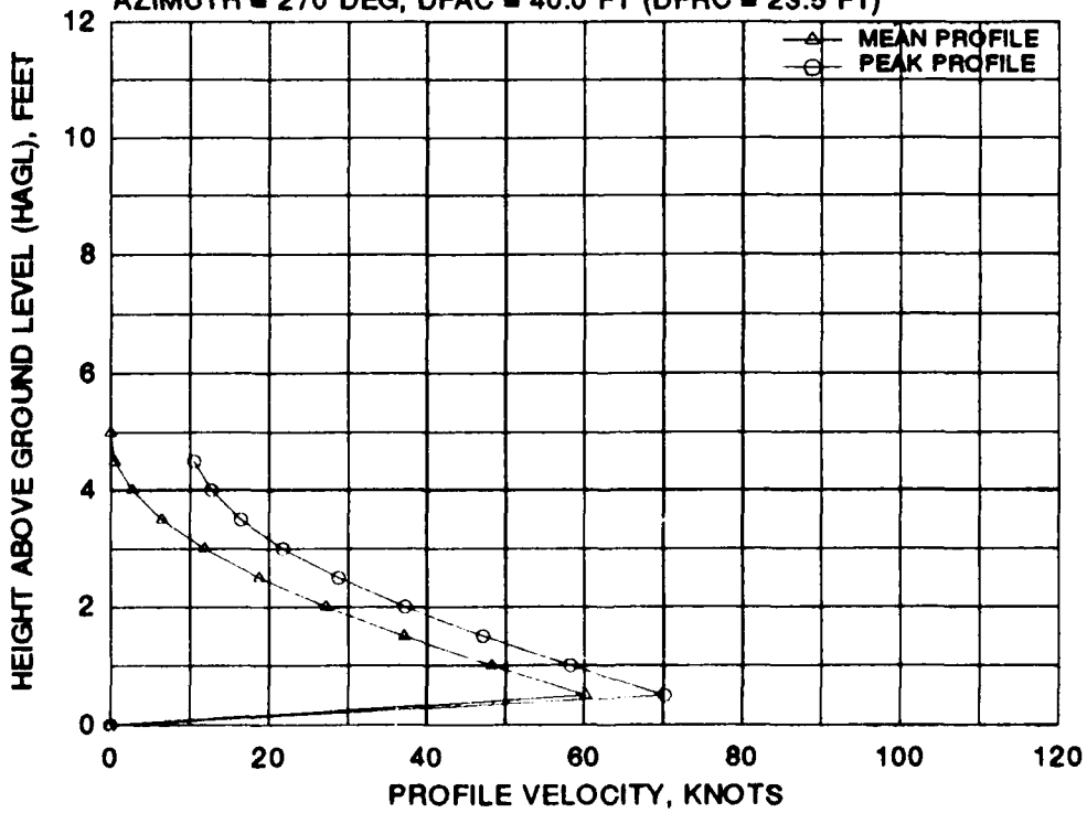
FIGURE D-2 CTR-800 MEAN AND PEAK VELOCITY PROFILES FOR EIGHT 270 DEGREE AZIMUTH RADIAL STATIONS AT A WHEEL HEIGHT OF 20 FEET AND A GROSS WEIGHT OF 15,750 POUNDS
