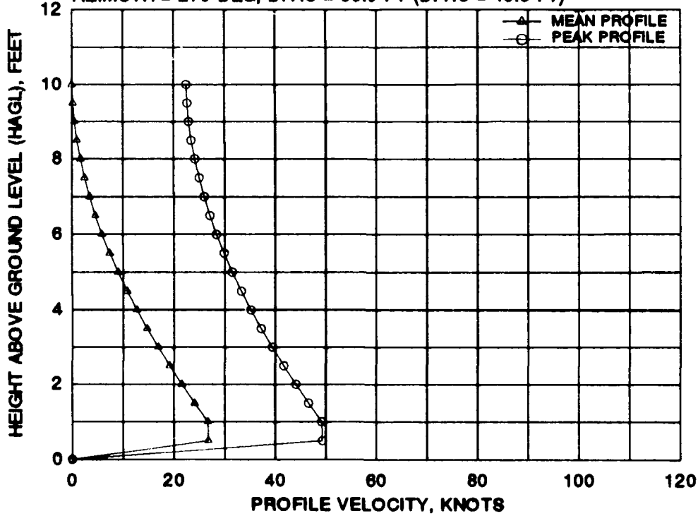
FIGURE D-2 CTR-800 MEAN AND PEAK VELOCITY PROFILES FOR EIGHT 270 DEGREE AZIMUTH RADIAL STATIONS AT A WHEEL HEIGHT OF 20 FEET AND A GROSS WEIGHT OF 15,750 POUNDS (Continued)
