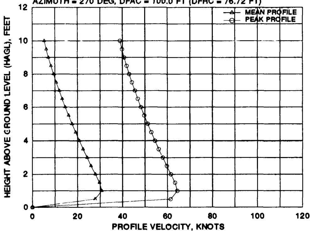
FIGURE B-4 BELL/BOEING MV-22 MEAN AND PEAK VELOCITY PROFILES FOR EIGHT 270 DEGREE AZIMUTH RADIAL STATIONS AT A WHEEL HEIGHT OF 5 FEET AND A GROSS WEIGHT OF 47,500 POUNDS (Continued)
