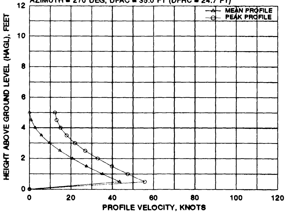
FIGURE I-2 CANADAIR CL-84 MEAN AND PEAK VELOCITY PROFILES FOR EIGHT 270 DEGREE AZIMUTH RADIAL STATIONS AT A WHEEL HEIGHT OF 15 FEET AND A GROSS WEIGHT OF 12,200 POUNDS
