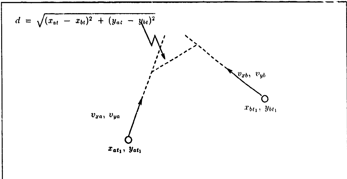
Figure 4.5. Illustration of Calculation
